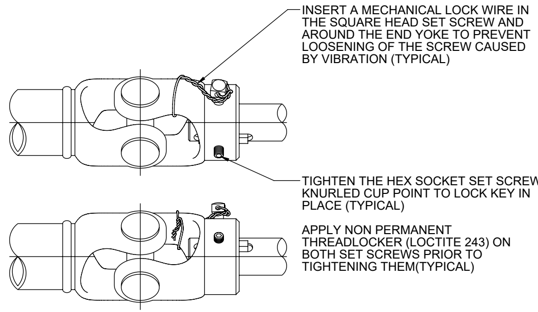
SHAFT LOCK WIRE INSTALLATION SCALE N.T.S.
