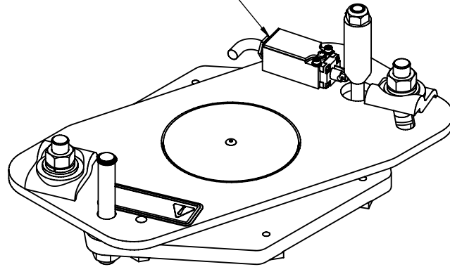
TOP PLATE SWITCH FOR ND9 REF. S10-023-011 NOT TO SCALE
