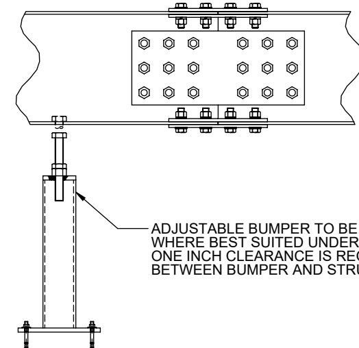
BUMPER INSTALLATION SCALE N.T.S.
