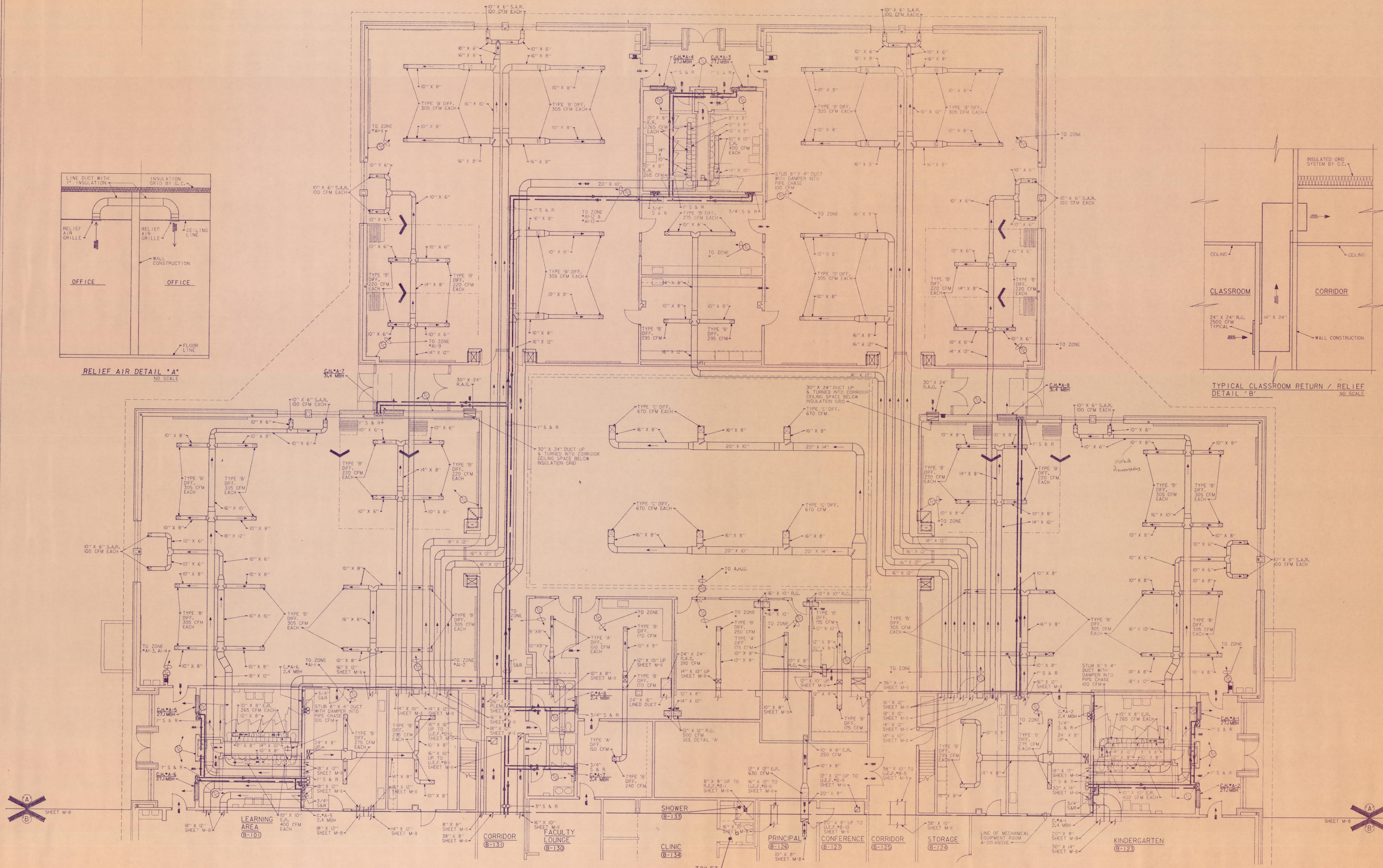
UNIT 'A' HEATING, VENTILATING, AIR-CONDITIONING FIRST FLOOR PLAN SCALE: 1/8" = 1'-0"
