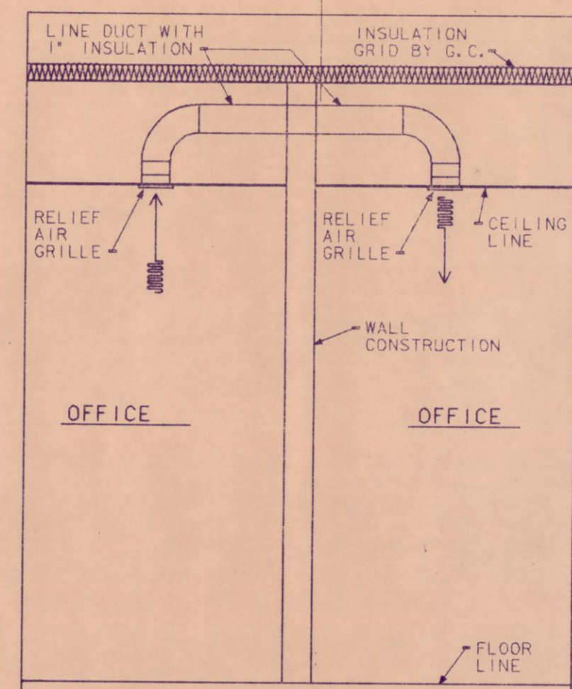
RELIEF AIR DETAIL "A" NO SCALE
