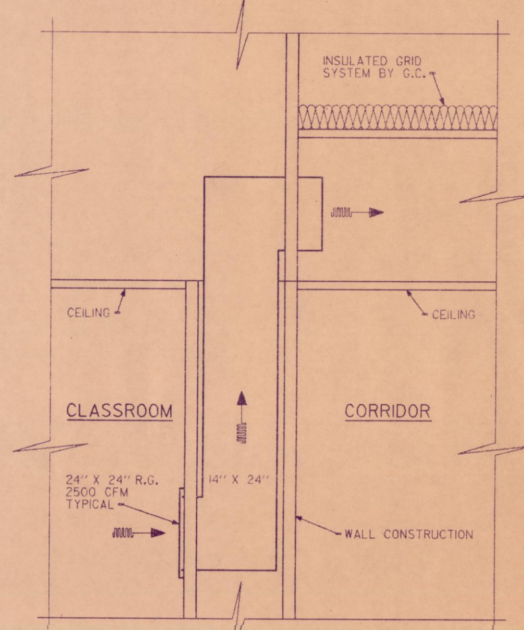
TYPICAL CLASSROOM RETURN / RELIEF DETAIL "B" NO SCALE
