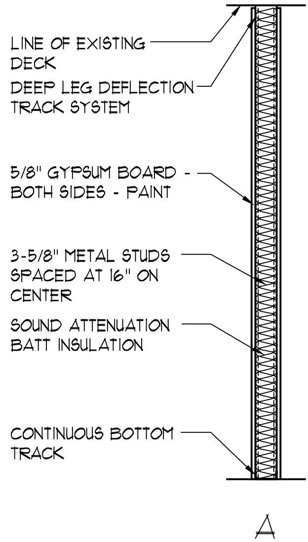
WALL TYPES NOT TO SCALE
