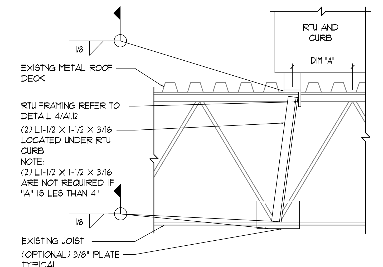
5 TYPICAL JOIST REINFORCEMENT UNDER RTU CURB 1 1/2" = 1'-0"
