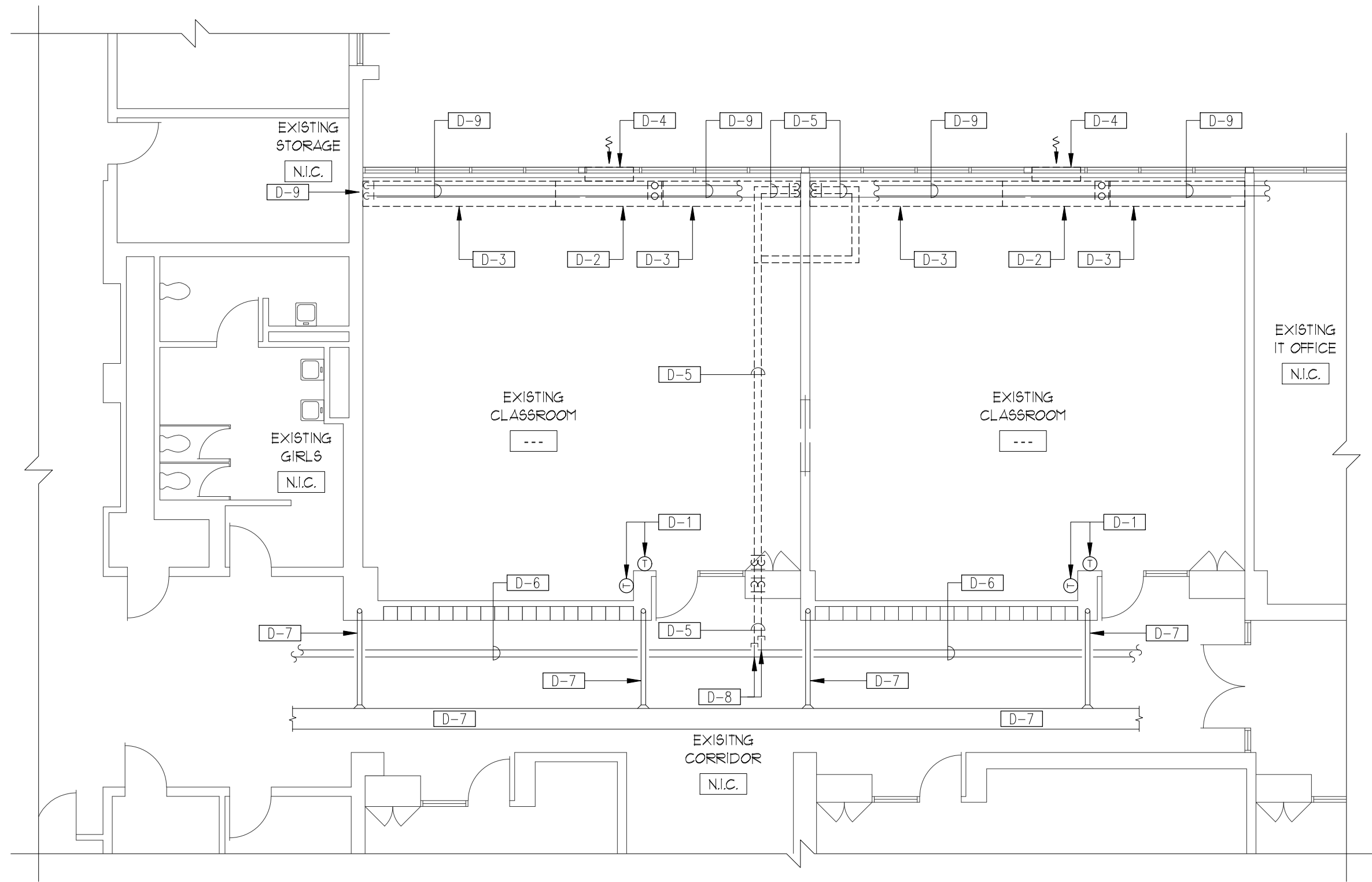
1 EXISTING PARTIAL FLOOR PLAN - MECHANICAL 1/8" = 1'-0"
