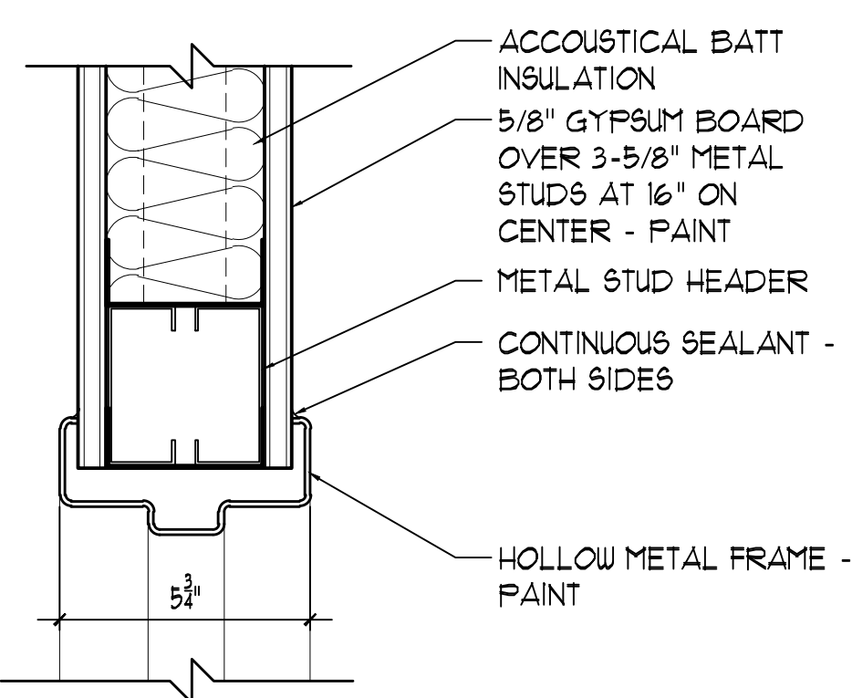
1 HEAD DETAIL 3" = 1'-0"
