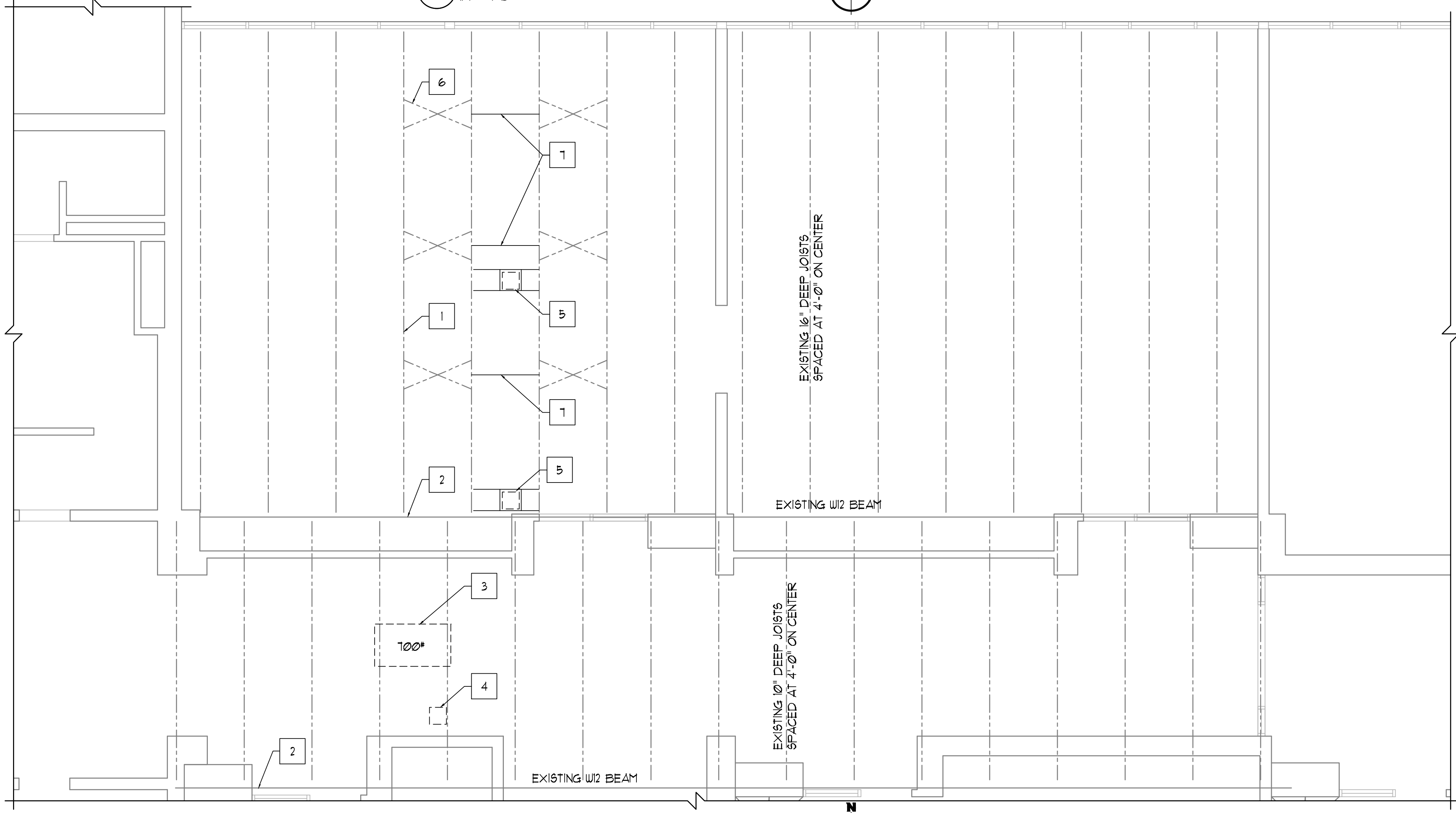
2 PARTIAL ROOF FRAMING PLAN 1/4" = 1'-0"
