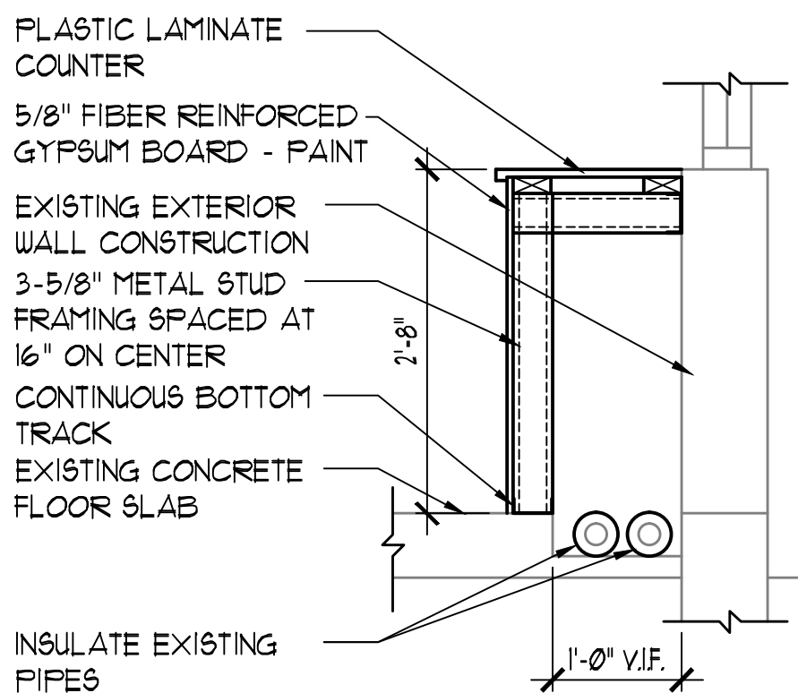
5 DETAIL 3" = 1'-0"
