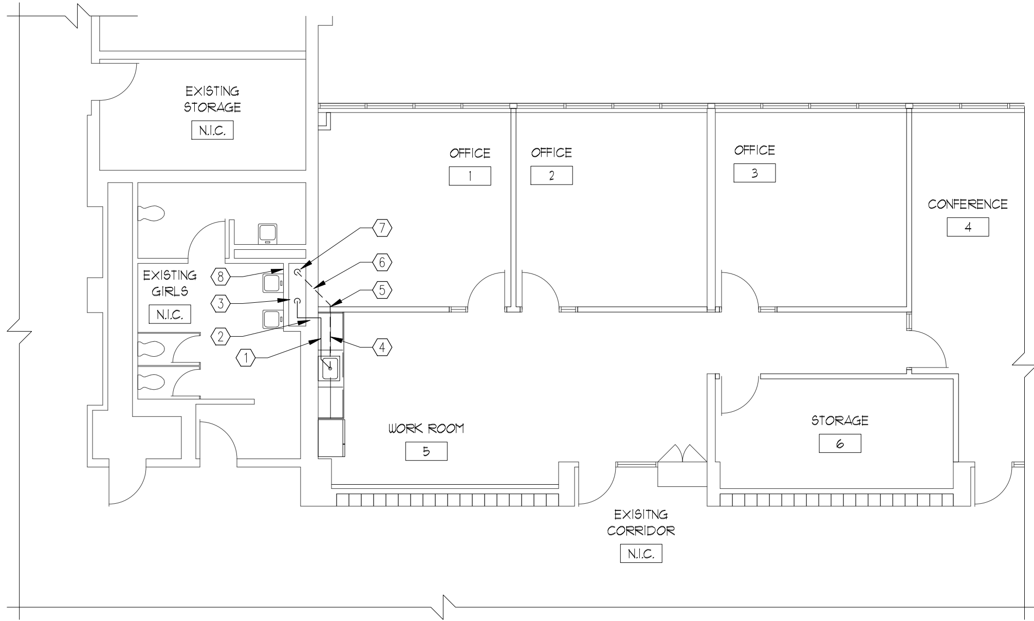
1 PARTIAL FLOOR PLAN - PLUMBING - SANITARY 1/8" = 1'-0"
