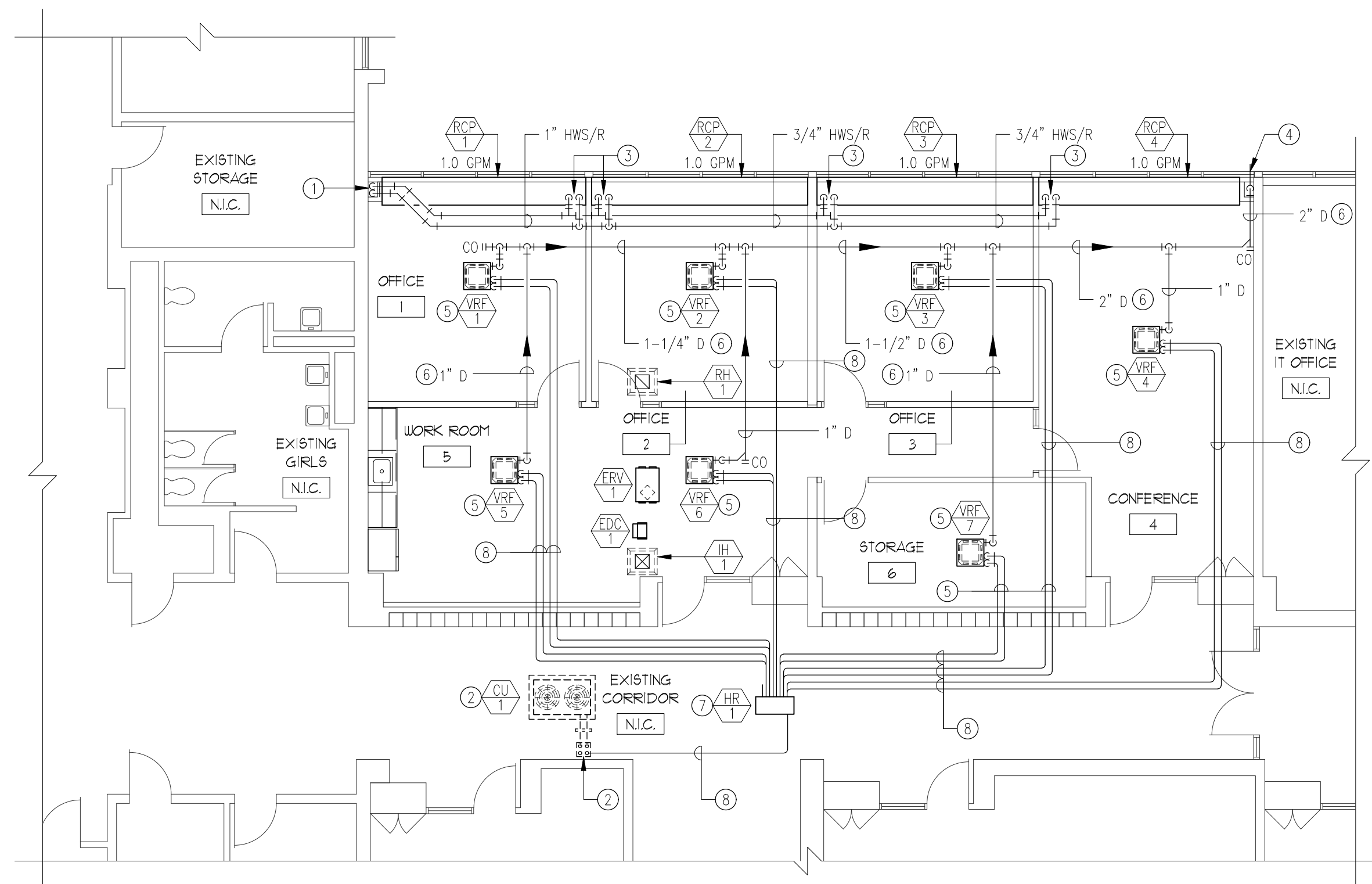
2 PARTIAL FLOOR PLAN - PIPING 1/8" = 1'-0"
