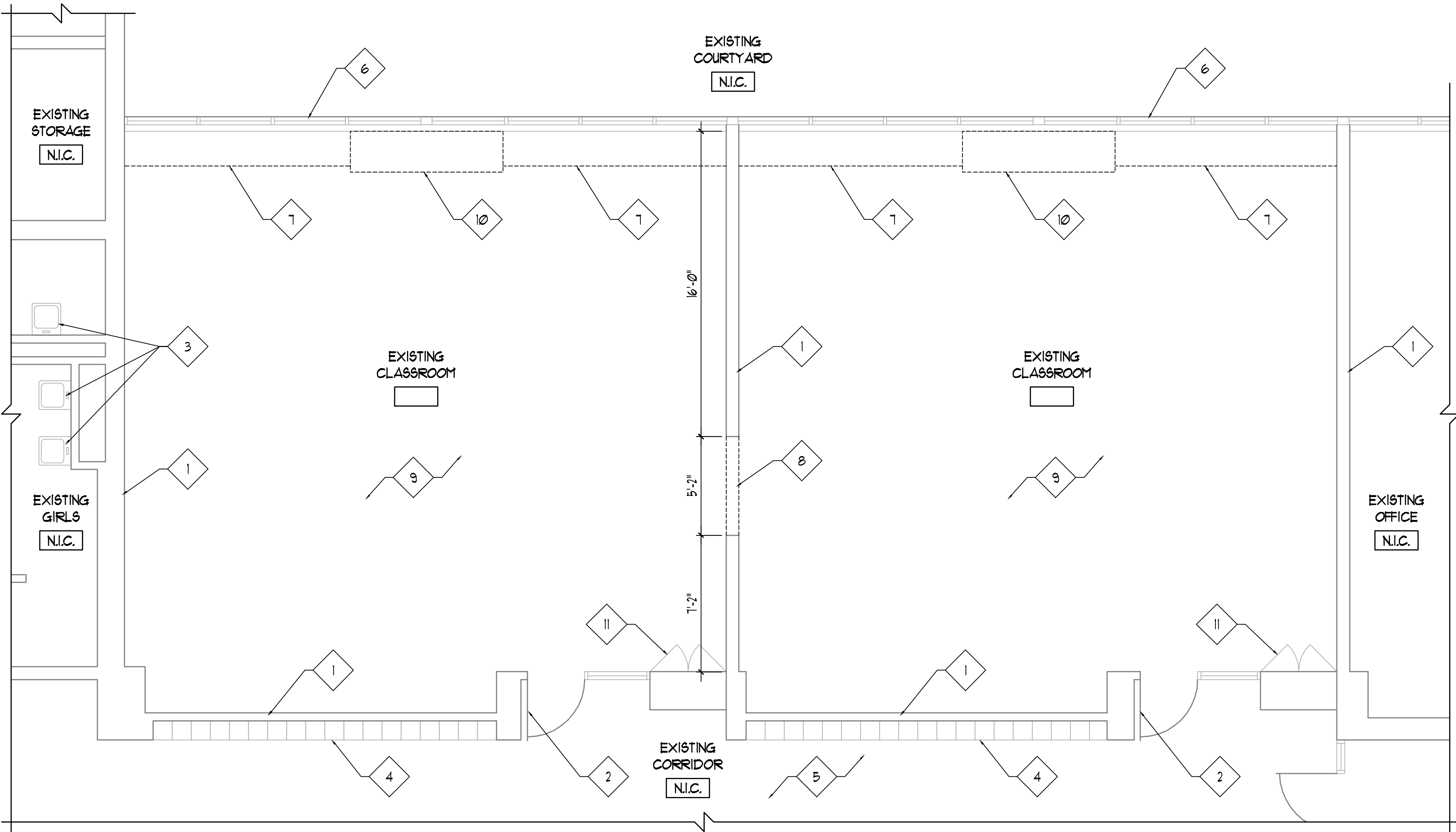
1 PARTIAL EXISTING FLOOR PLAN 1/4" = 1'-0"
