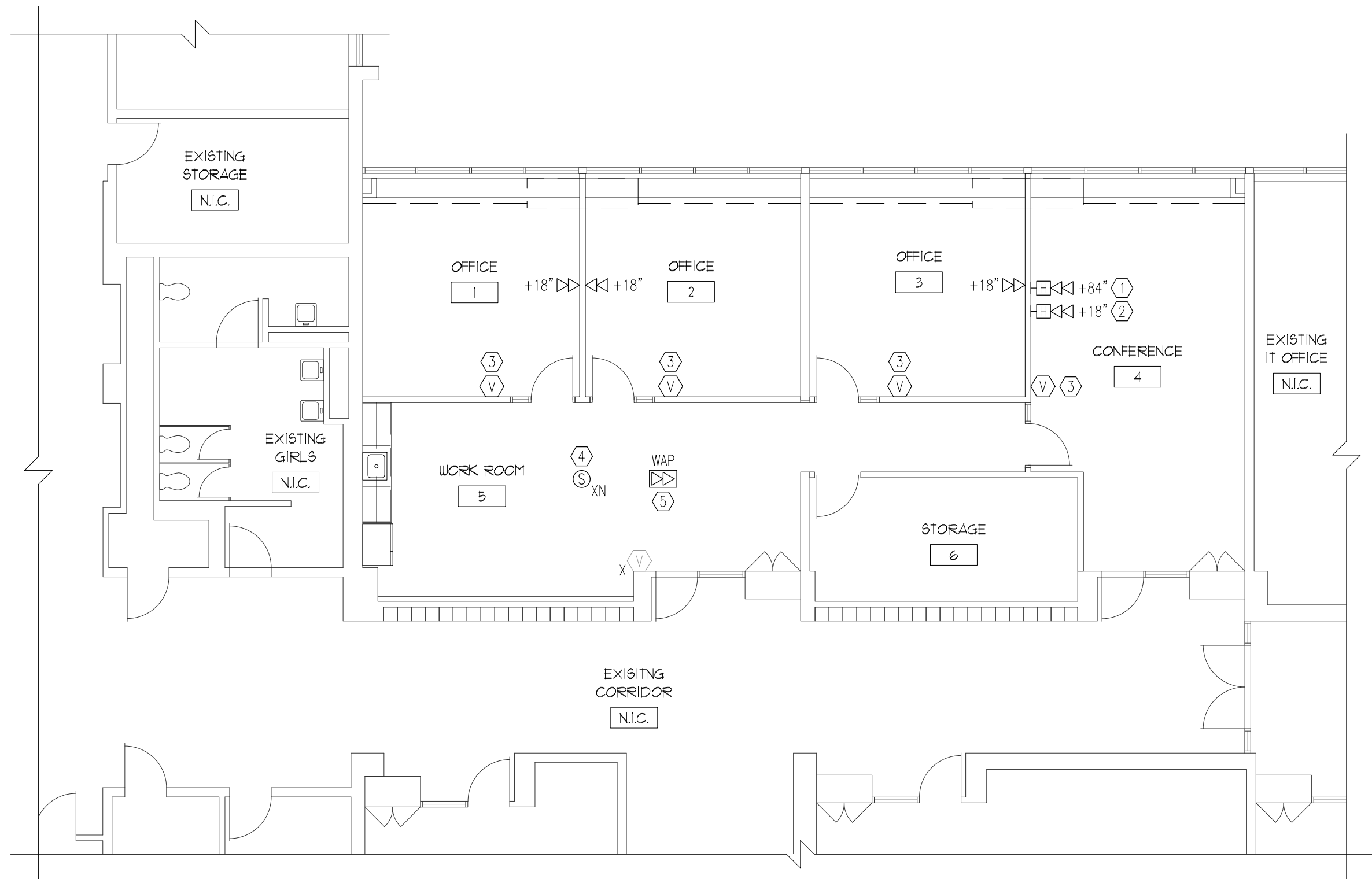
2 PARTIAL FLOOR PLAN - SYSTEMS 1/8" = 1'-0"
