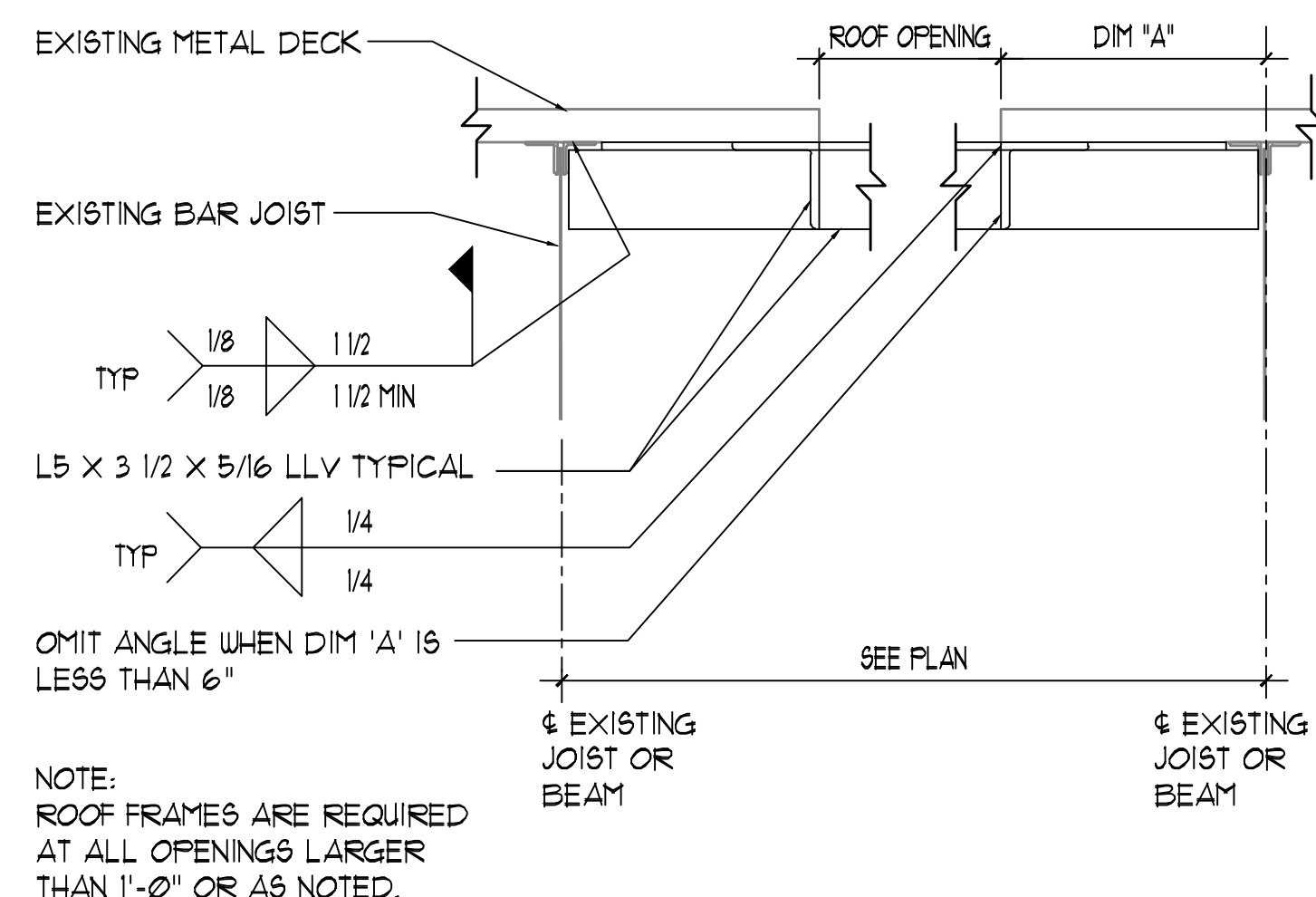
4 TYPICAL OPENING IN EXISTING ROOF DETAIL 1 1/2" = 1'-0"
