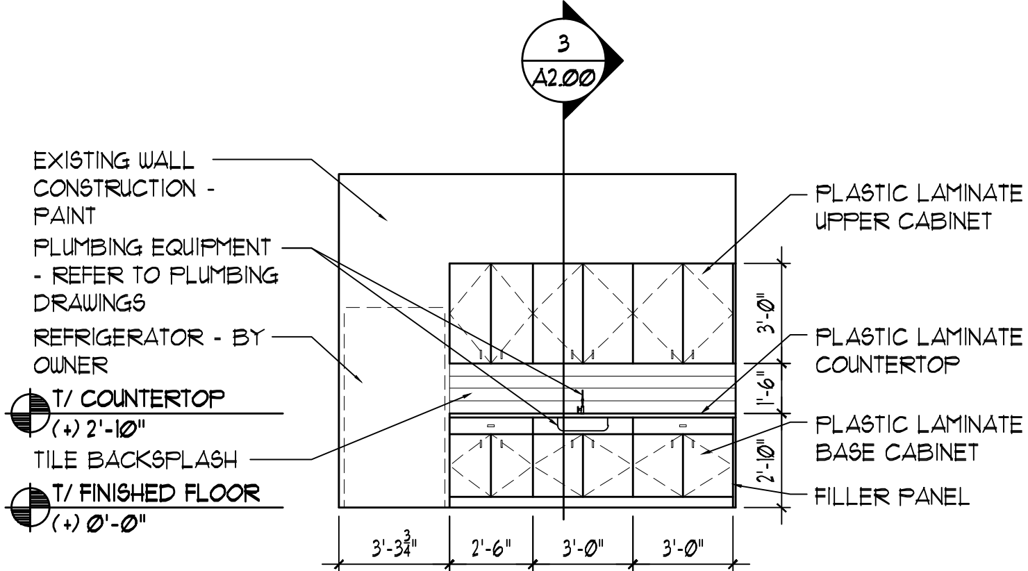
4 INTERIOR ELEVATION - ALTERNATE 1/4" = 1'-0"
