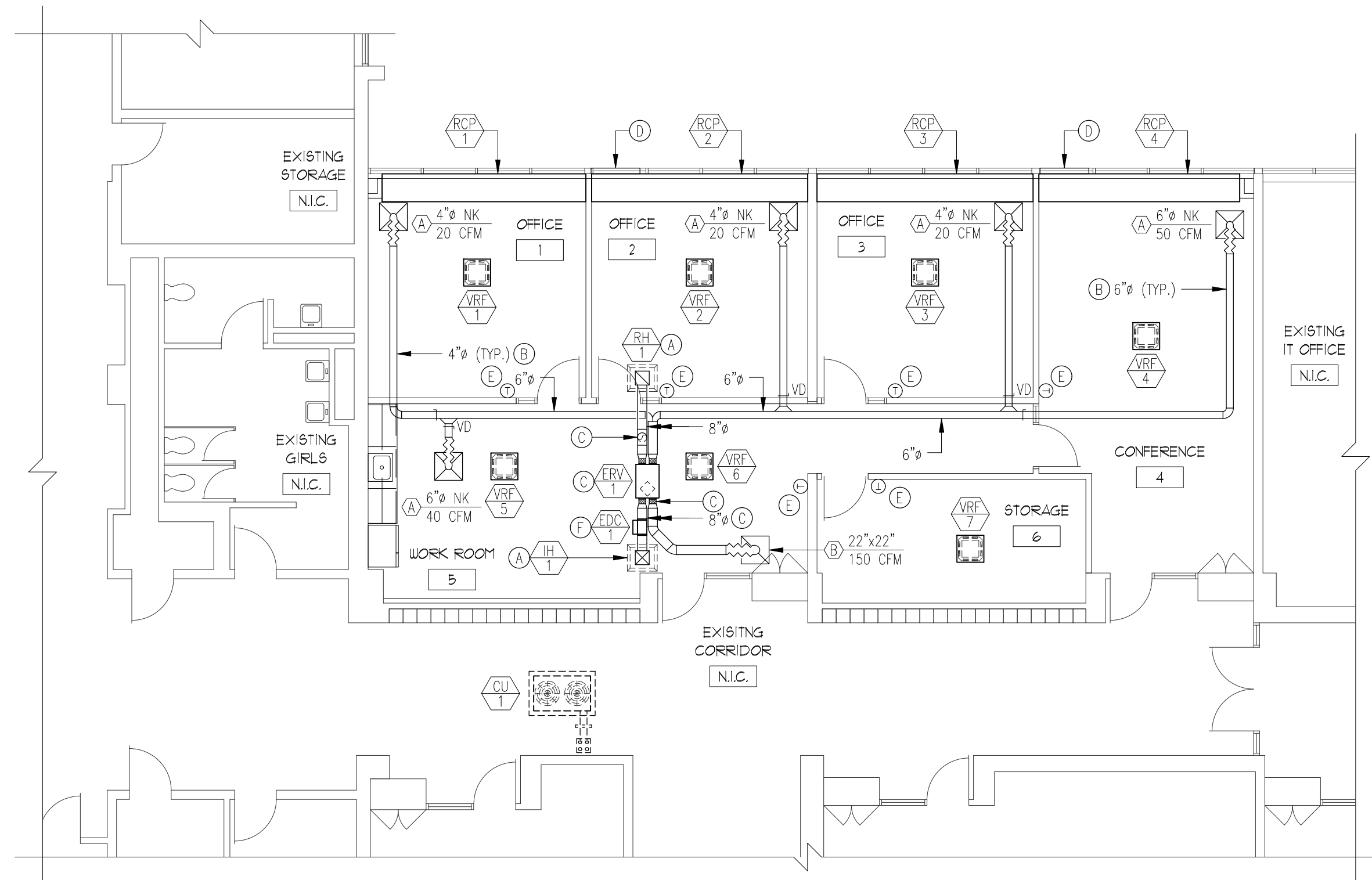
1 PARTIAL FLOOR PLAN - VENTILATION 1/8" = 1'-0"
