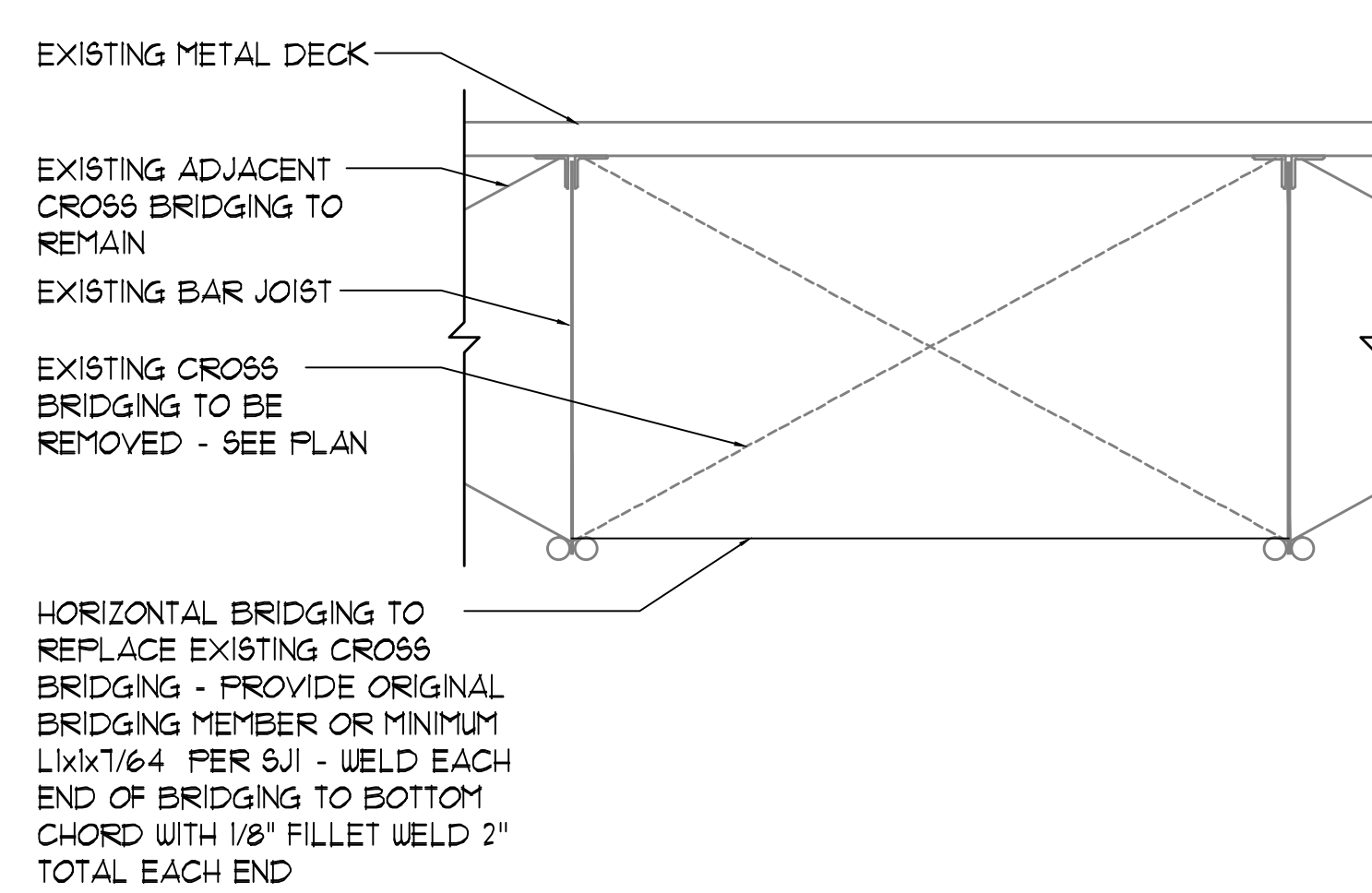
6 TYPICAL HORIZONTAL BRIDGING DETAIL 1 1/2" = 1'-0"
