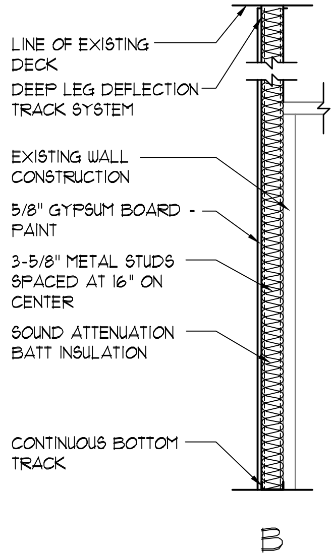
WALL TYPES NOT TO SCALE
