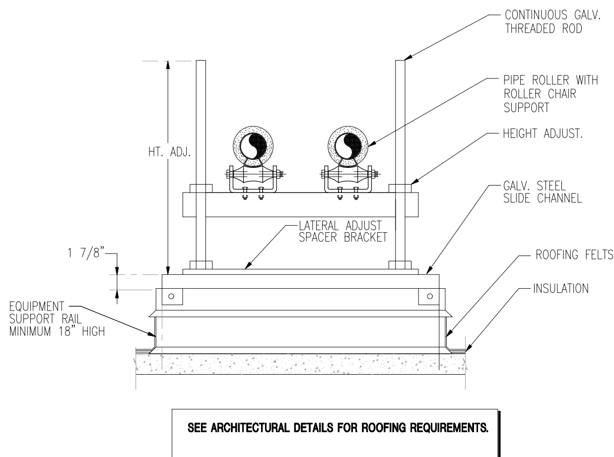
11 ROOF PIPE MOUNTING PEDESTAL M4.10 NO SCALE
