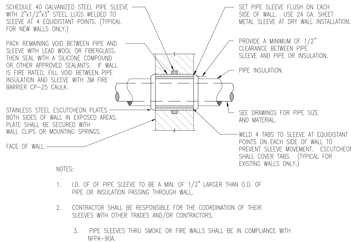
9 PIPE SLEEVE THRU INTERIOR RATED WALL DETAIL M4.10 NO SCALE
