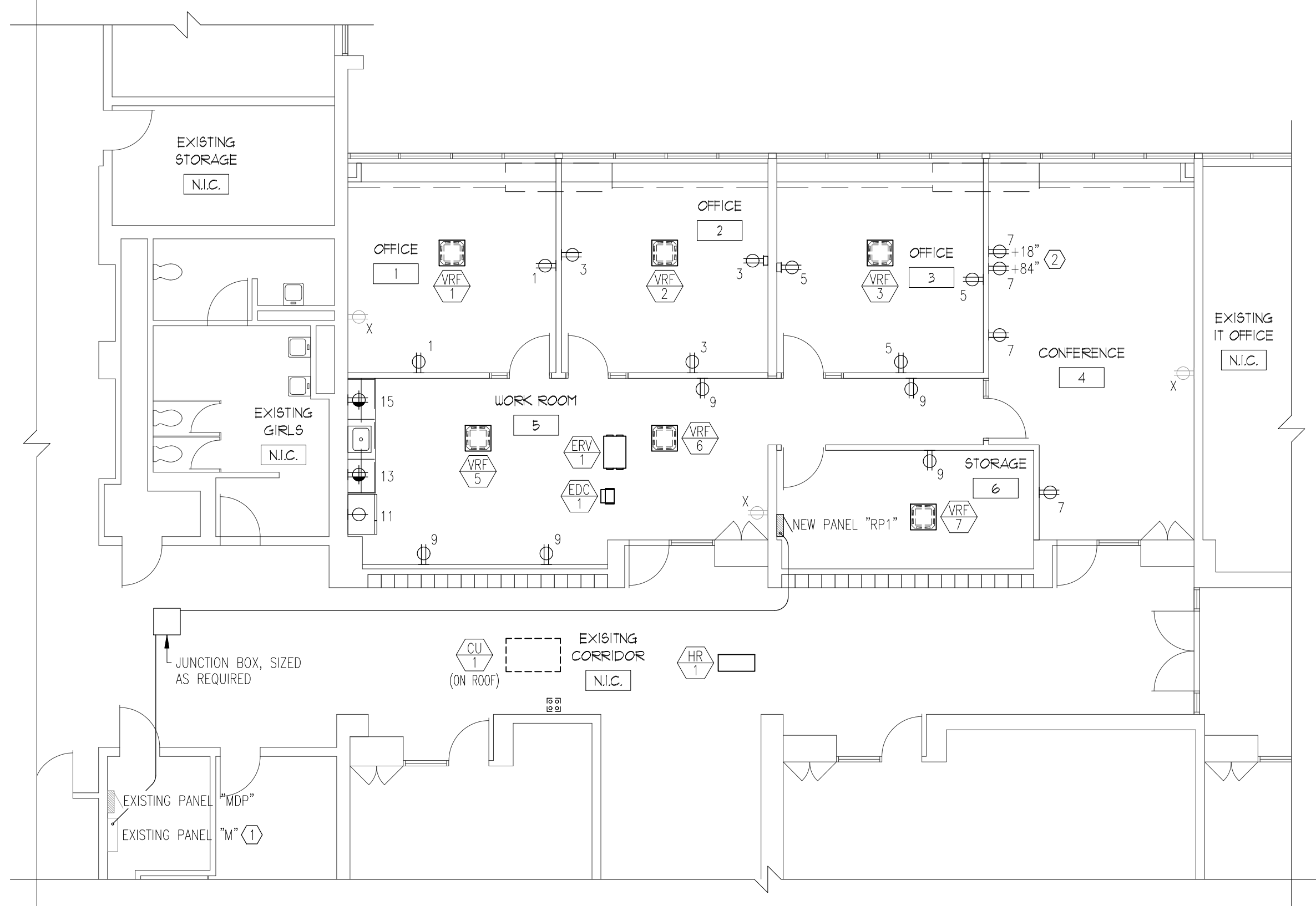
1 PARTIAL FLOOR PLAN - POWER 1/8" = 1'-0"
