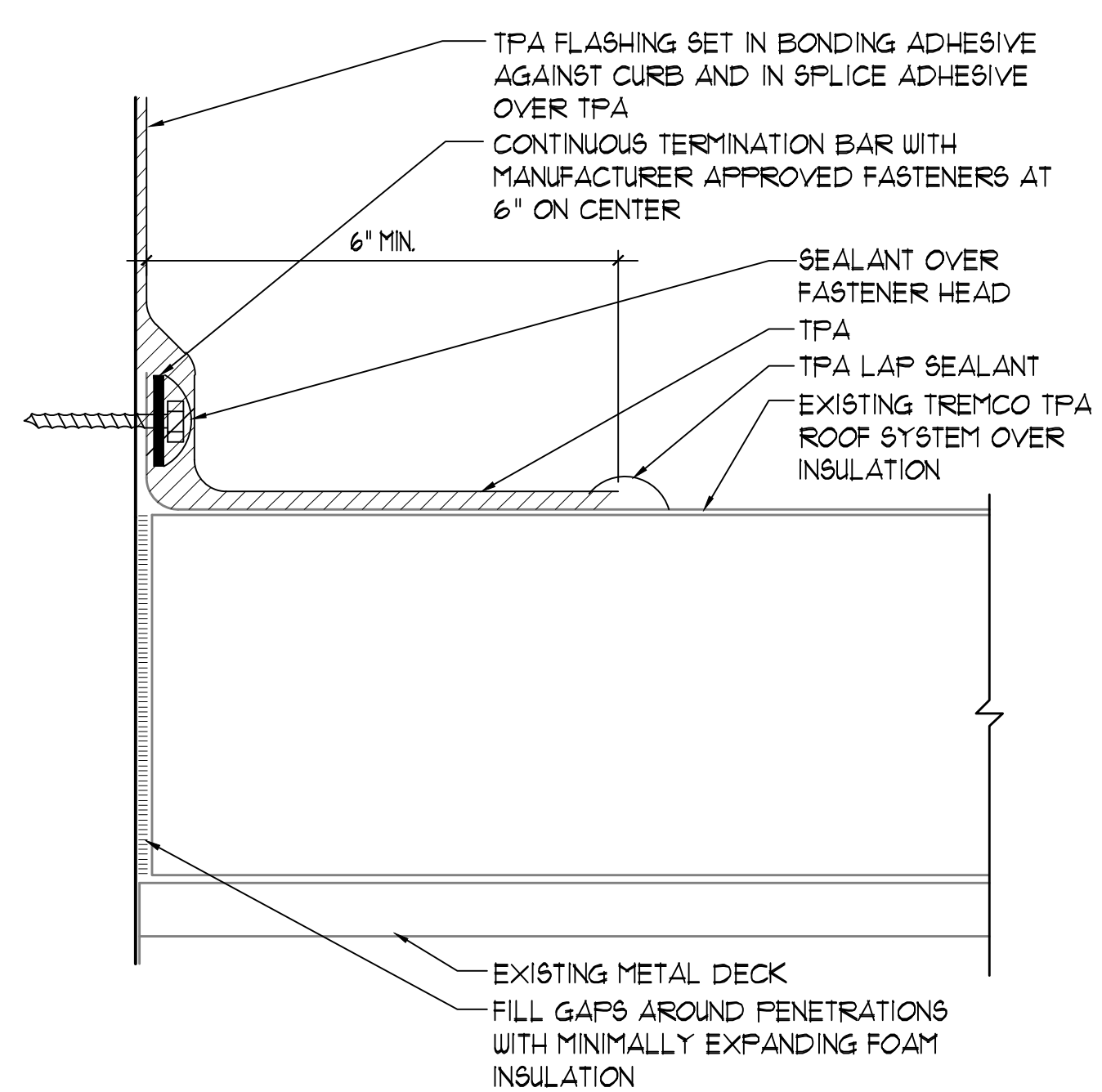
3 TYPICAL SPM ANCHOR STRIP DETAIL 6" = 1'-0"
