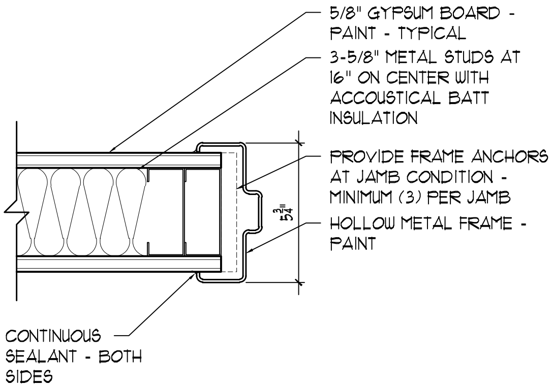
2 JAMB DETAIL 3" = 1'-0"
