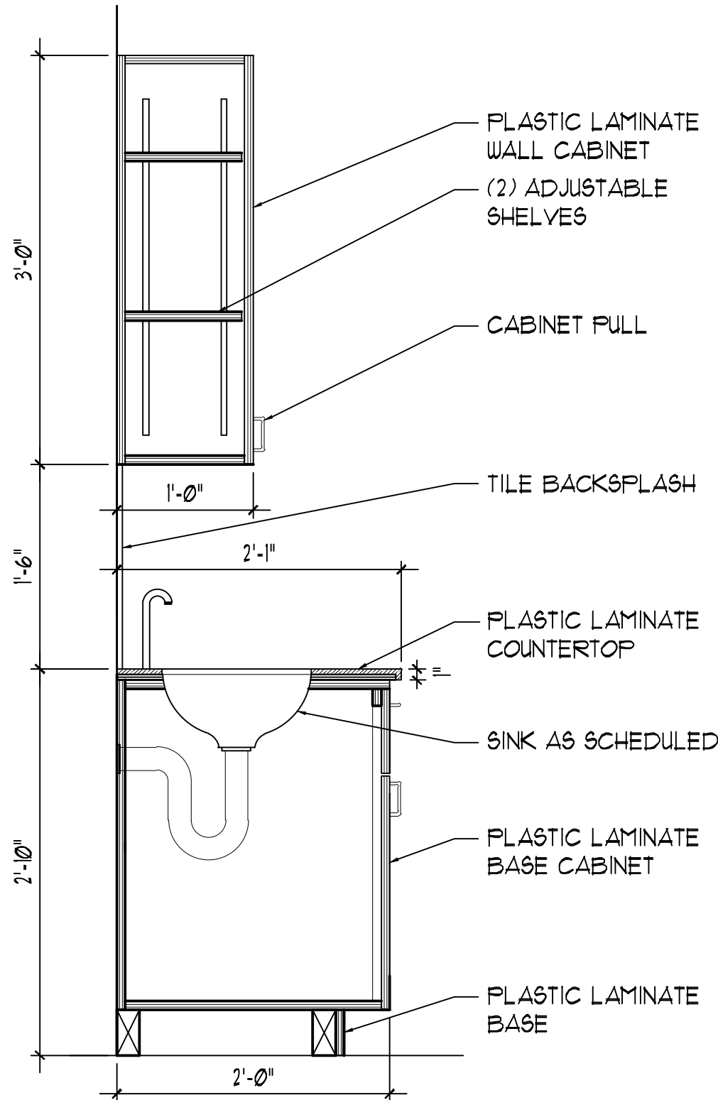
3 CASEWORK SECTION - ALTERNATE 1" = 1'-0"
