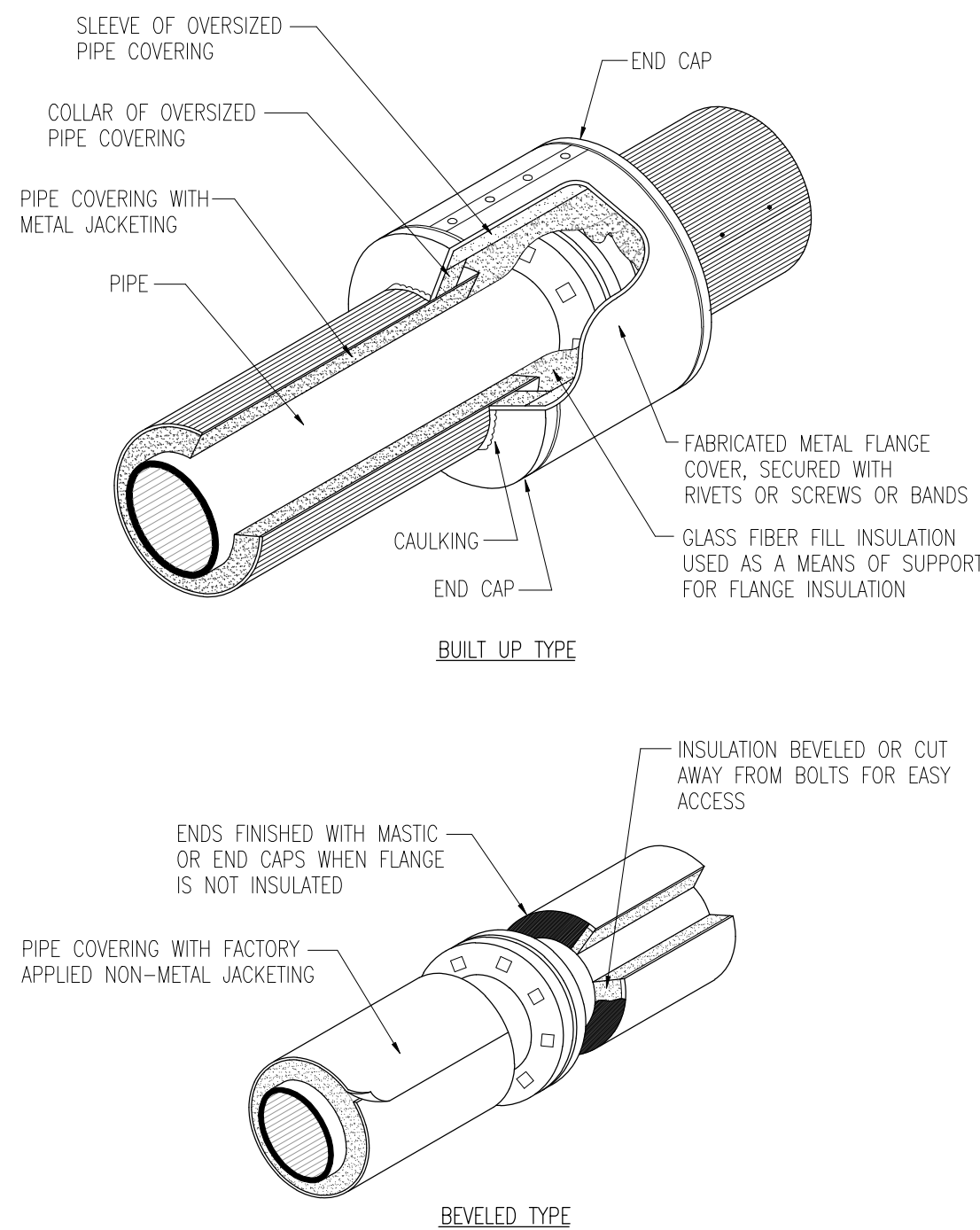
2 IN-LINE FLANGE INSULATION M4.10 NO SCALE
