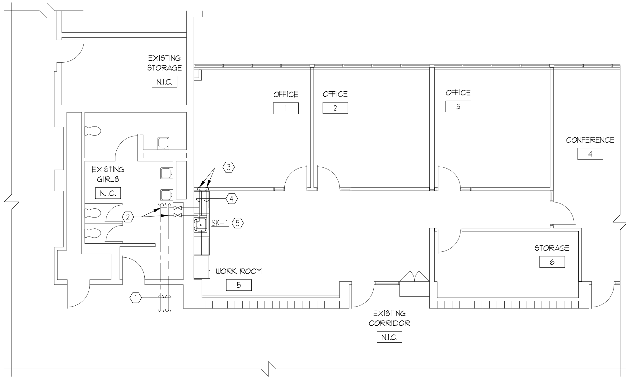
2 PARTIAL FLOOR PLAN - PLUMBING - WATER 1/8" = 1'-0"
