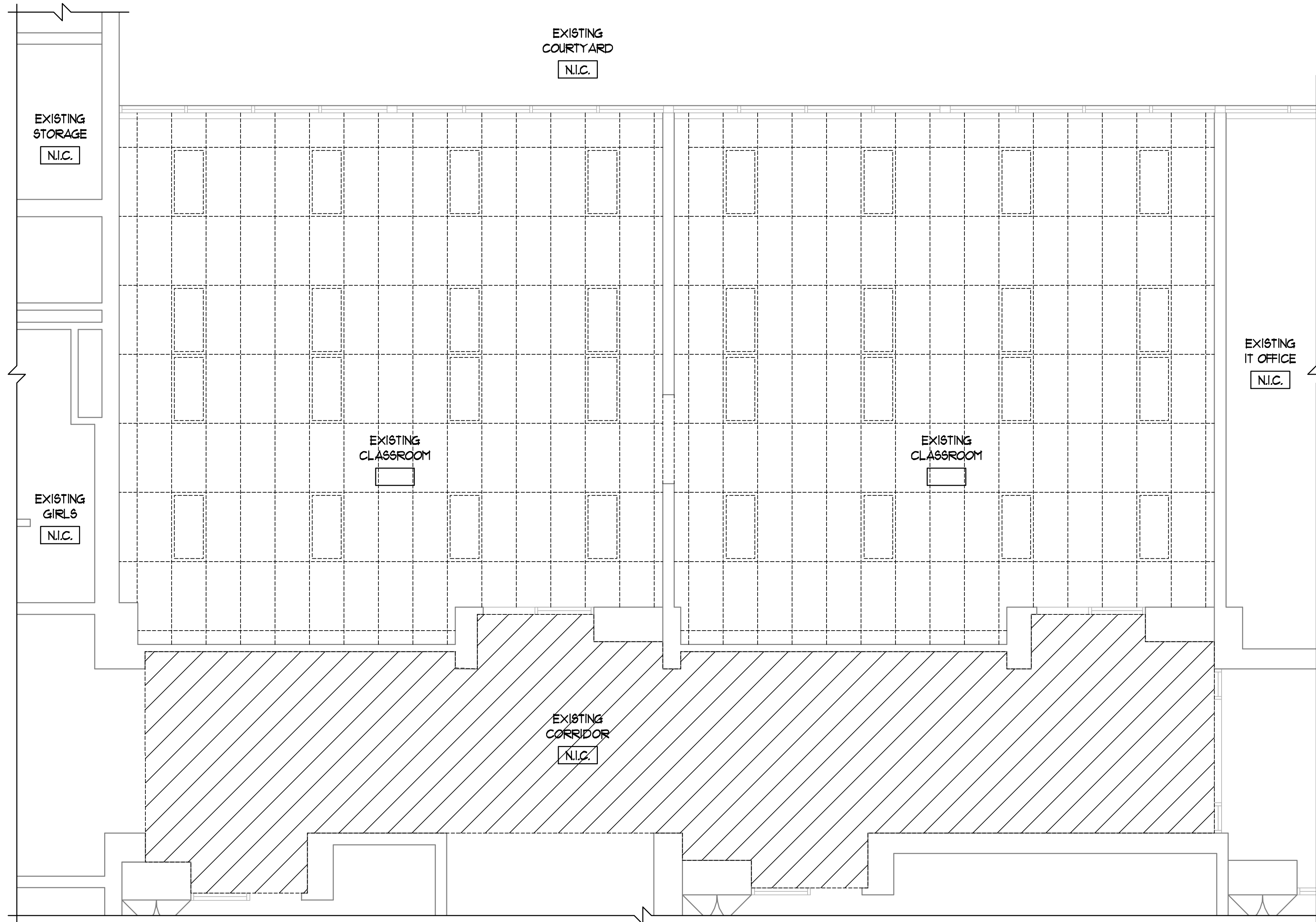
1 PARTIAL EXISTING REFLECTED CEILING PLAN 1/8" = 1'-0"
