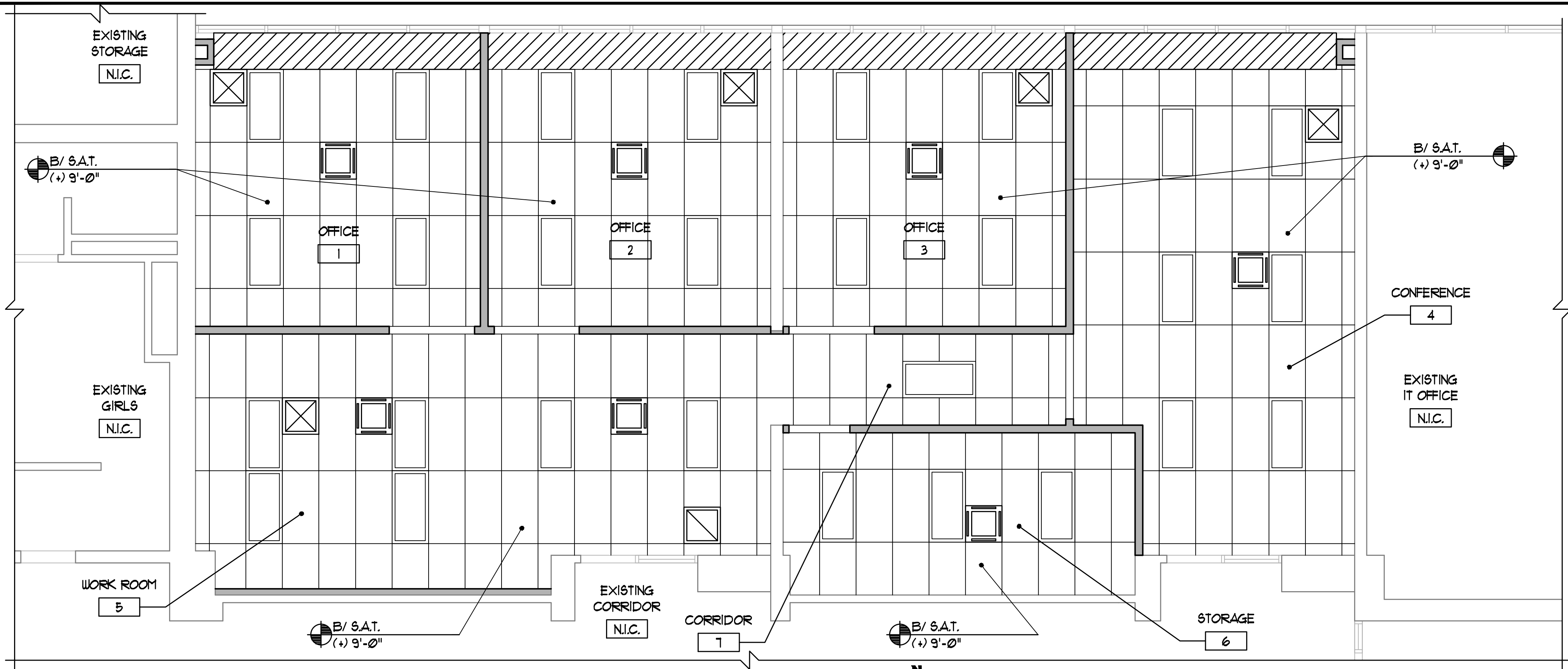
1 PARTIAL REFLECTED CEILING PLAN 1/4" = 1'-0"
