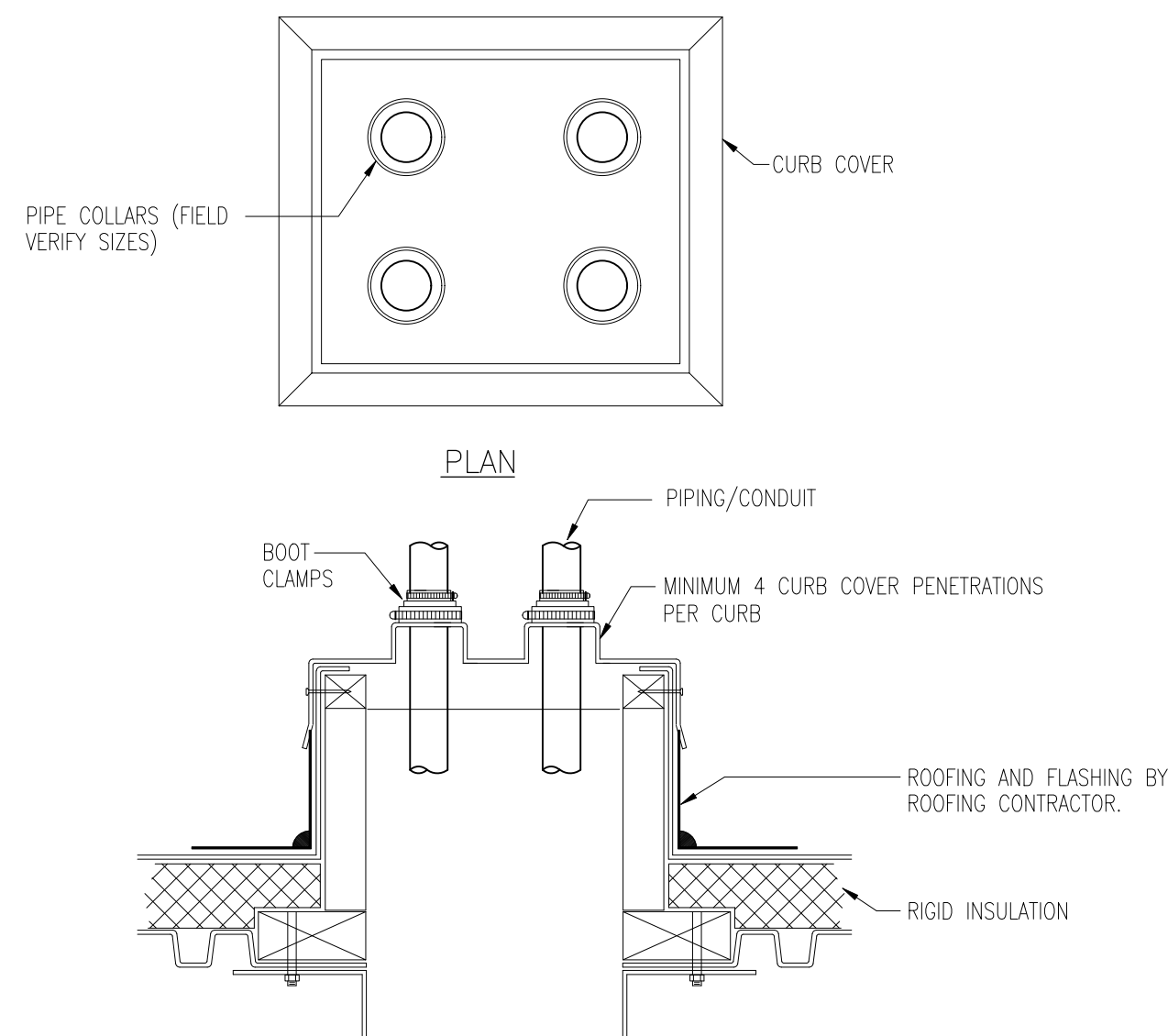
10 PIPE CURB ASSEMBLY DETAIL M4.10 NO SCALE
