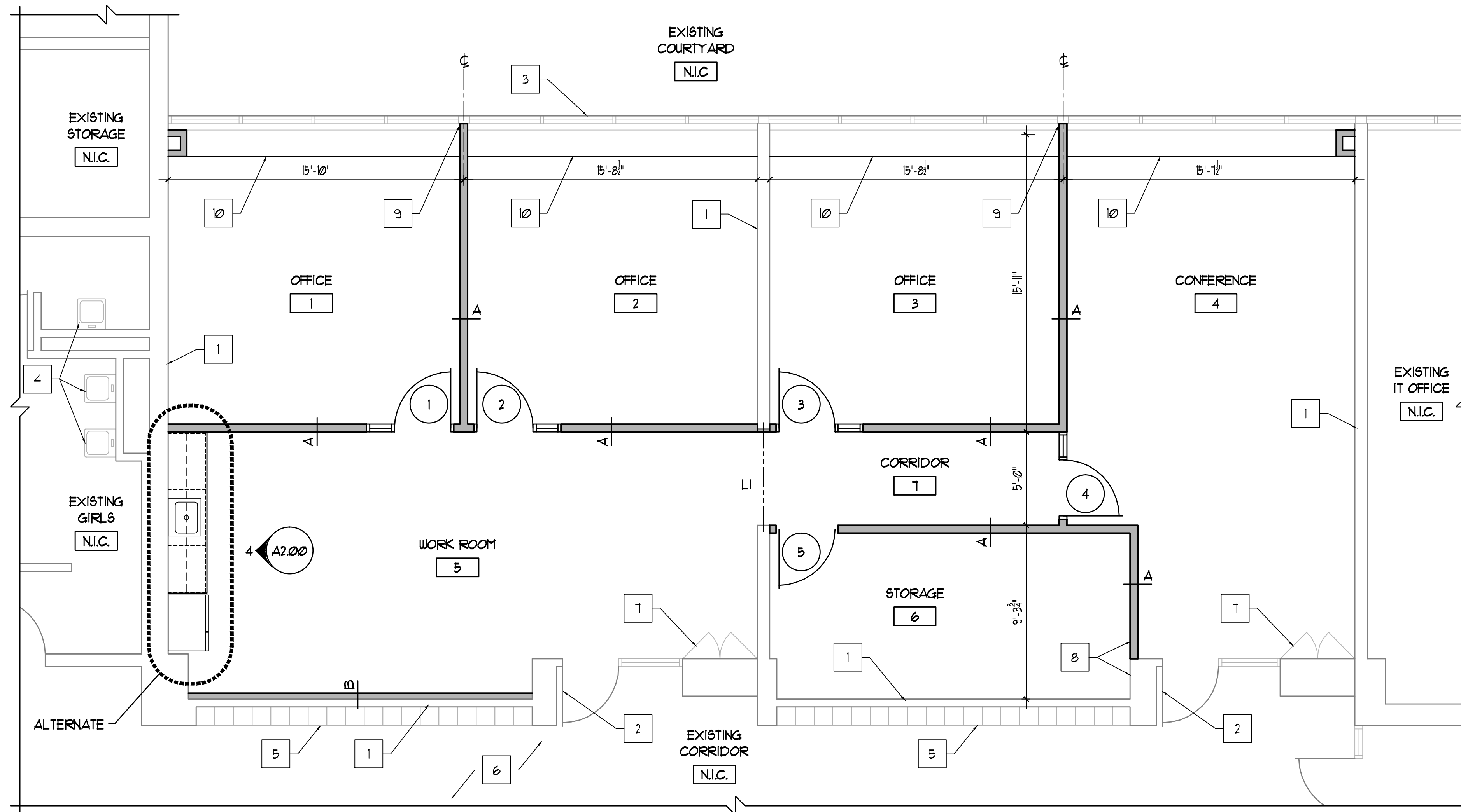
1 PARTIAL FLOOR PLAN 1/4" = 1'-0"
