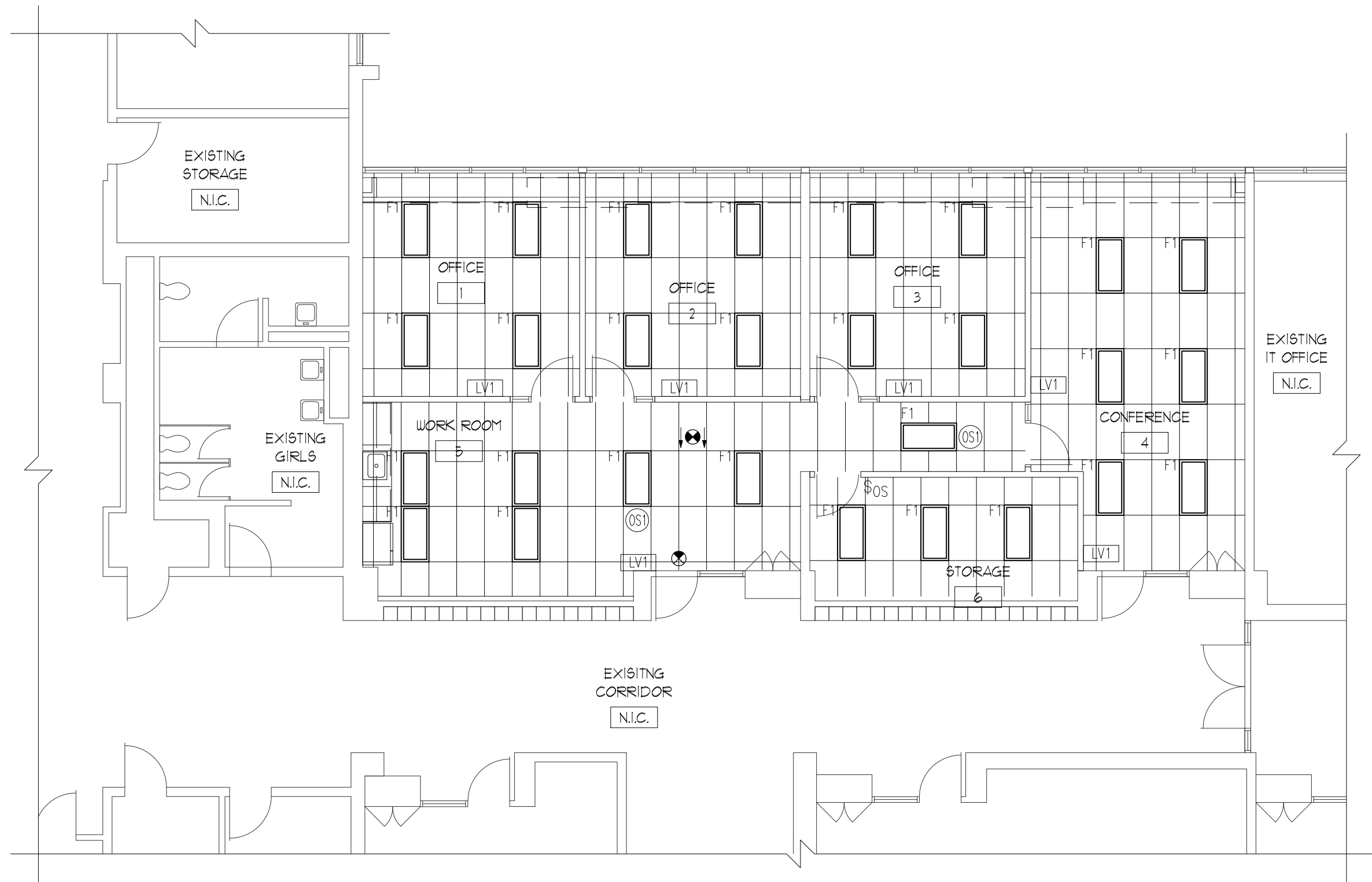
1 PARTIAL FLOOR PLAN - LIGHTING 1/8" = 1'-0"
