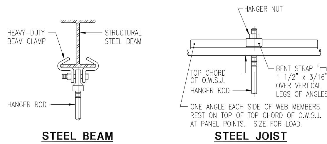
5 PIPE HANGER DETAILS M4.10 NO SCALE
