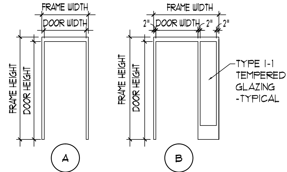
FRAME TYPES NOT TO SCALE
