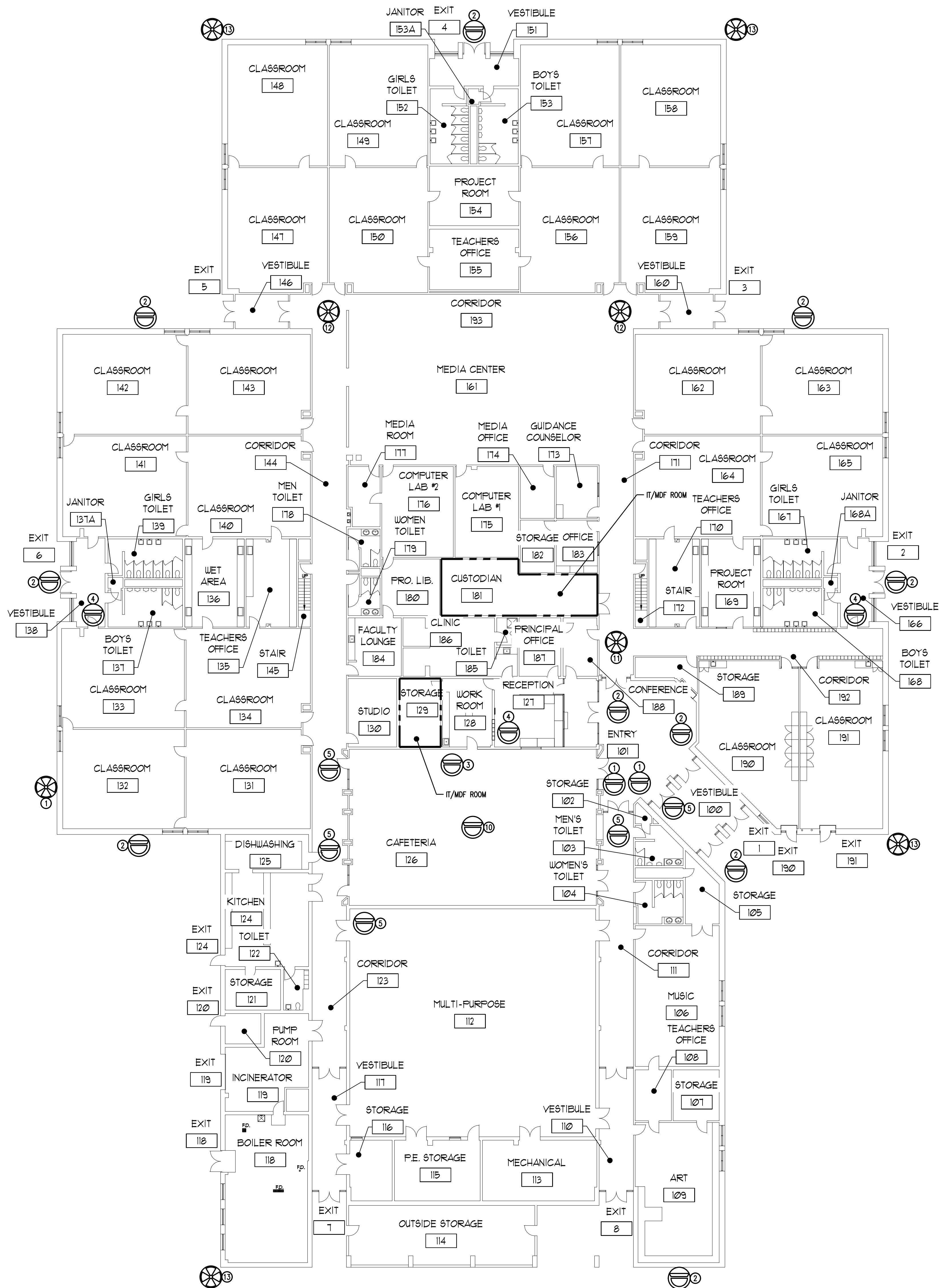
1 FIRST FLOOR PLAN - ELECTRICAL 1/16" = 1'-0"
