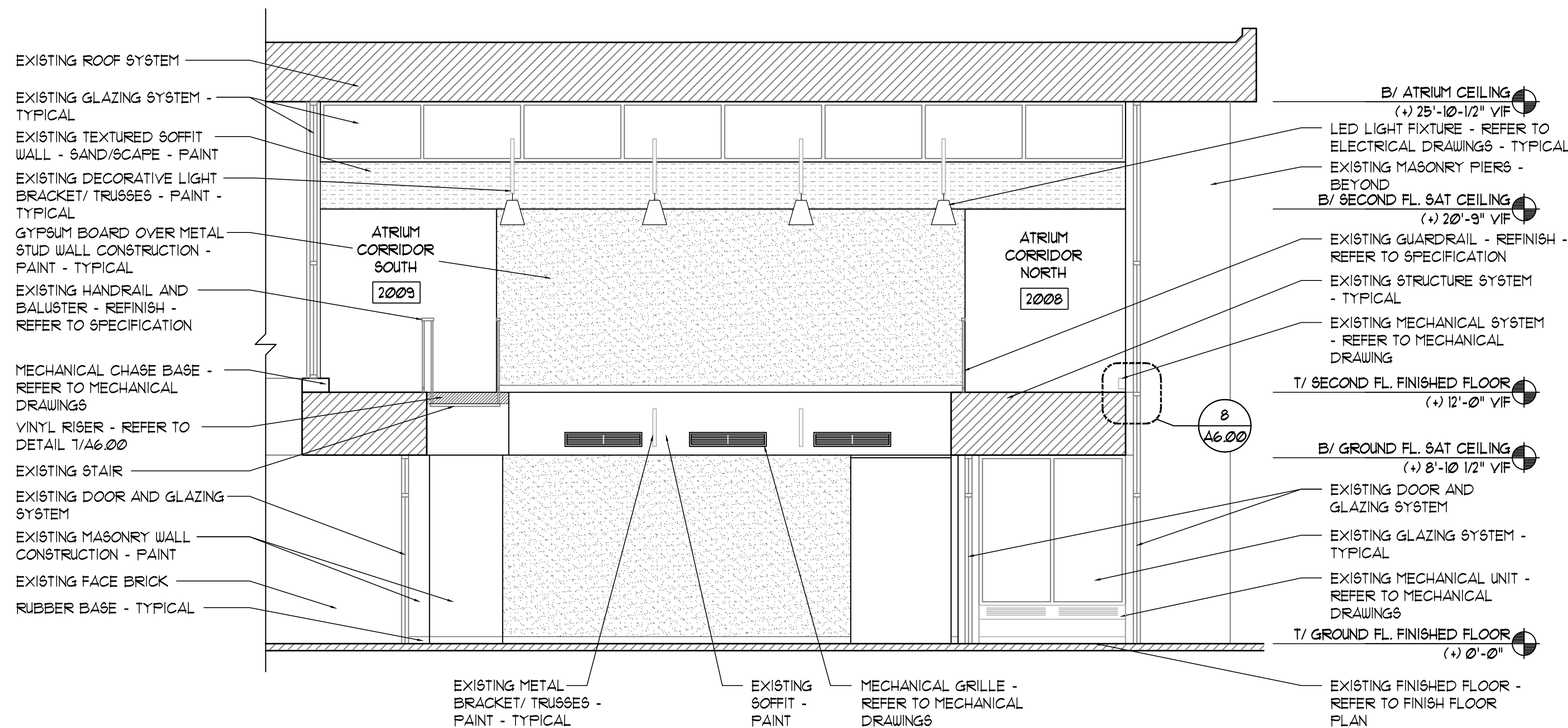
1 PARTIAL BUILDING SECTION 1/4" = 1'-0"
