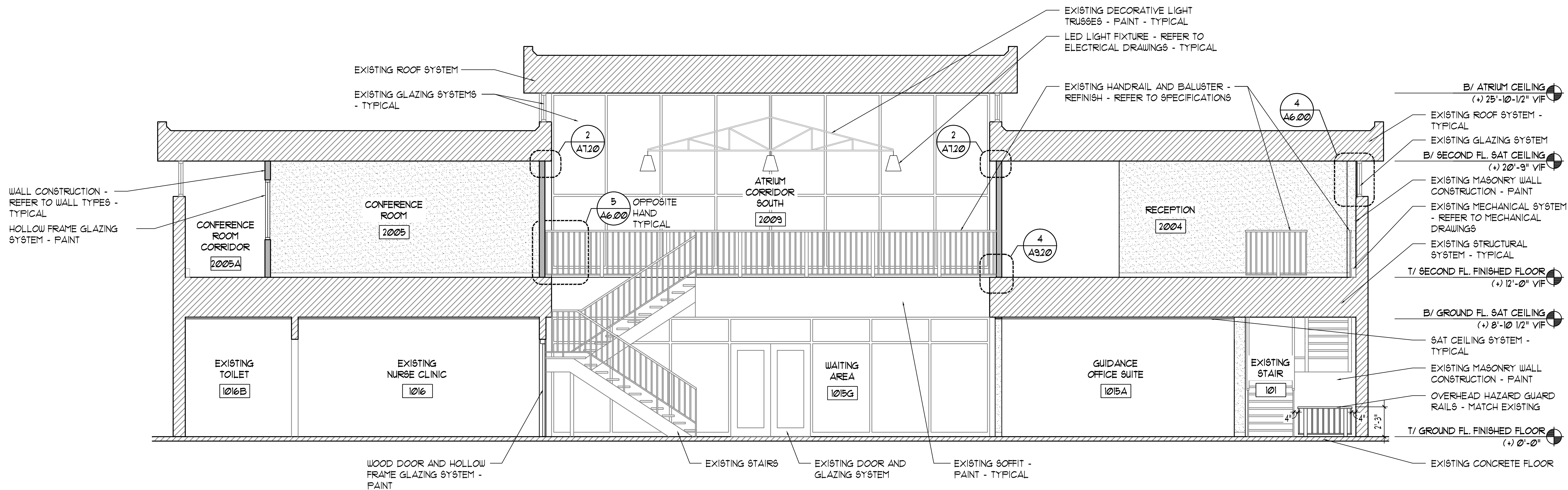
2 BUILDING SECTION 1/4" = 1'-0"
