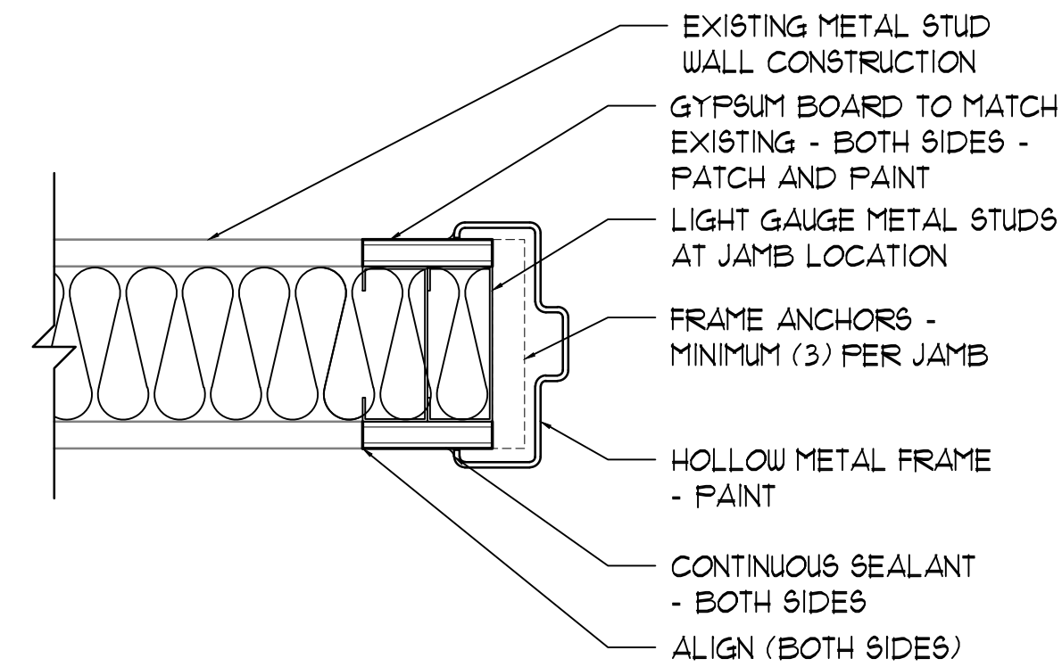
5 JAMB DETAIL 3" = 1'-0"
