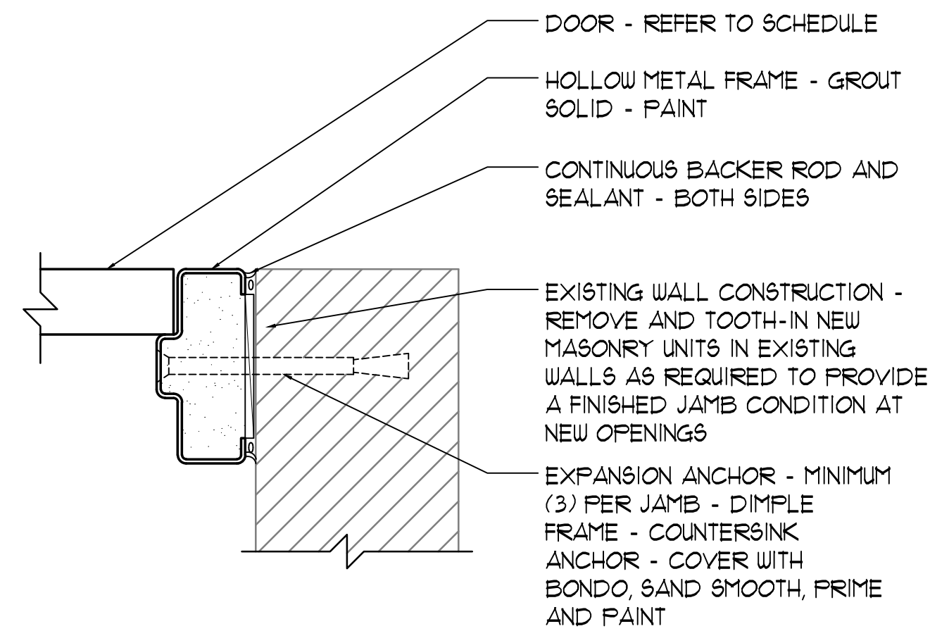
8 JAMB DETAIL 3" = 1'-0"
