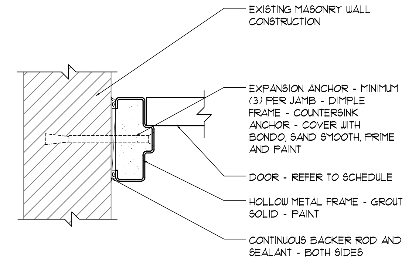
7 JAMB DETAIL 3" = 1'-0"
