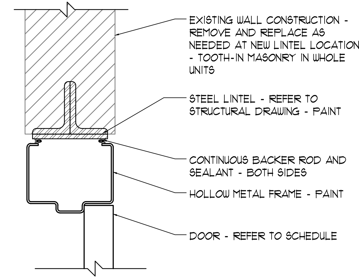
3 HEAD DETAIL 3" = 1'-0"
