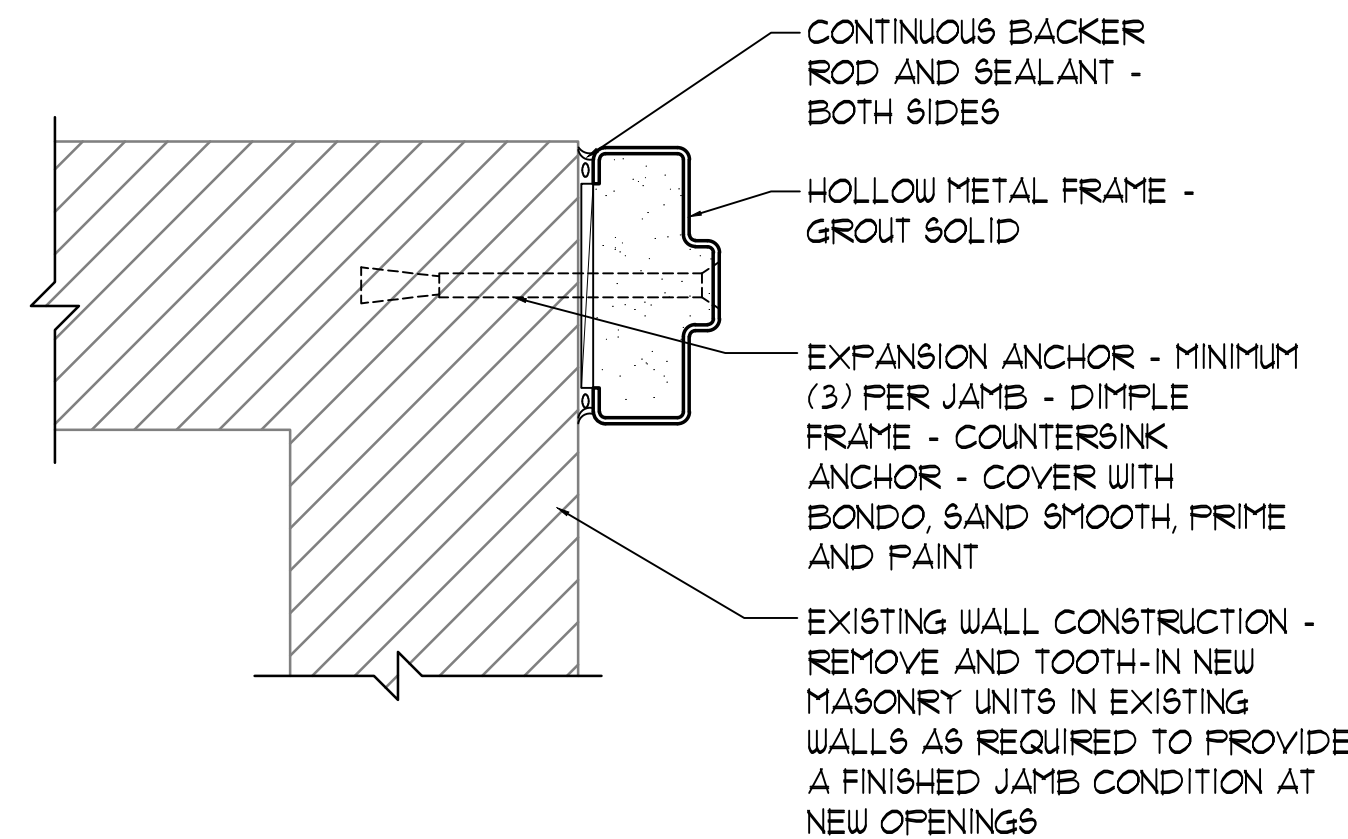
9 JAMB DETAIL 3" = 1'-0"
