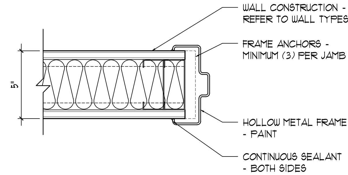
4 JAMB DETAIL 3" = 1'-0"
