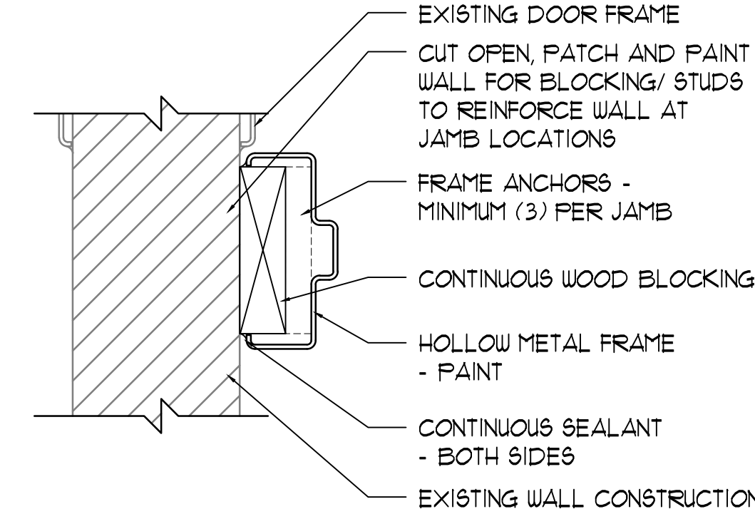
6 JAMB DETAIL 3" = 1'-0"
