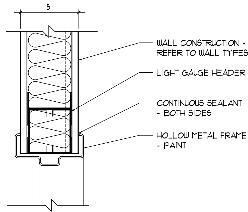
1 HEAD DETAIL 3" = 1'-0"
