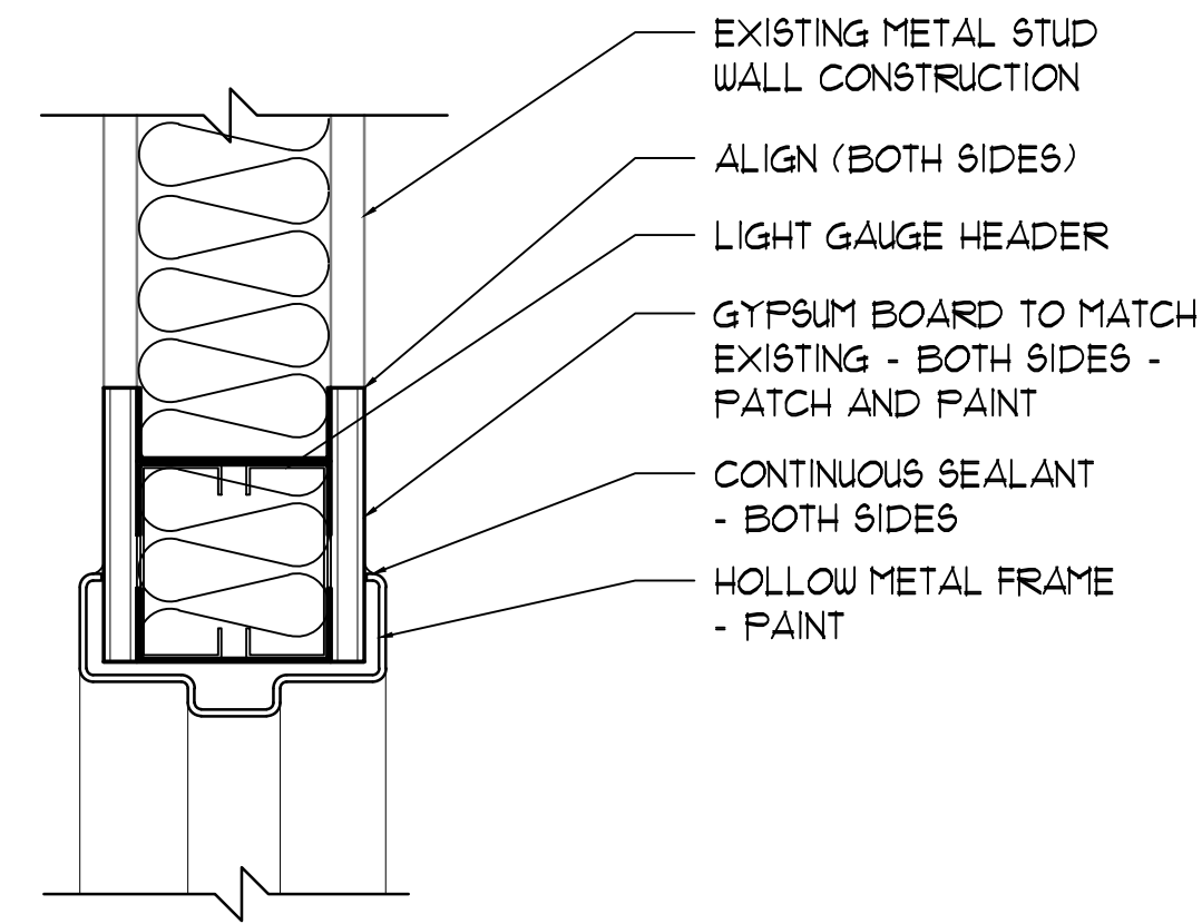
2 HEAD DETAIL 3" = 1'-0"
