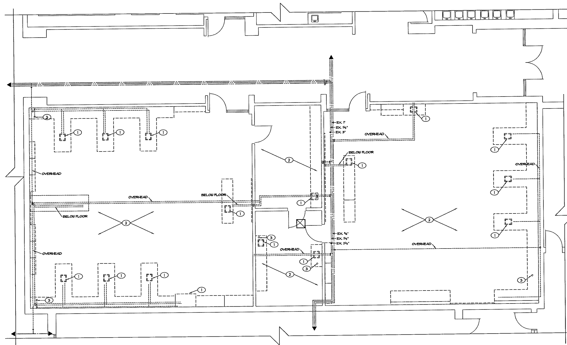
1 PARTIAL FIRST FLOOR PLAN - PLUMBING DEMOLITION 1/4" = 1'-0"
