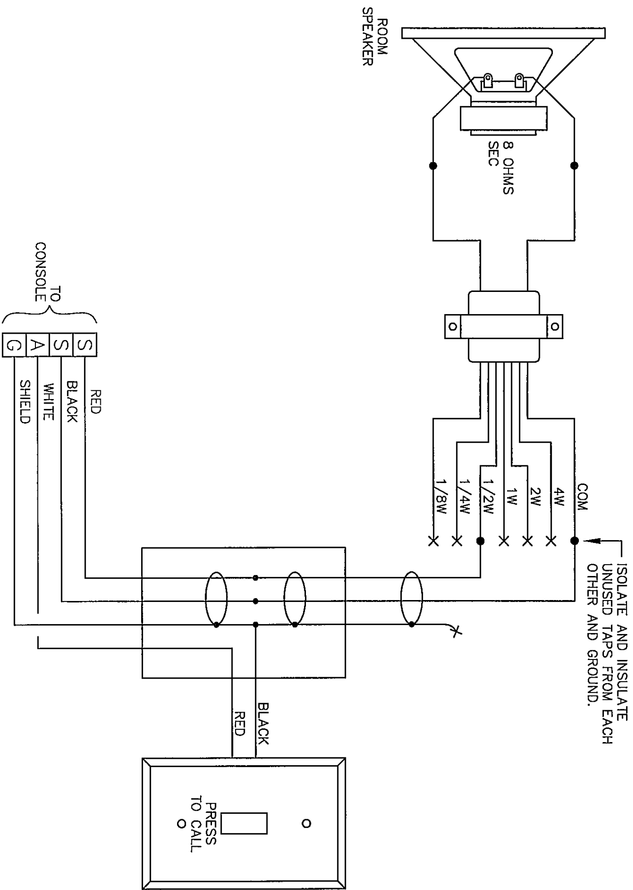
CALL IN SWITCH CIRCUIT CONNECTIONS DETAIL A
