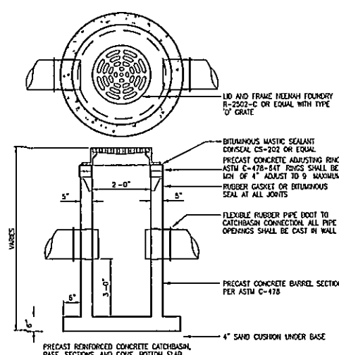
Typical Yard Inlet
