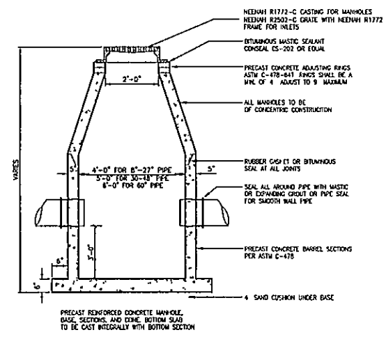
Storm Sewer Manhole or Inlet
