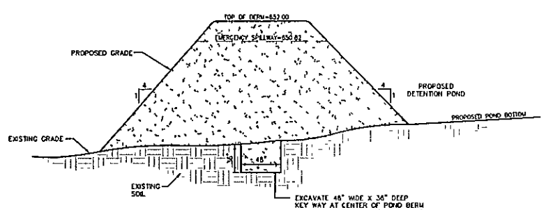
Pond Berm Detail
