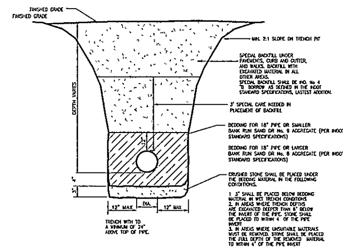
Class 'B' Pipe Trench and Bedding
