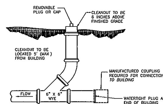
Cleanout for Pavement or Turf Areas
