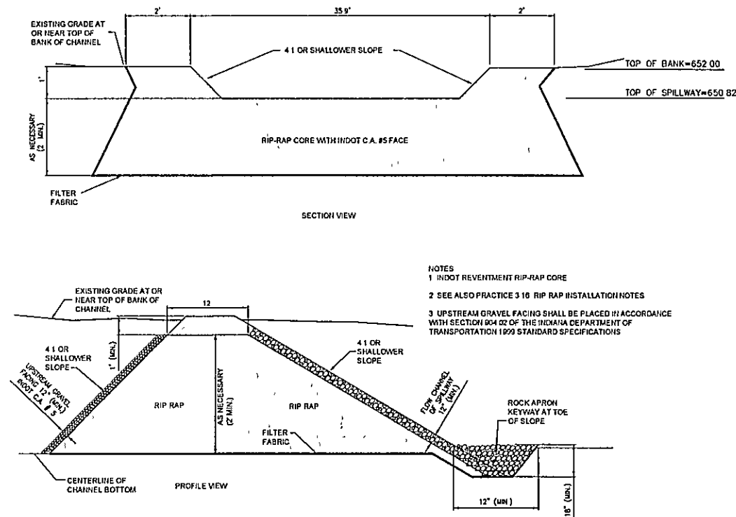
Emergency Spillway Detail
