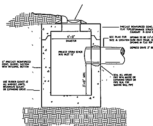
Standard Curb Inlet
