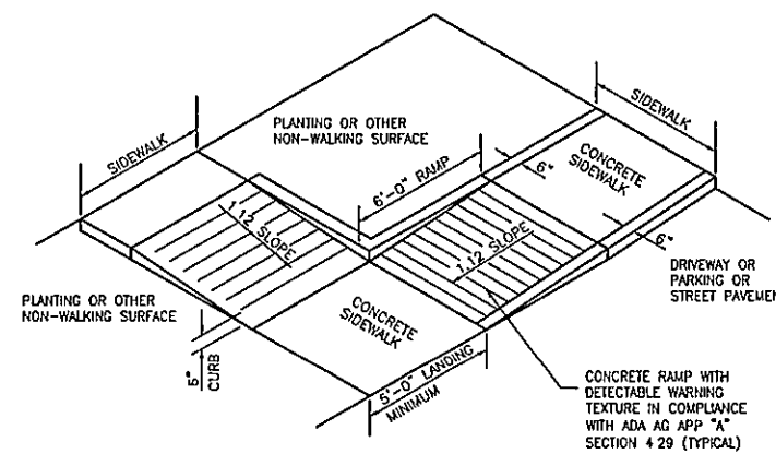
Returned Curb Accessibility Ramp
