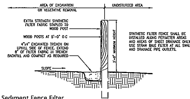
Sediment Fence Filter Sedimentation Control Structures
