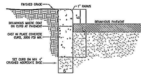
Standard 6" Curb Detail
