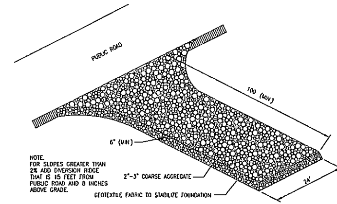
Temporary Gravel Construction Entrance
