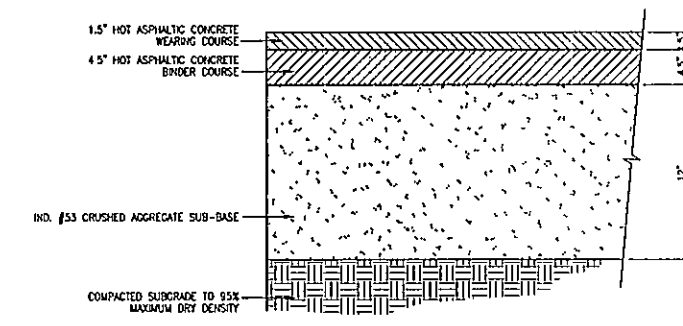
Parking Lot Pavement Detail
