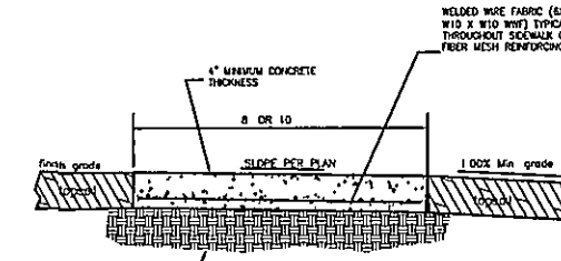
Concrete Sidewalk Detail
