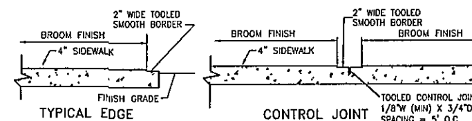
Concrete Sidewalk Finishing Details
