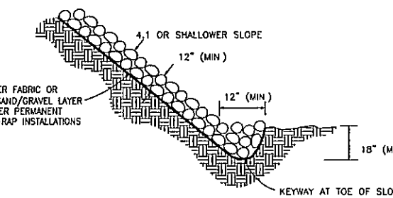
Rip Rap Installation
