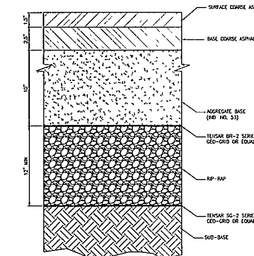
Pavement Section - Poor Soils
