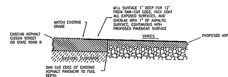
Lap Joint Detail - Asphalt Pavement
