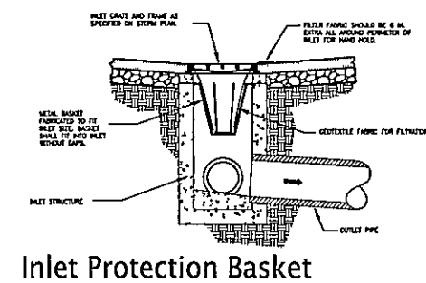
Inlet Protection Basket
