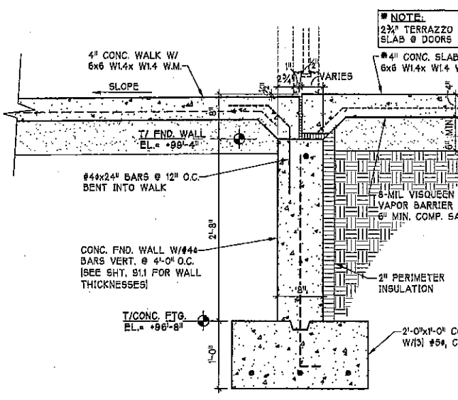
2 FND. WALL DTL. @ DOORS S1.2 (@ 12" WALL) 1" = 1'-0"
