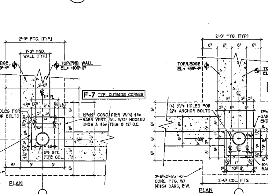
7 COLUMN PIER/FTG. DETAIL S1.2 (TYP. @ F-7 FTG. - OUTSIDE CORNERS) 1" = 1'-0"
