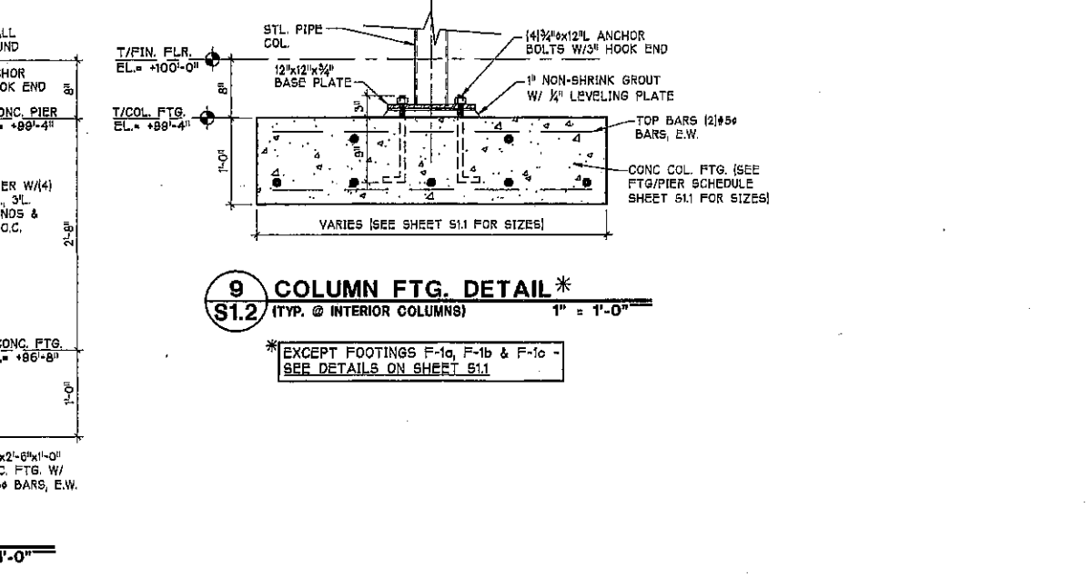
12 CANOPY COLUMN DTL. S1.2 (TYP. OF 3) 3" = 1'-0"
