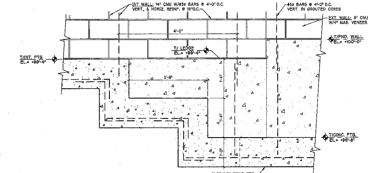
4 STEP FTG./FND. WALL DETAIL S1.2 1" = 1'-0"
