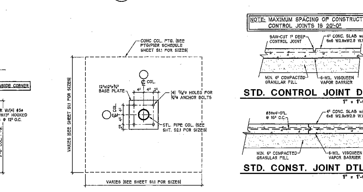
8 COLUMN PIER/FTG. DETAIL S1.2 (TYP. @ F-8 FTG. - INSIDE CORNERS) 1" = 1'-0"
