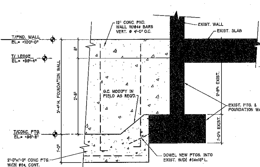
3 FND. WALL DTL. S1.2 (@ EXIST. FND. WALL) 1" = 1'-0"
