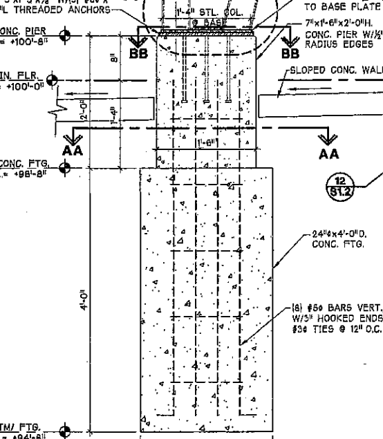
9 COLUMN FTG. DETAIL S1.2 (TYP. @ INTERIOR COLUMNS) 1" = 1'-0"
