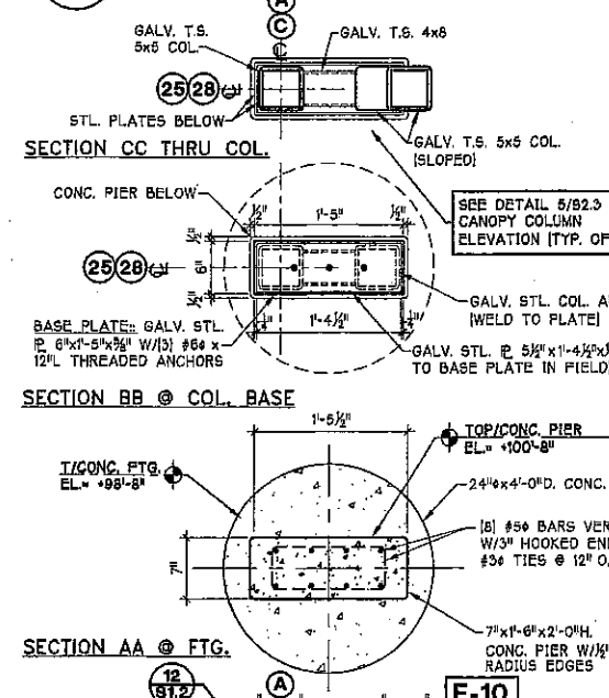
5 CANOPY FTG. DETAIL S1.2 (TYP. OF 3) 1" = 1'-0"
