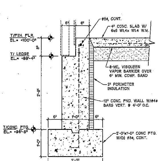
1 TYP. FND. WALL DETAIL S1.2 (@ 12" WALL) 1" = 1'-0"
