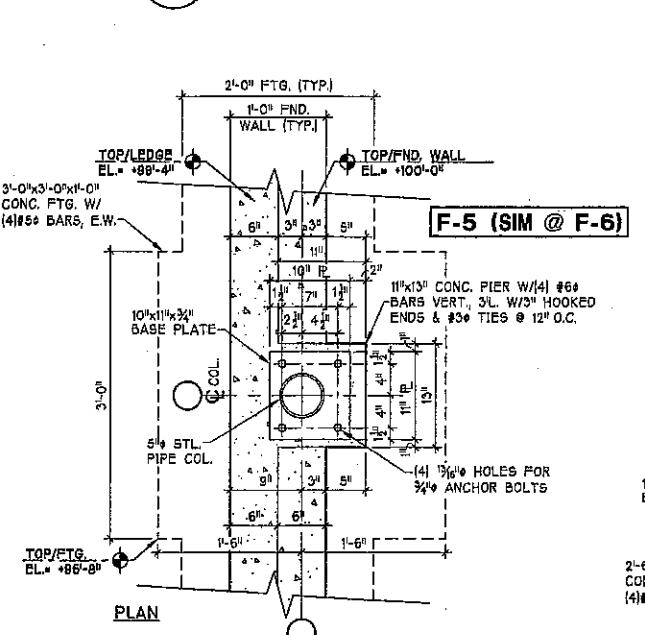
6 COLUMN PIER/FTG. DETAIL S1.2 (TYP. @ F-5 FTG. - SIM @ F-6 FTG.) 1" = 1'-0"
