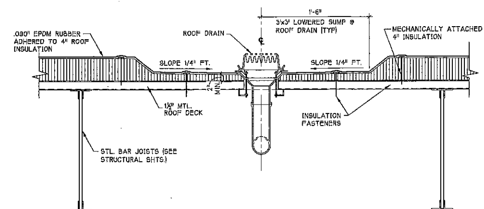
1 TYP. ROOF DRAIN DETAIL A8.1 1 1/2" = 1'-0"
