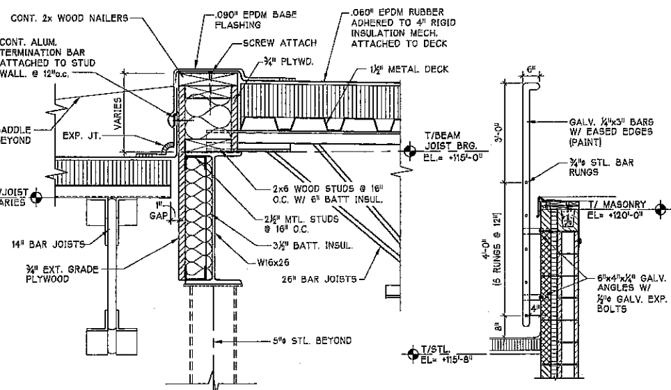
2 ROOF EXP. JOINT DTL. A8.1 1 1/2" = 1'-0"
