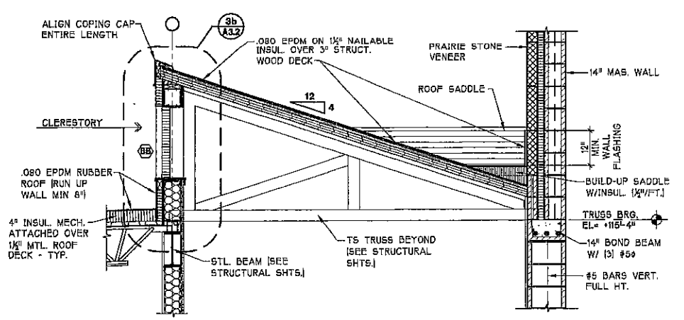
SECTION 'B-B' / A8.1 1/2" = 1'-0"
