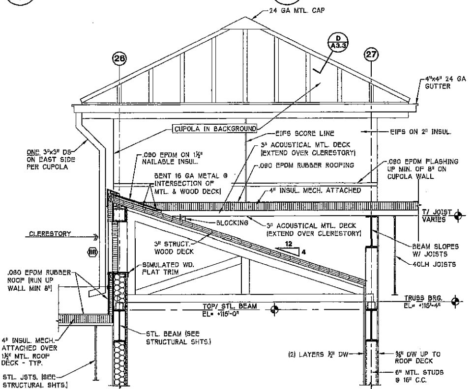
SECTION 'A-A' / A8.1 1/2" = 1'-0"
