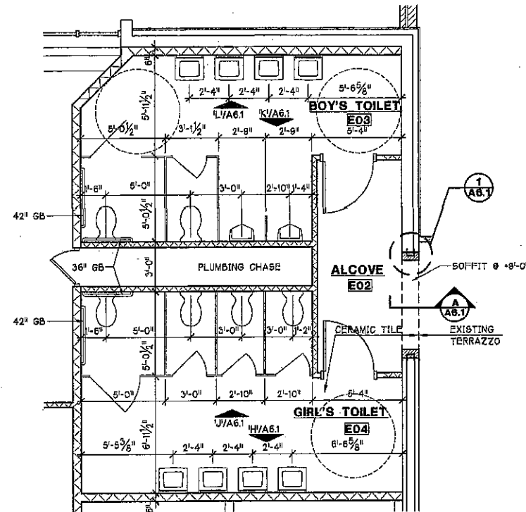
ENLARGED TOILET PLAN
