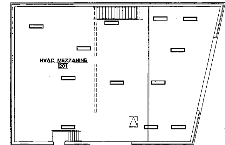
REFLECTED CEILING PLAN - MEZZANINE
