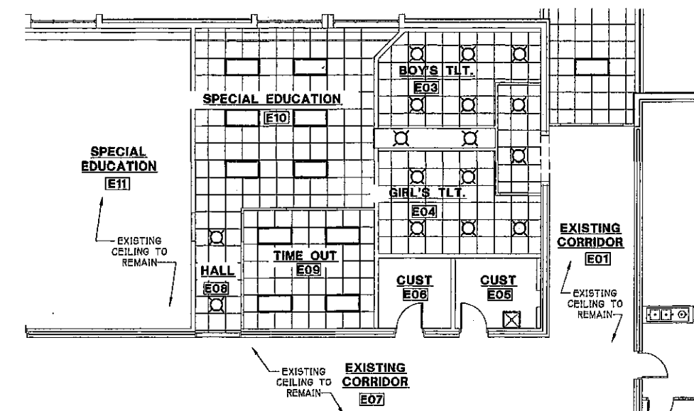
REFLECTED CEILING PLAN - EXISTING BUILDING
