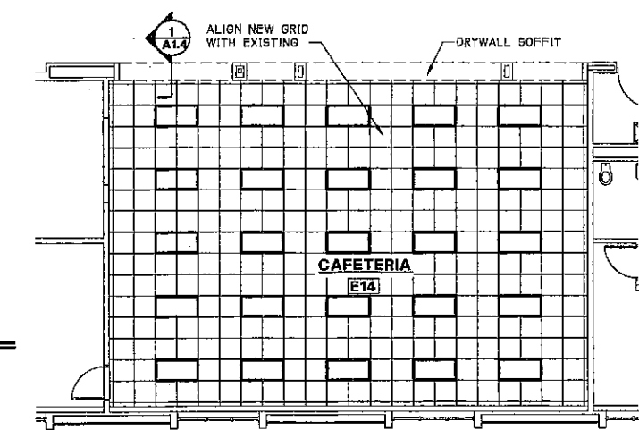
REFLECTED CEILING PLAN - CAFETERIA
