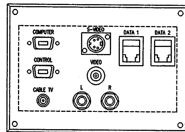
5 I/O PODIUM PLATE DETAILS T3.3 SCALE: NTS PODIUM
