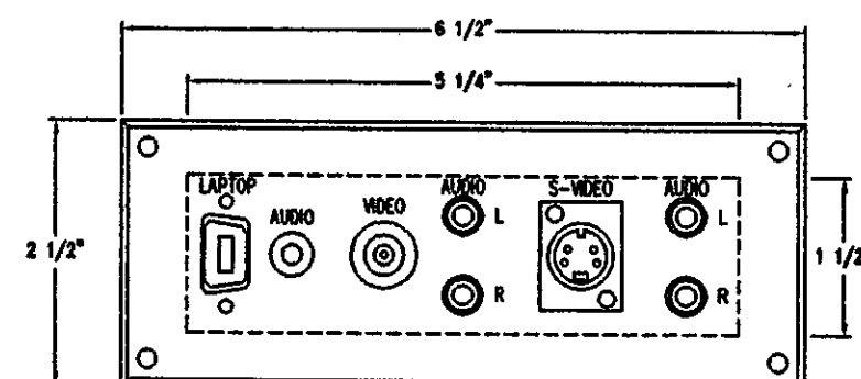
6 PODIUM GUEST PLATE DETAILS T3.3 SCALE: NTS PODIUM
