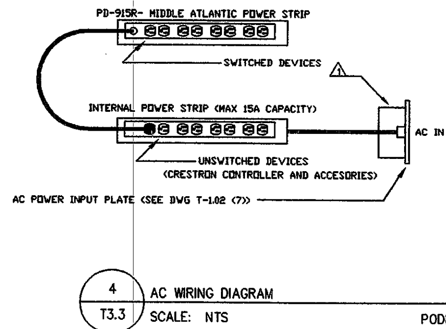
3 AC INPUT PLATE DETAILS T3.3 SCALE: NTS PODIUM
