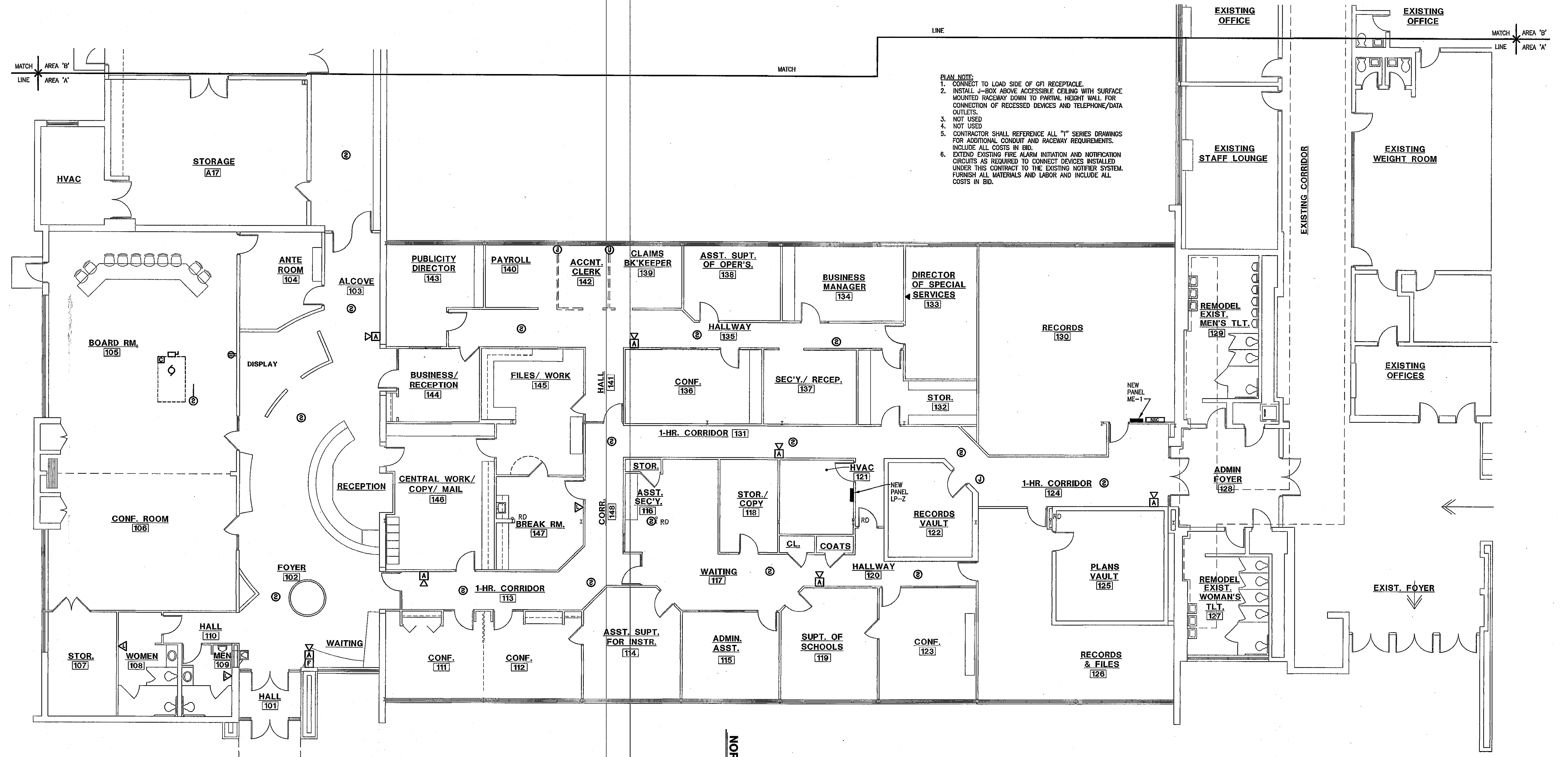
SYSTEMS PLAN - AREA 'A' 1/8"=1'-0"
