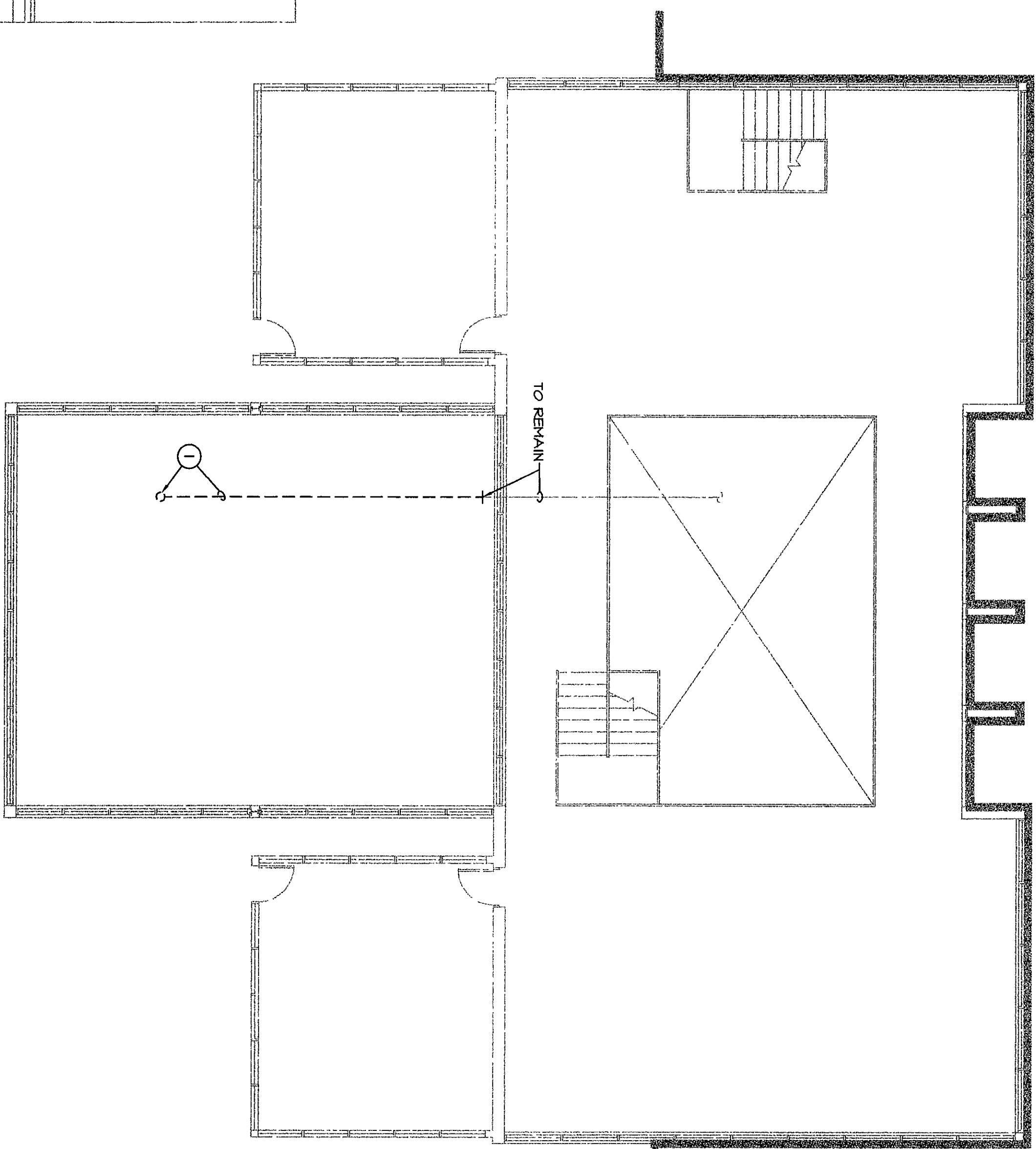
DEMOLITION PLAN - UNIT B (UPPER LEVEL) SCALE: 1/8" = 1'-0"
