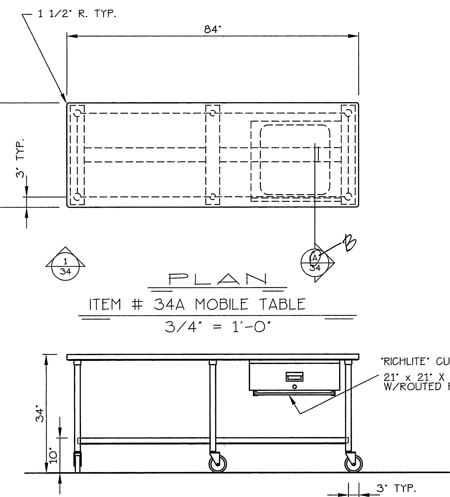
ELEVATION 3/4" = 1'-0"
