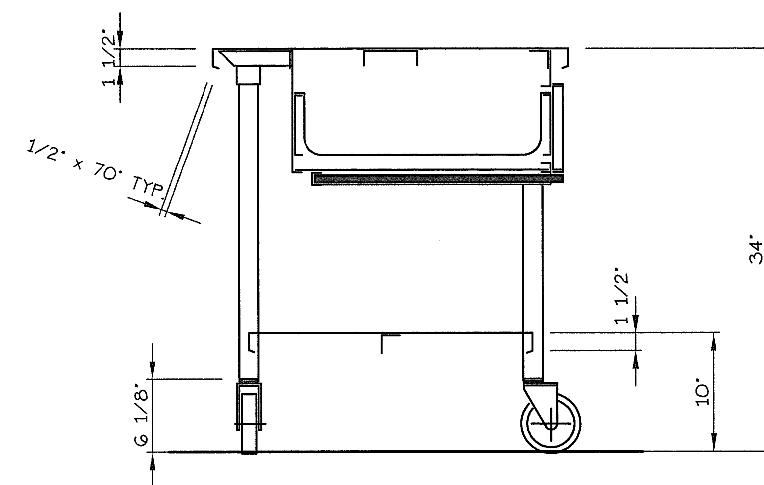
SECTION 1 1/2" = 1'-0"
