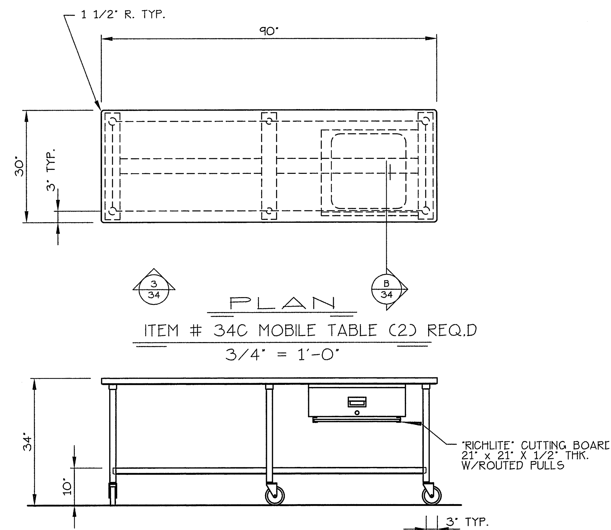
ELEVATION 3/4" = 1'-0"
