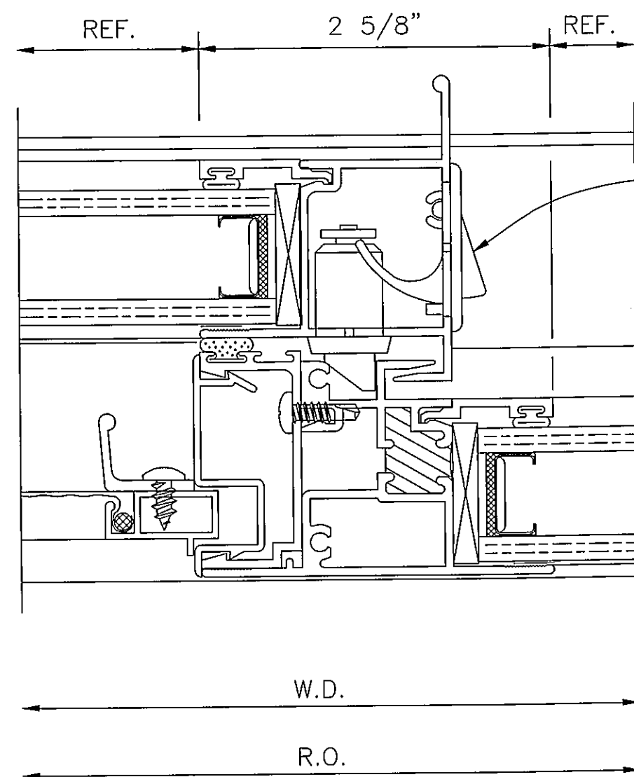
45 MEETING RAIL
