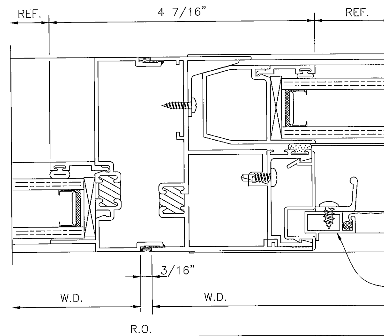
49 STACK
