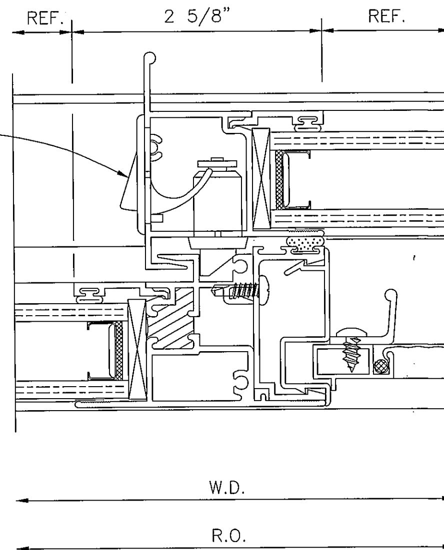
46 MEETING RAIL
