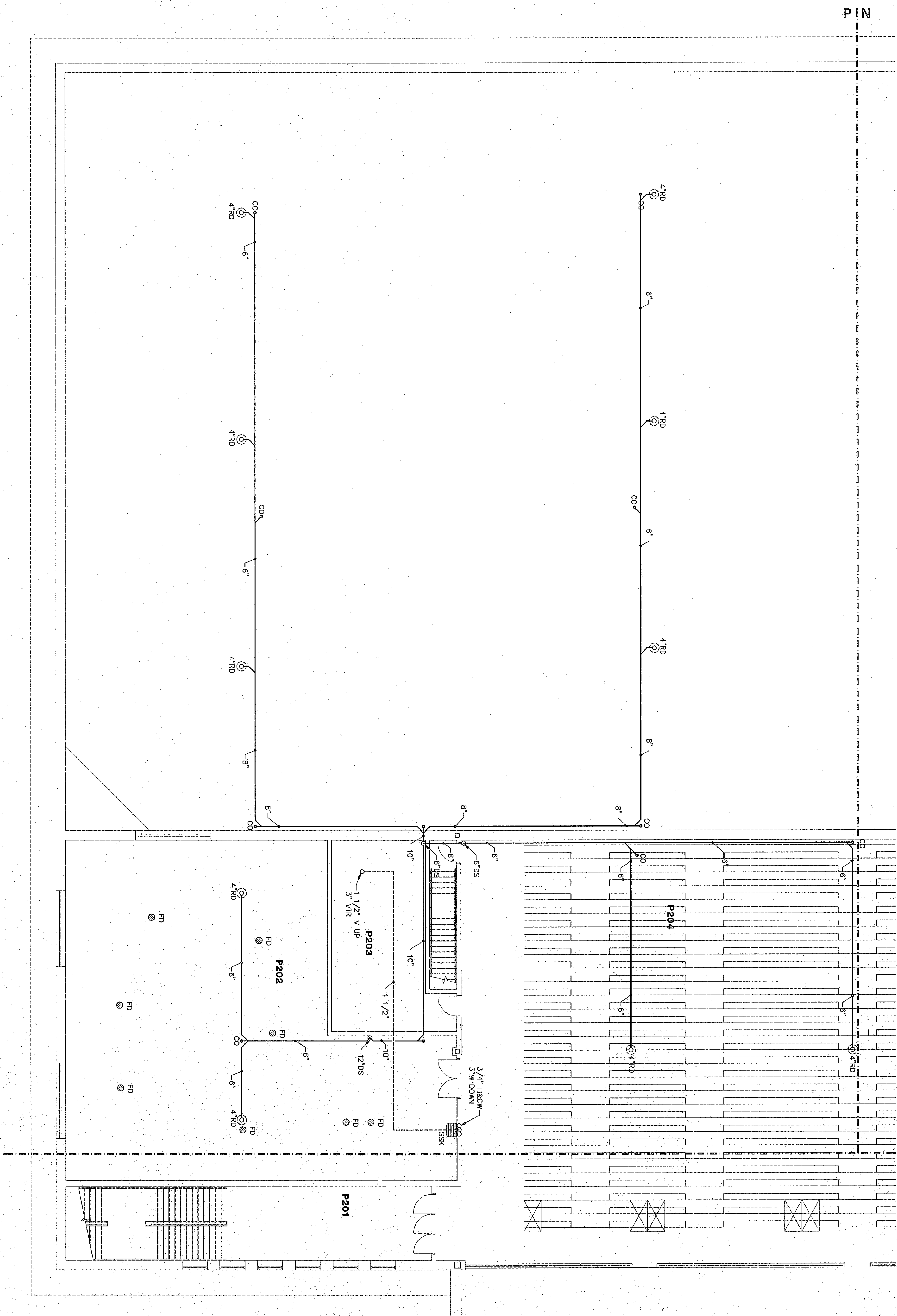
FLOOR PLAN UNIT "P2"
