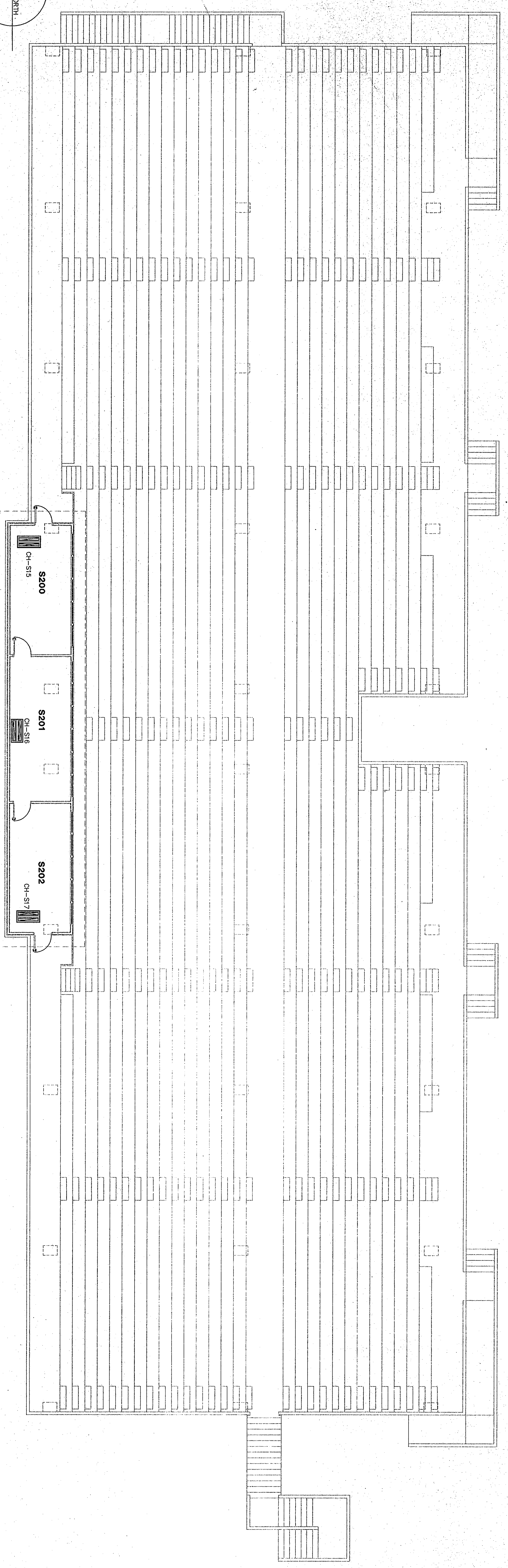
FLOOR PLAN UNIT "S2" (ALTERNATE REFER TO SPECIFICATIONS SECTION 01030) 1/8" = 1'-0"
