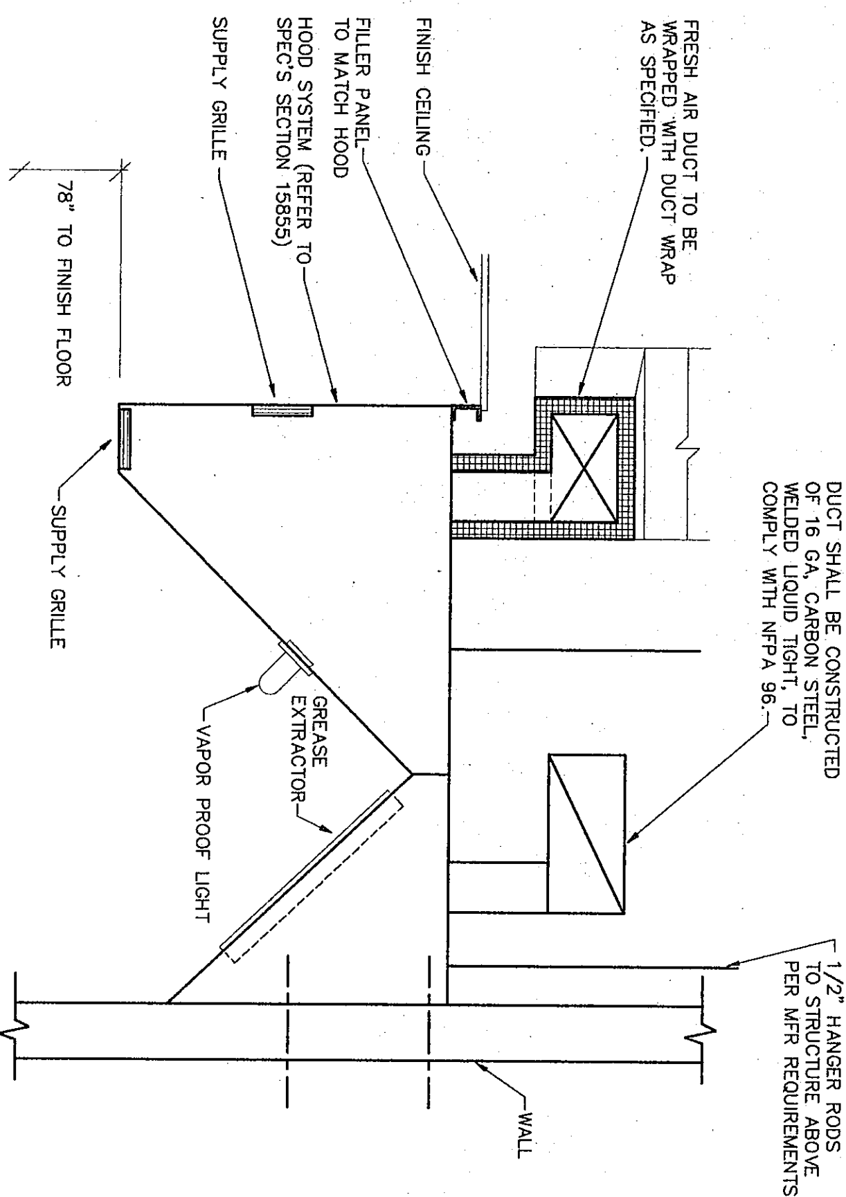
KITCHEN HOOD DETAIL NOT TO SCALE
