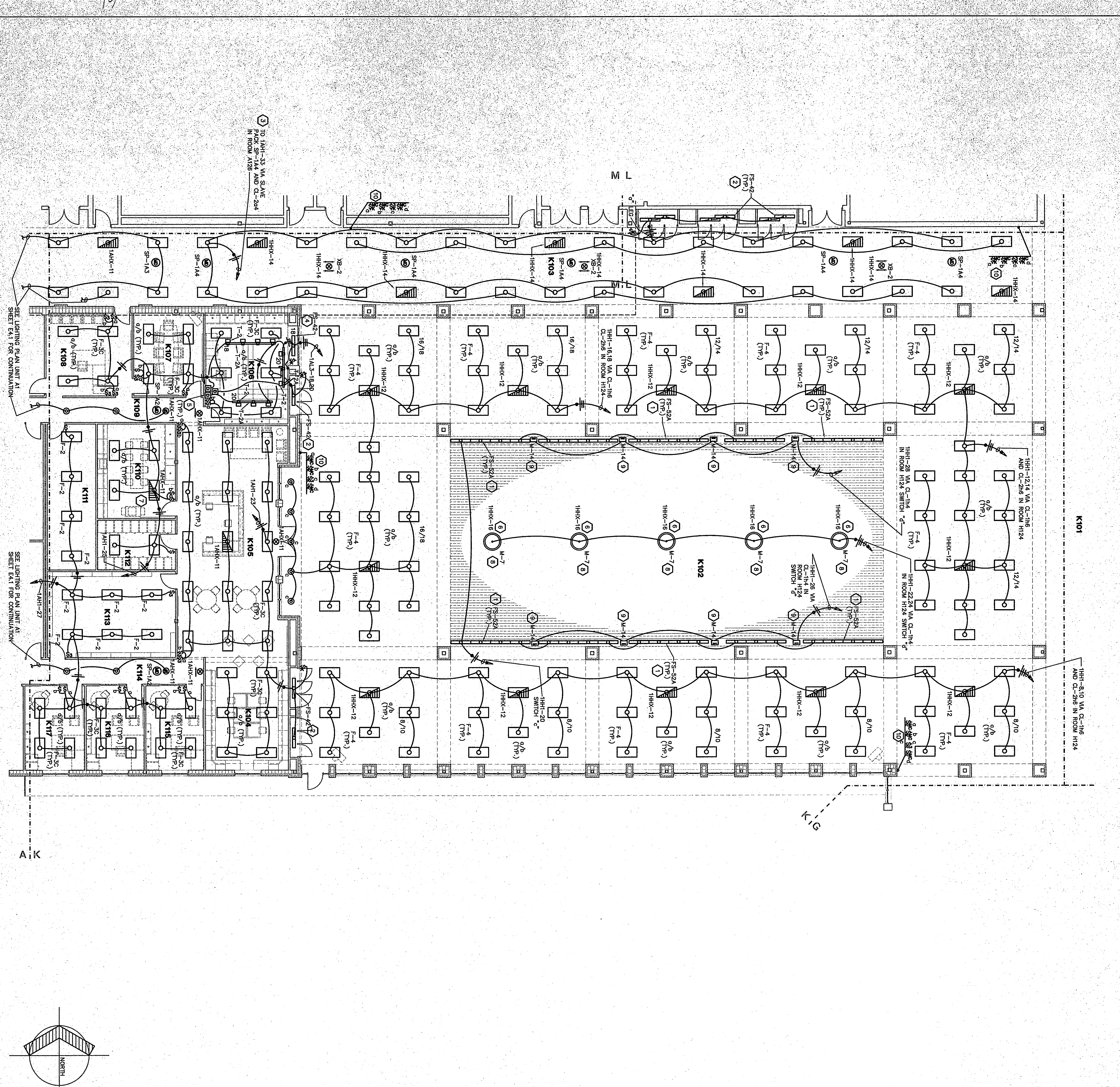
LIGHTING PLAN UNIT K
