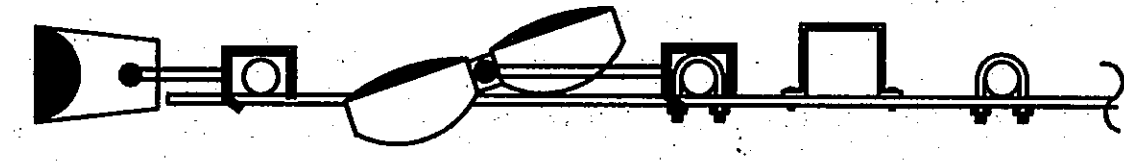
6 CYCLORAMA MOUNTING DETAIL NO SCALE
