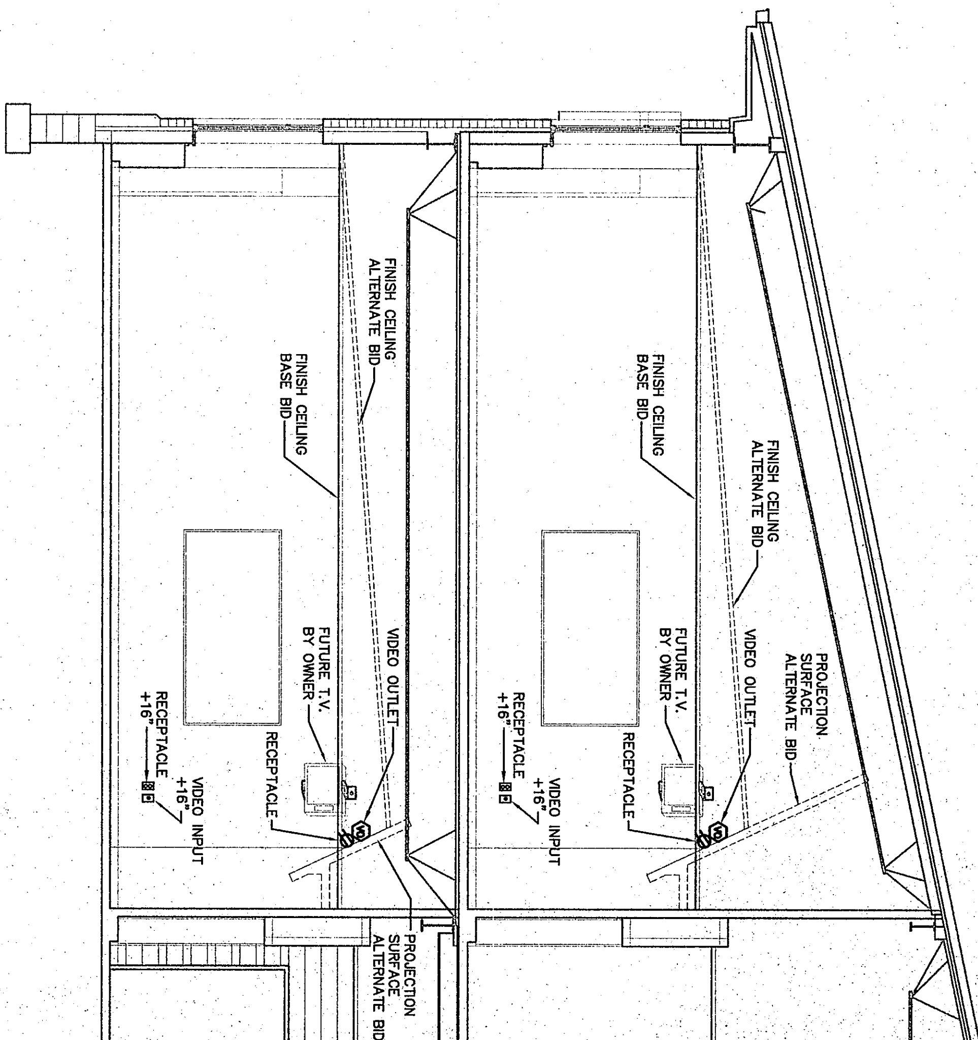
9 TYPICAL CLASSROOM SECTION NO SCALE
