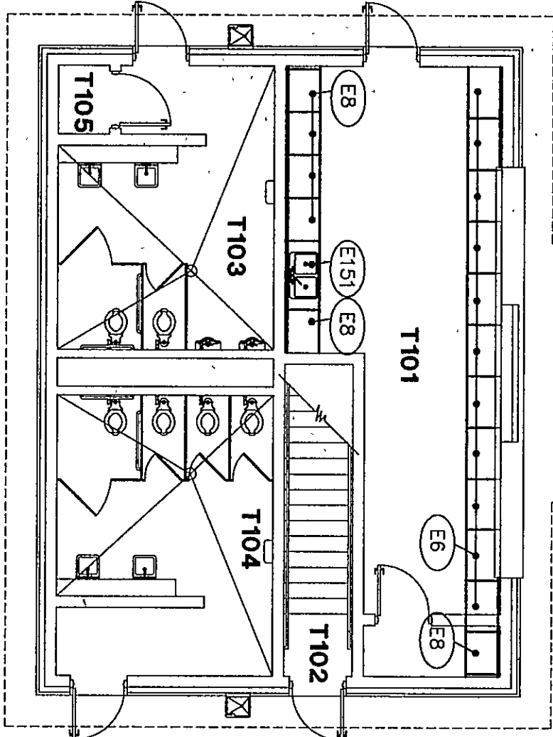
EQUIPMENT PLAN - BUILDING 'T'
