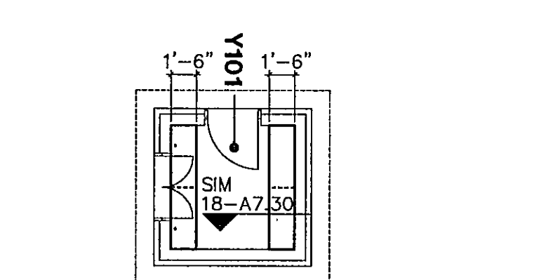
EQUIPMENT PLAN UNIT Y
