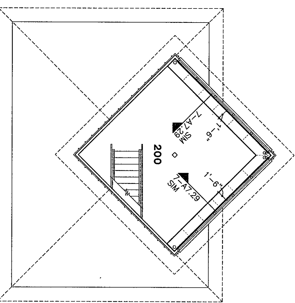
SECOND FLOOR EQUIPMENT PLAN - BUILDING 'T,U,V'
