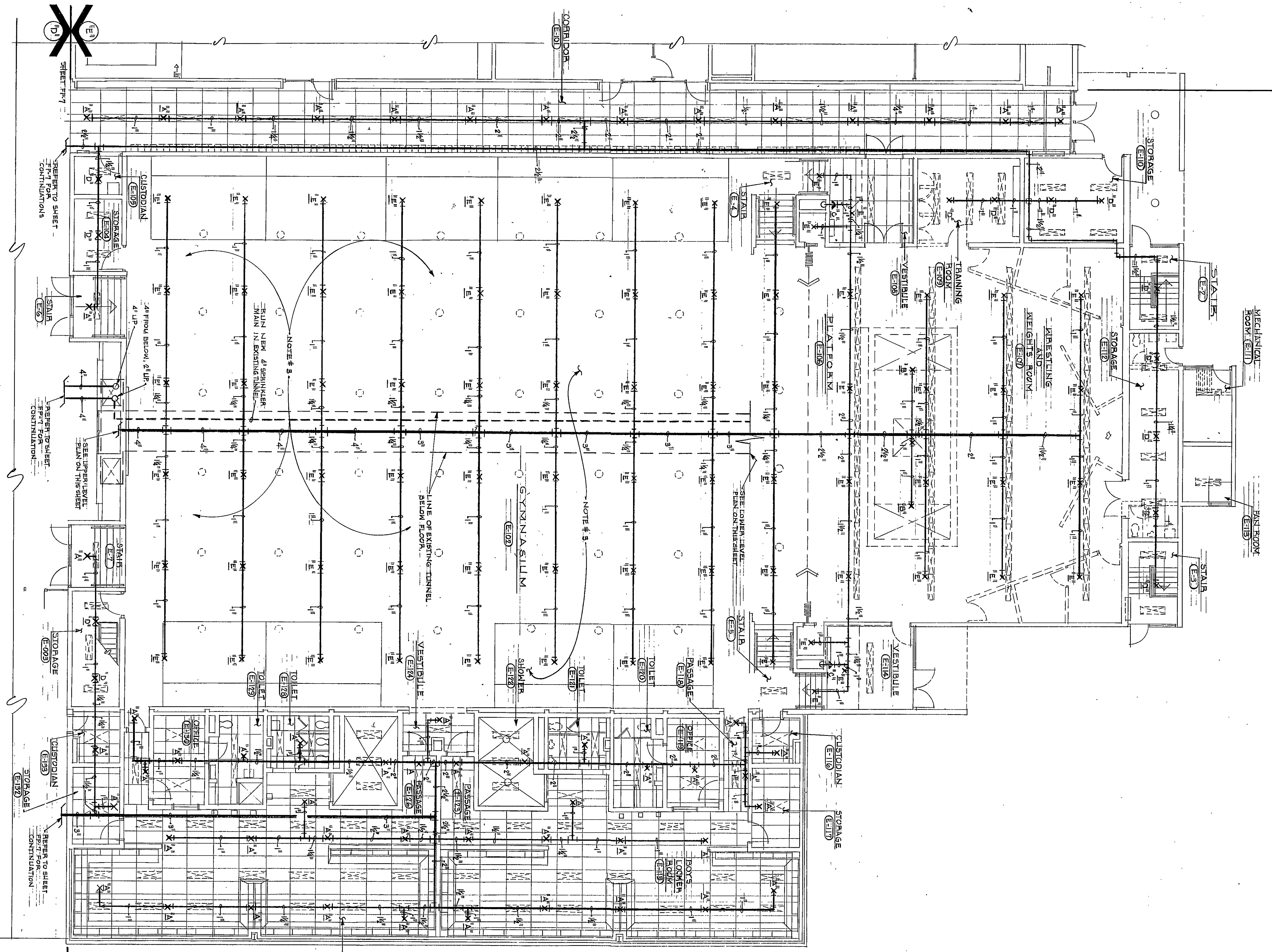
UNIT "E" SPRINKLER FLOOR PLAN SCALE 1/8" = 1'-0"
