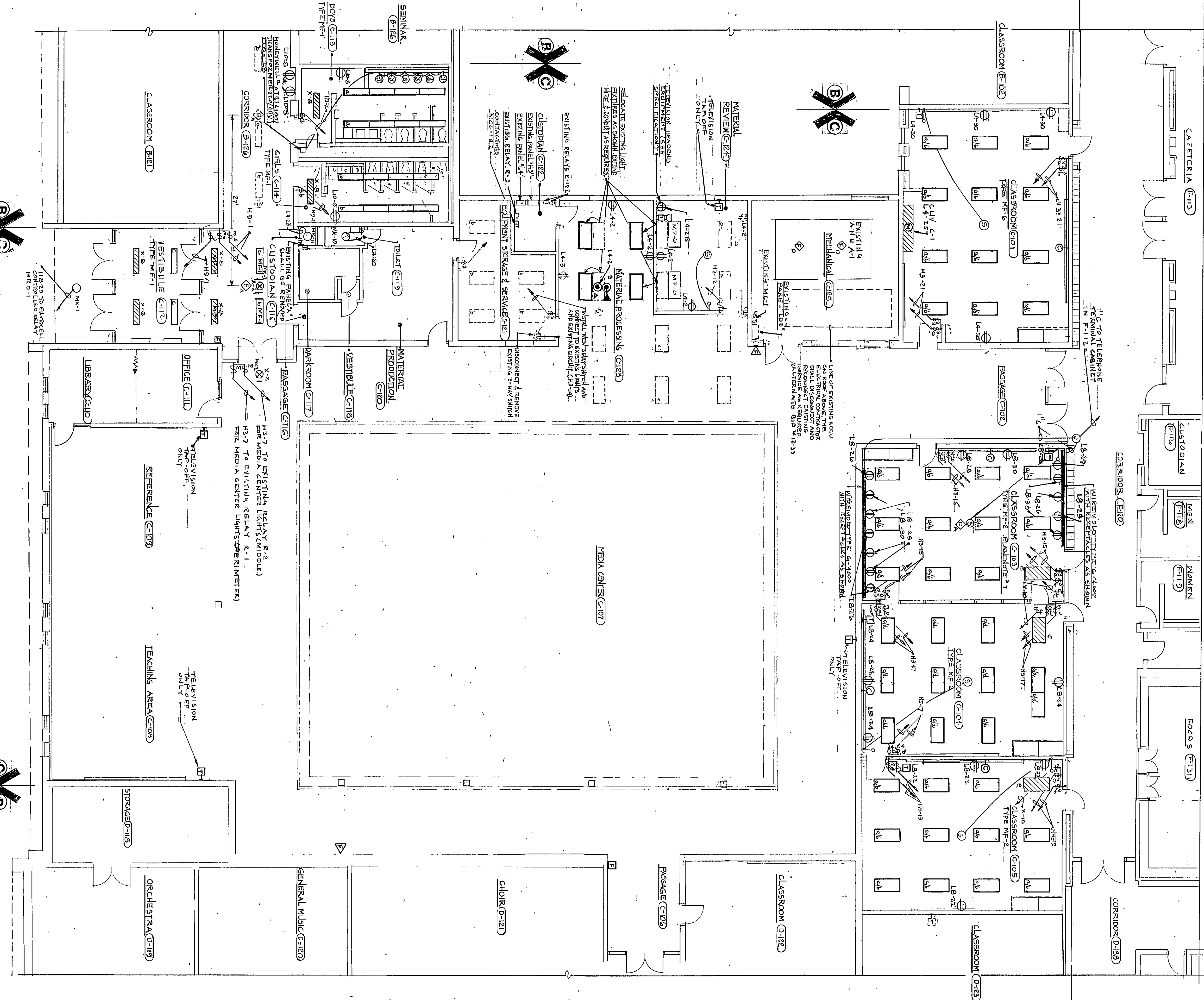
UNIT C ELECTRICAL FIRST FLOOR PLAN SCALE: 1/8" = 1'-0"
