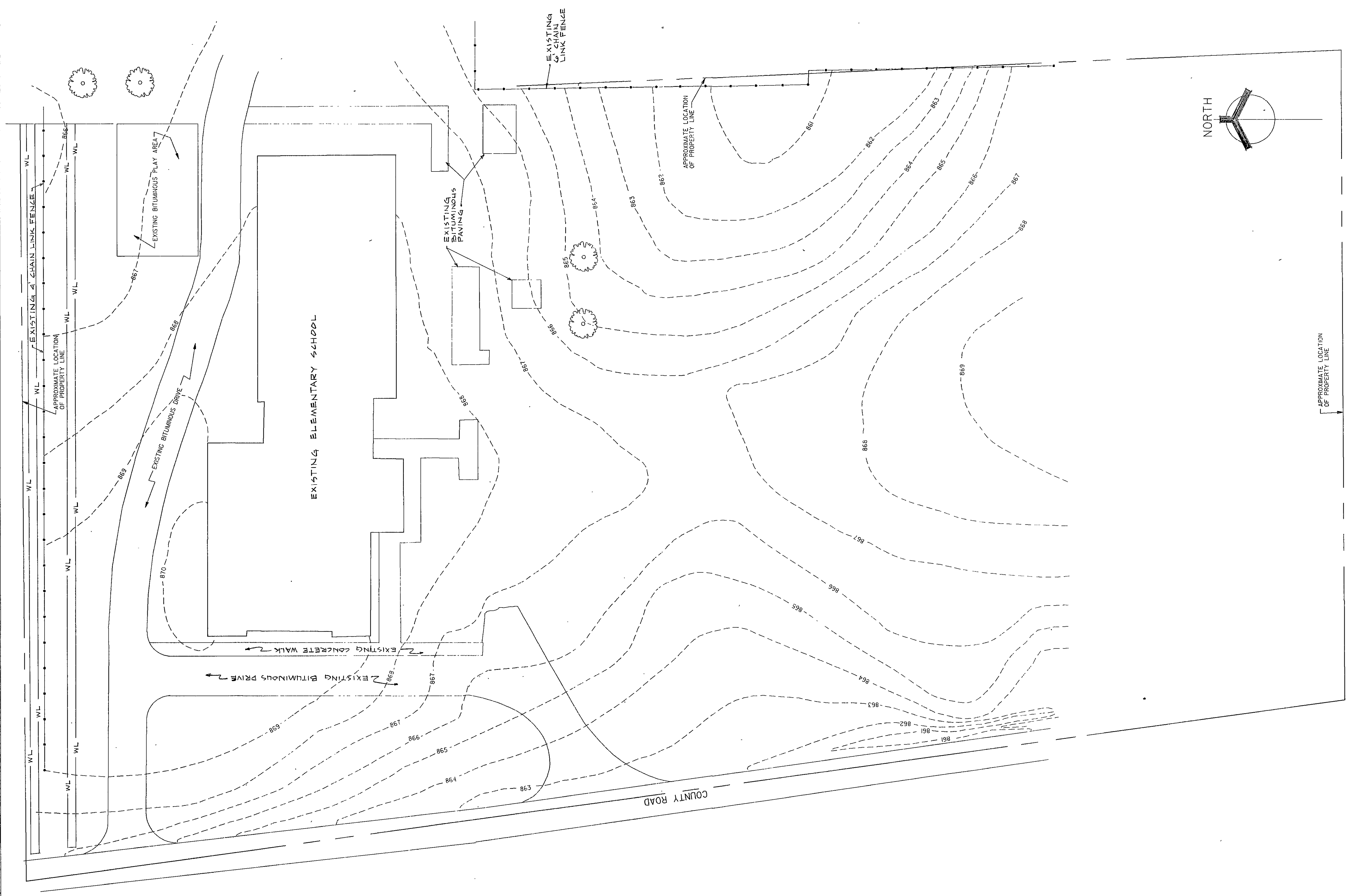
PARTIAL PLOT PLAN SCALE: 1" = 30' NOTE: SEE SHEET "S-1" FOR PLAN NOTES. SEE SHEET "S-2" FOR LEAND.
