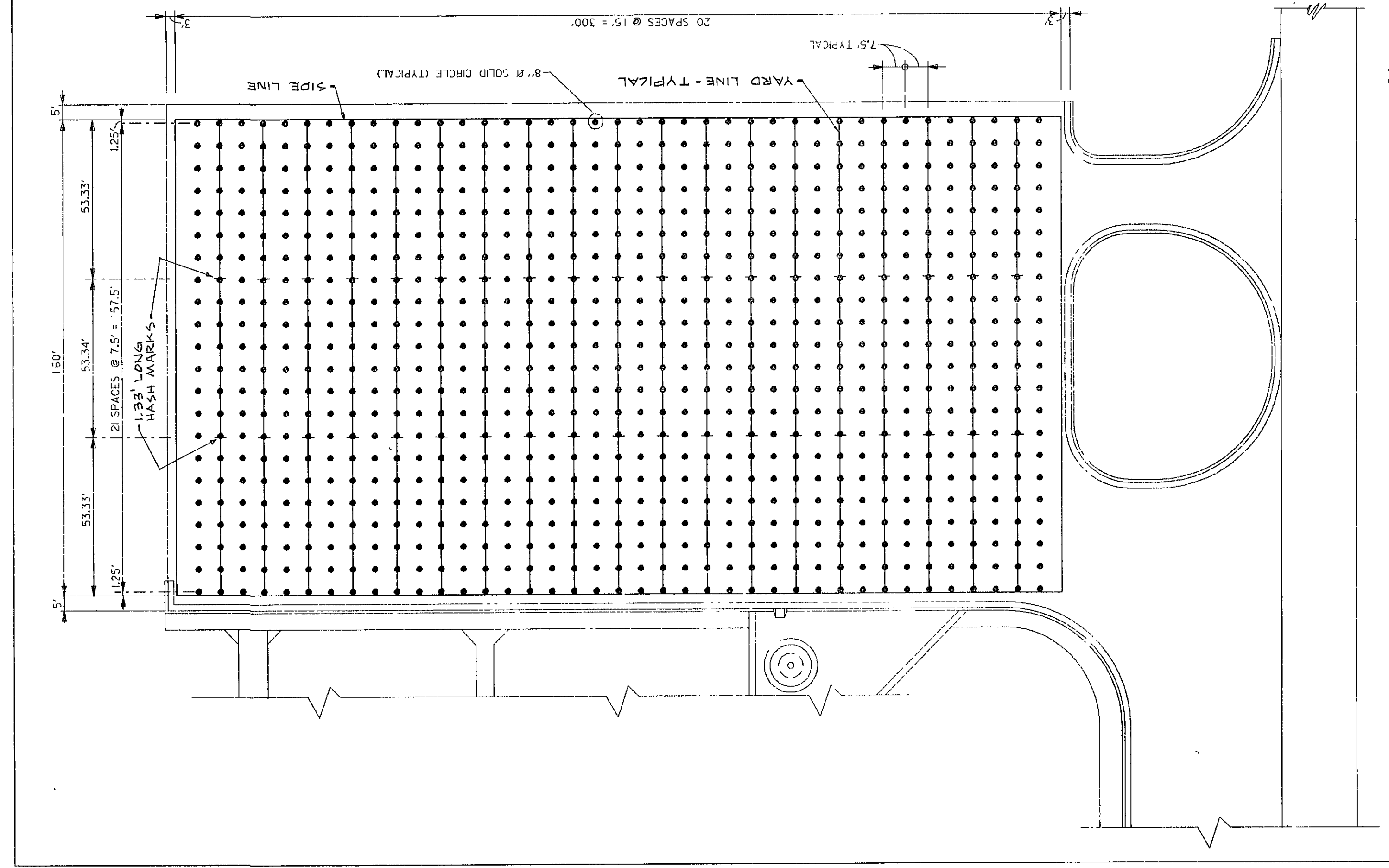
STRIPING PLAN SCALE: 1" = 30' NOTE: SEE SHEET "S-1" FOR PLAN NOTES. NOTE: SEE SHEET "S-2" FOR LEGEND.
