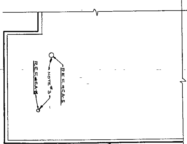
PARTIAL ROOF PLAN AREA #2 SCALE 1/8" = 1'-0"
