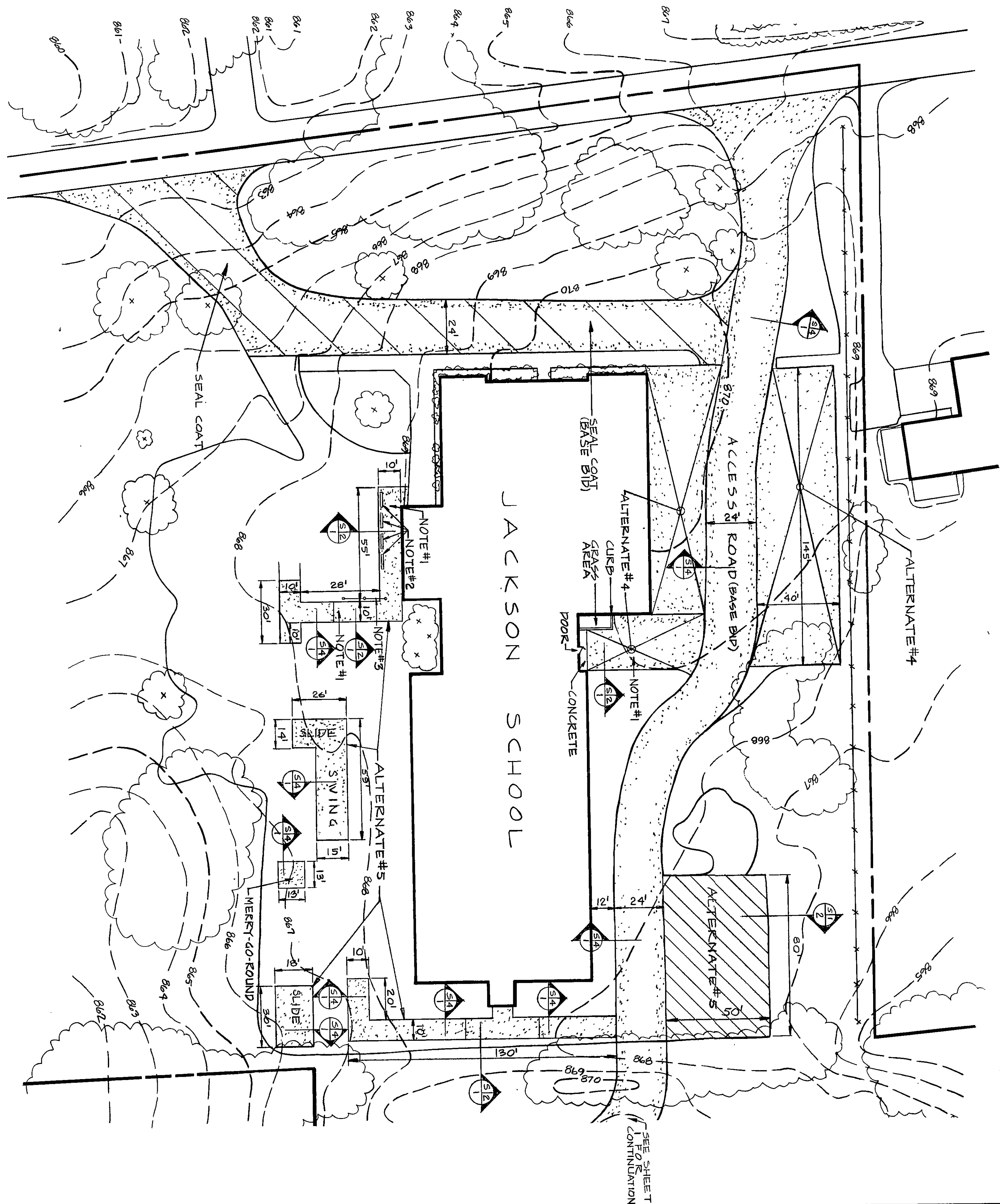
PLOT PLAN SCALE: 1"=30' JACKSON SCHOOL
