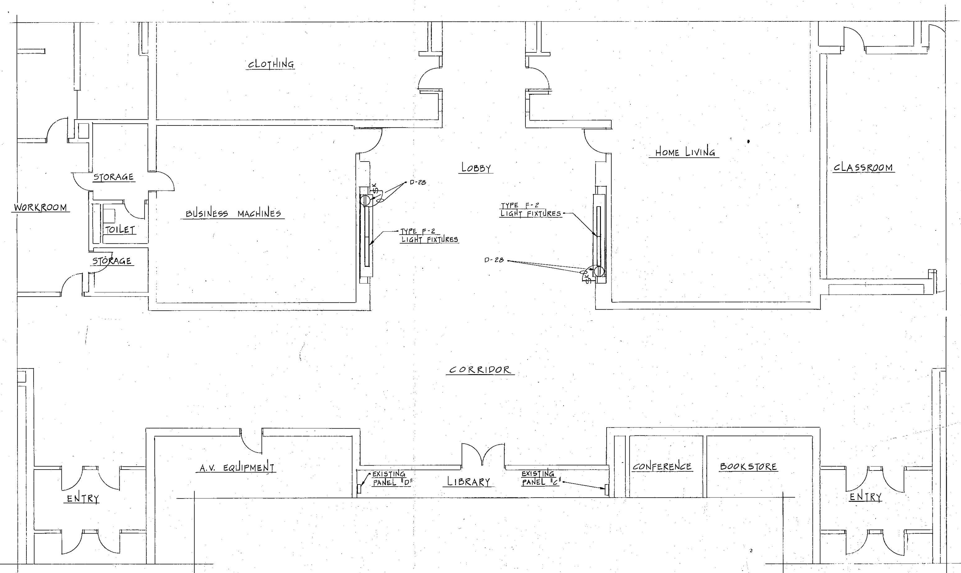
ELECTRICAL PLAN OF NEW DISPLAY CASES
