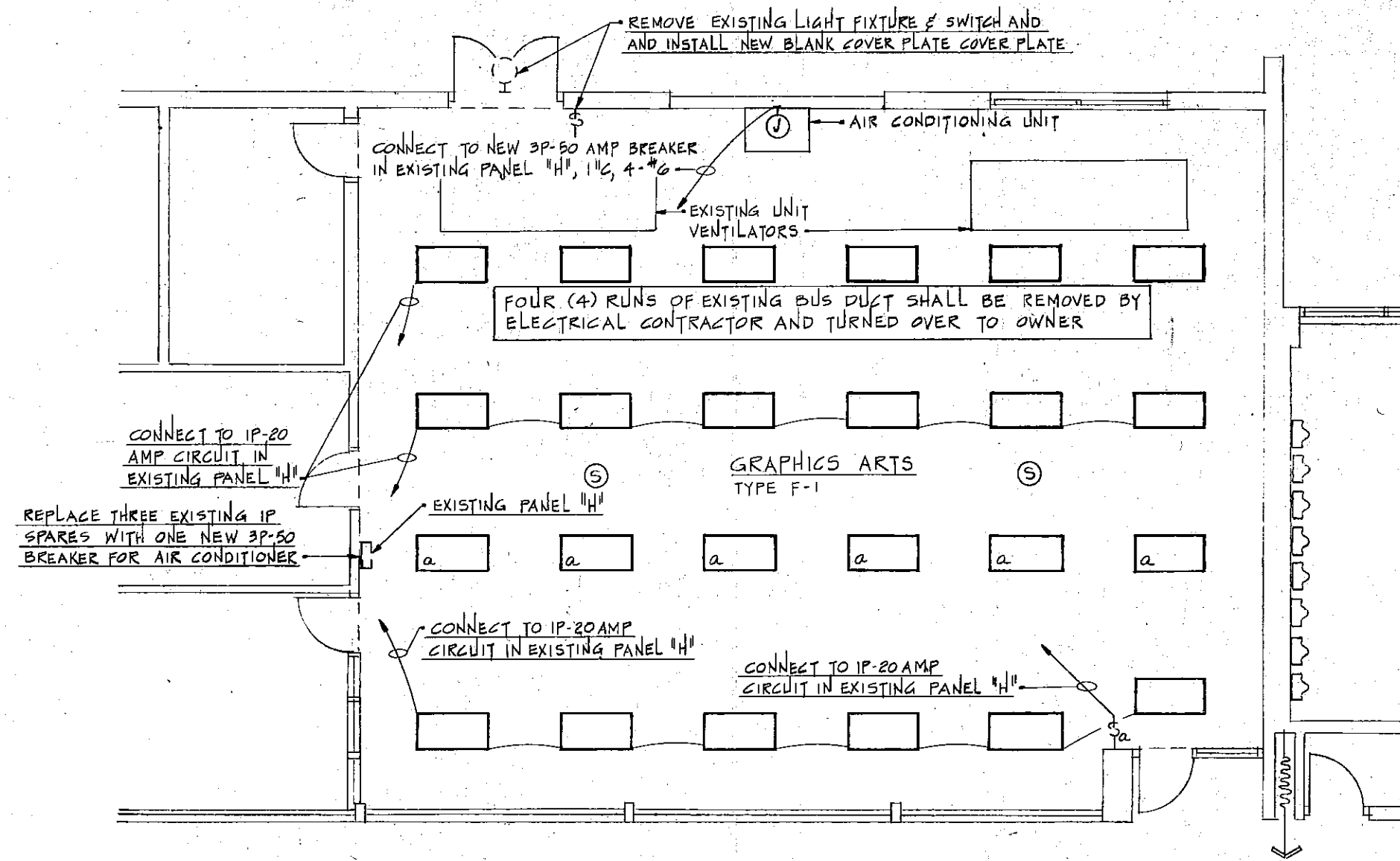
ELECTRICAL PLAN OF GRAPHIC ARTS ROOM
