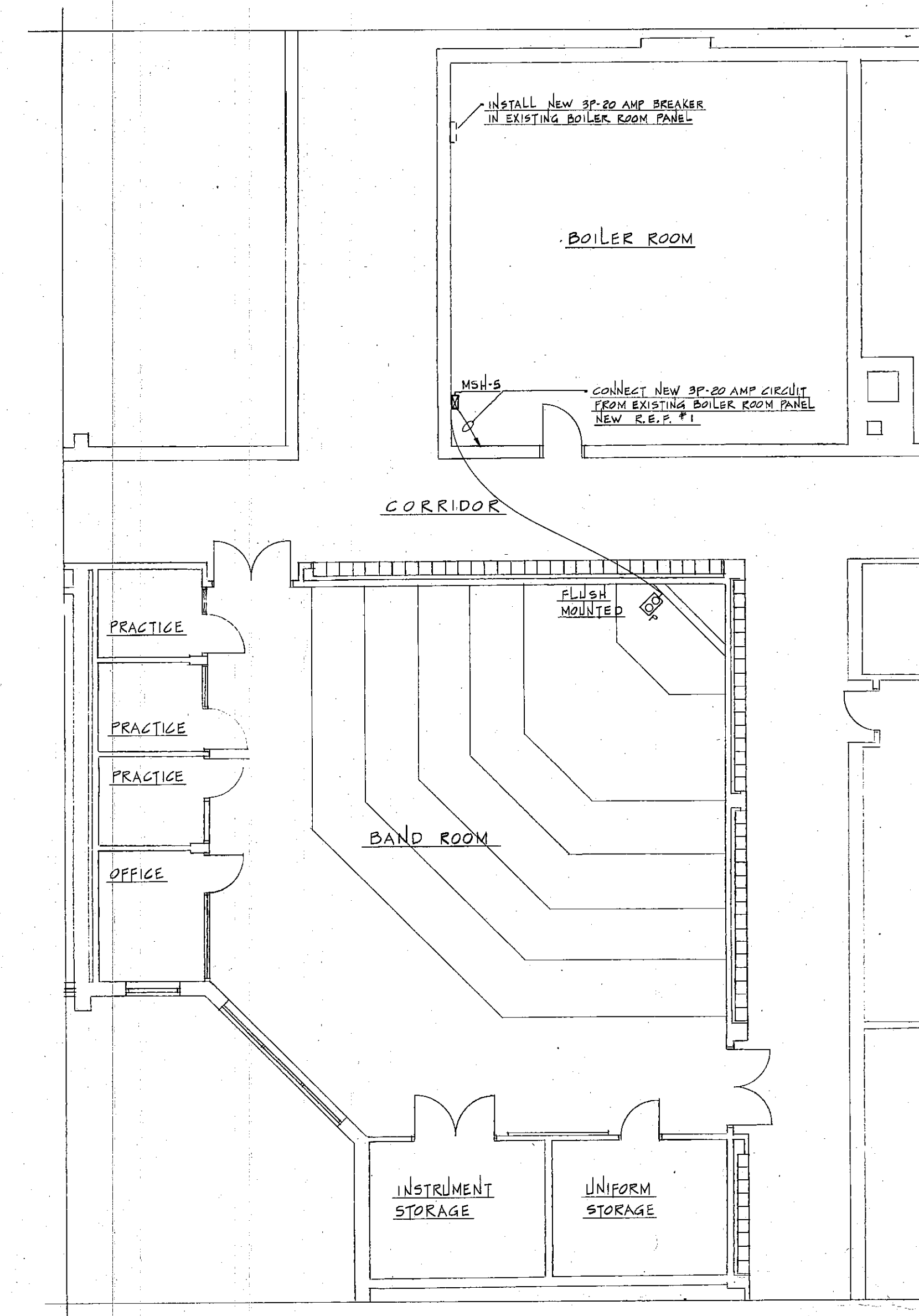
ELECTRICAL PLAN OF BAND ROOM
