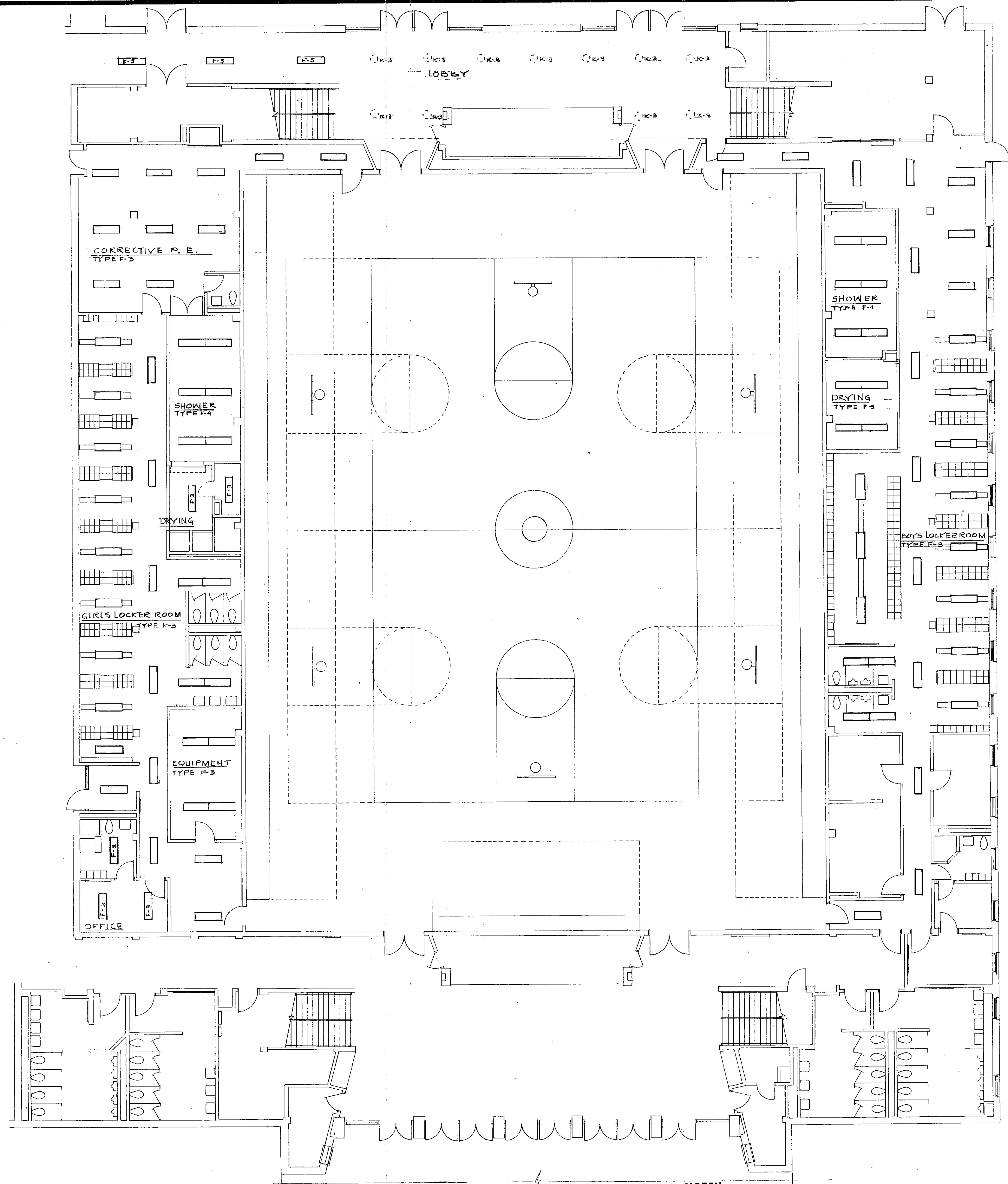
ELECTRICAL GYMNASIUM PLAN SCALE: 1/8"=1'-0"
