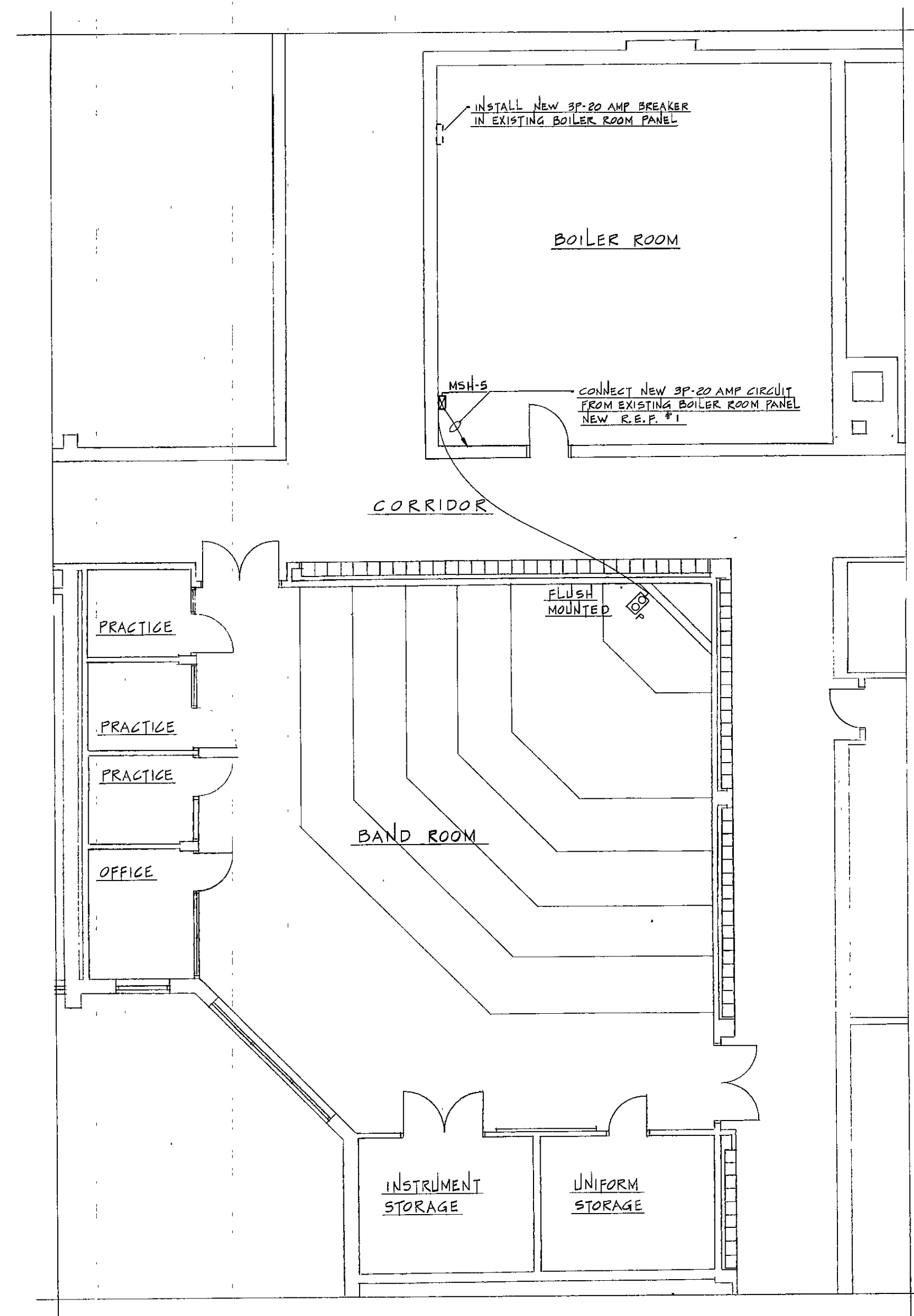
ELECTRICAL PLAN OF BAND ROOM SCALE: 1/8" = 1' - 0"
