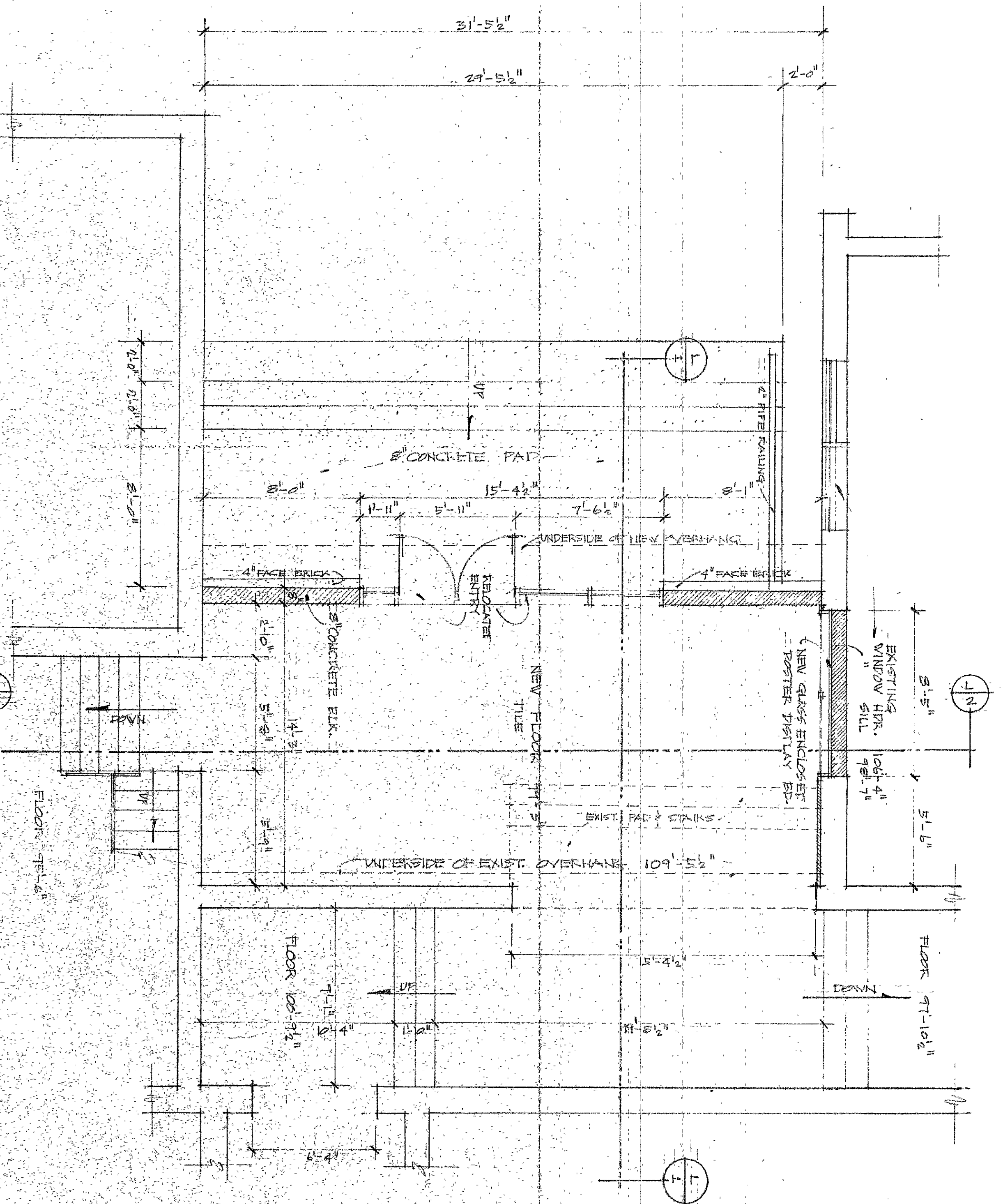
PLAN NEW SOUTH LOBBY SCALE: 1/4" = 1'-0"
