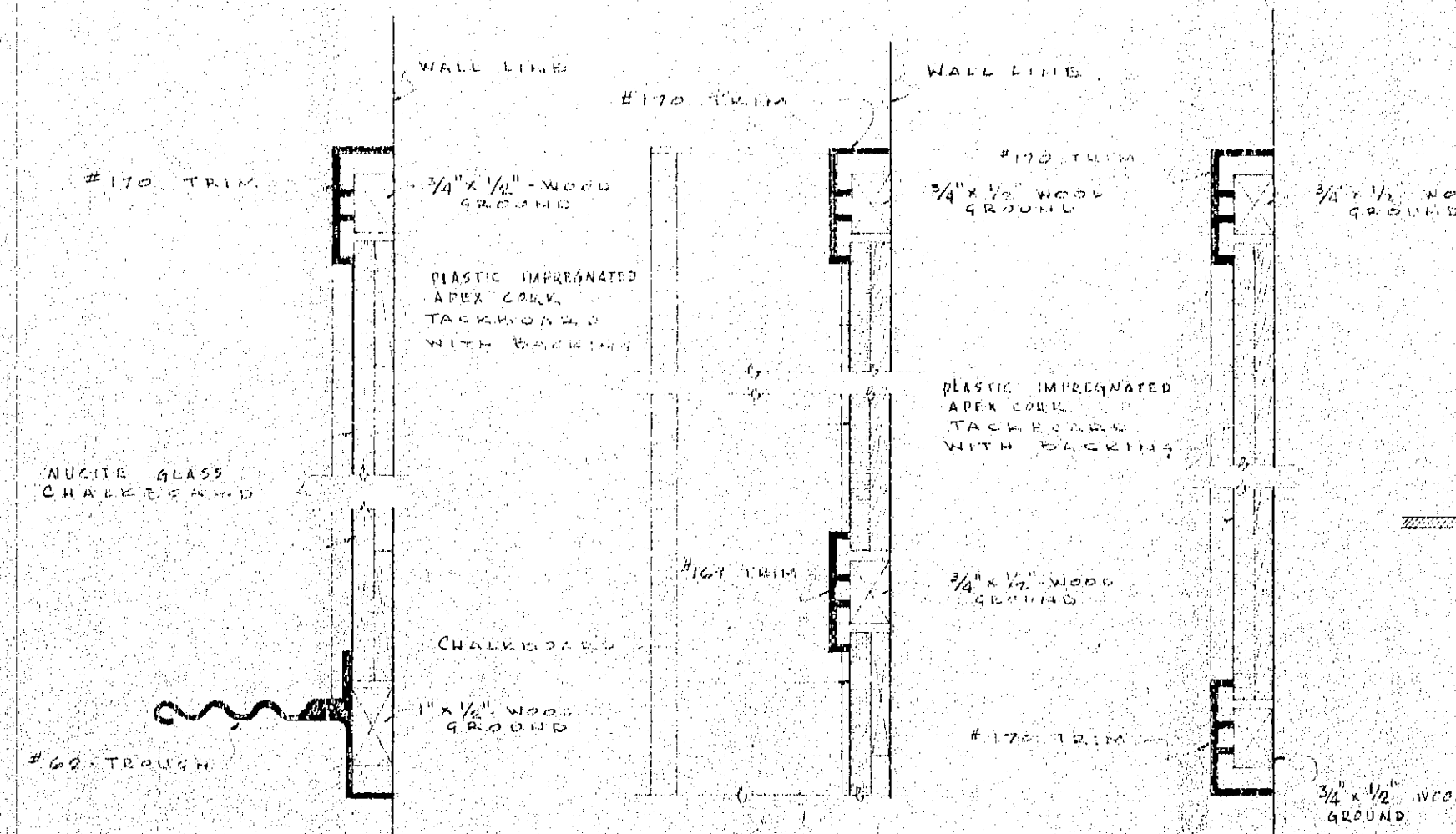
CHALKBOARD & TACKBOARD DETAILS SCALE - HALF SIZE ALUM. TRIM BY CLAUDE
