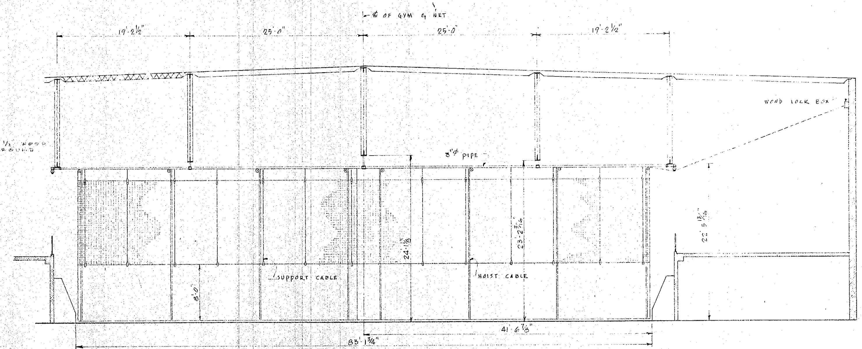
DETAIL OF DIVIDING CURTAIN SCALE 1/4\"/>
