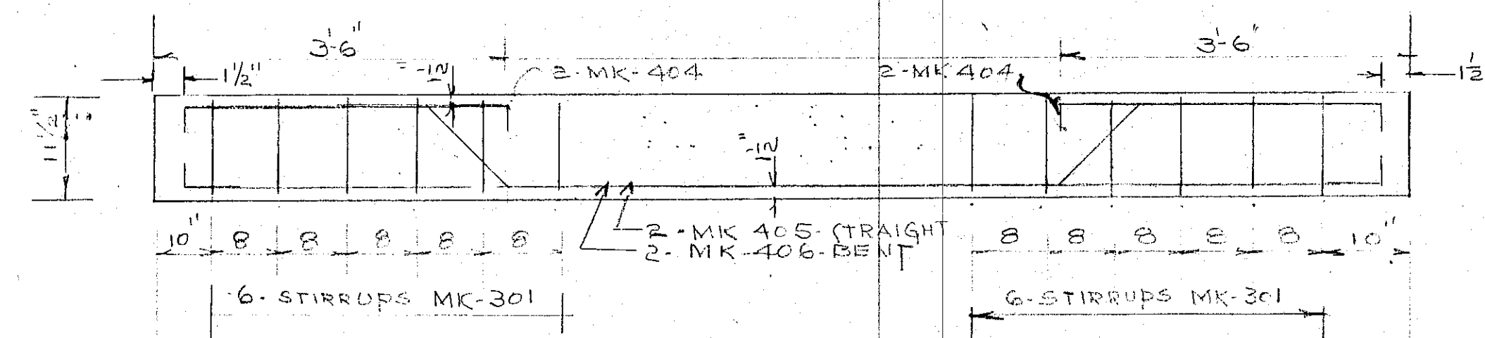
LINTEL (CL-2) (8 REQUIRED)
