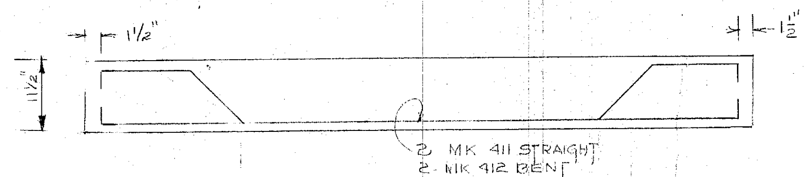
LINTEL (CL-5) (ONE REQUIRED)
