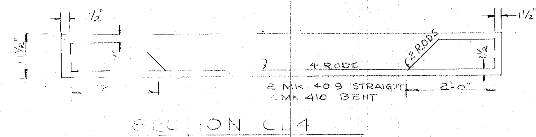
LINTEL (CL-4) (2 REQUIRED)
