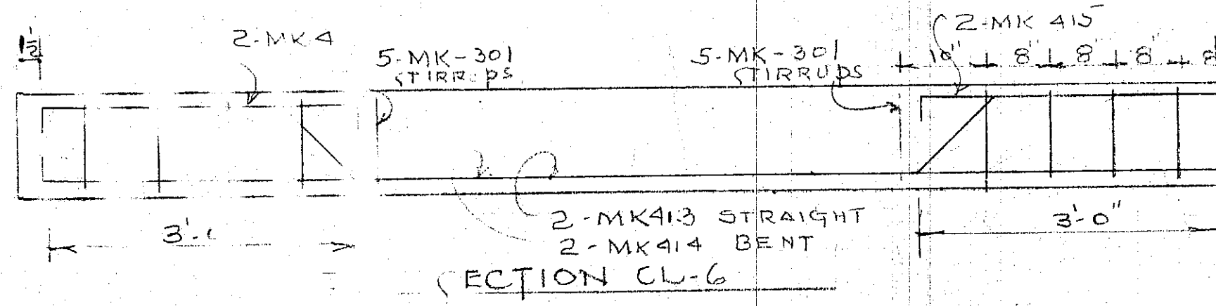
LINTEL (CL-6) (ONE REQUIRED)
