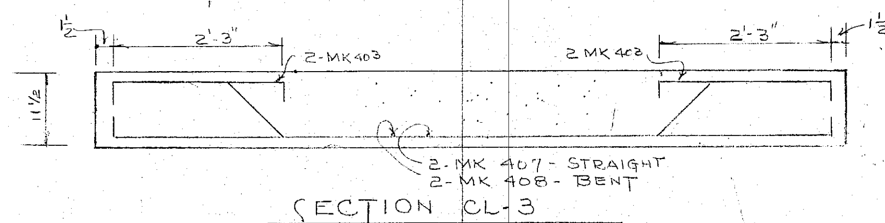
LINTEL (CL-3) (1-REQUIRED)
