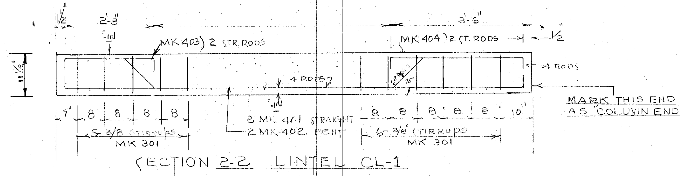
LINTEL (CL-1) (15-REQUIRED)
