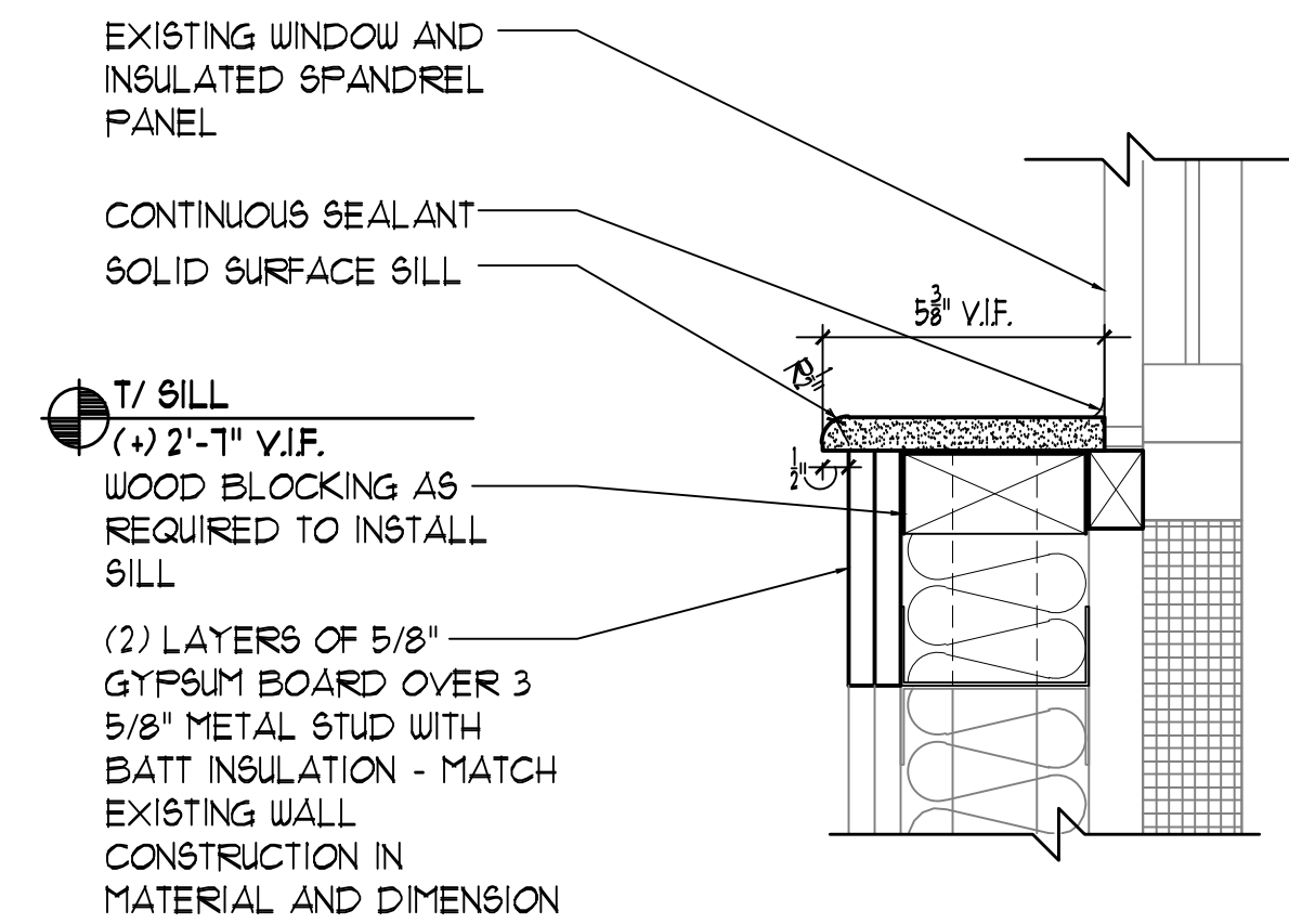
7 DETAIL 3" x 1'-0"
