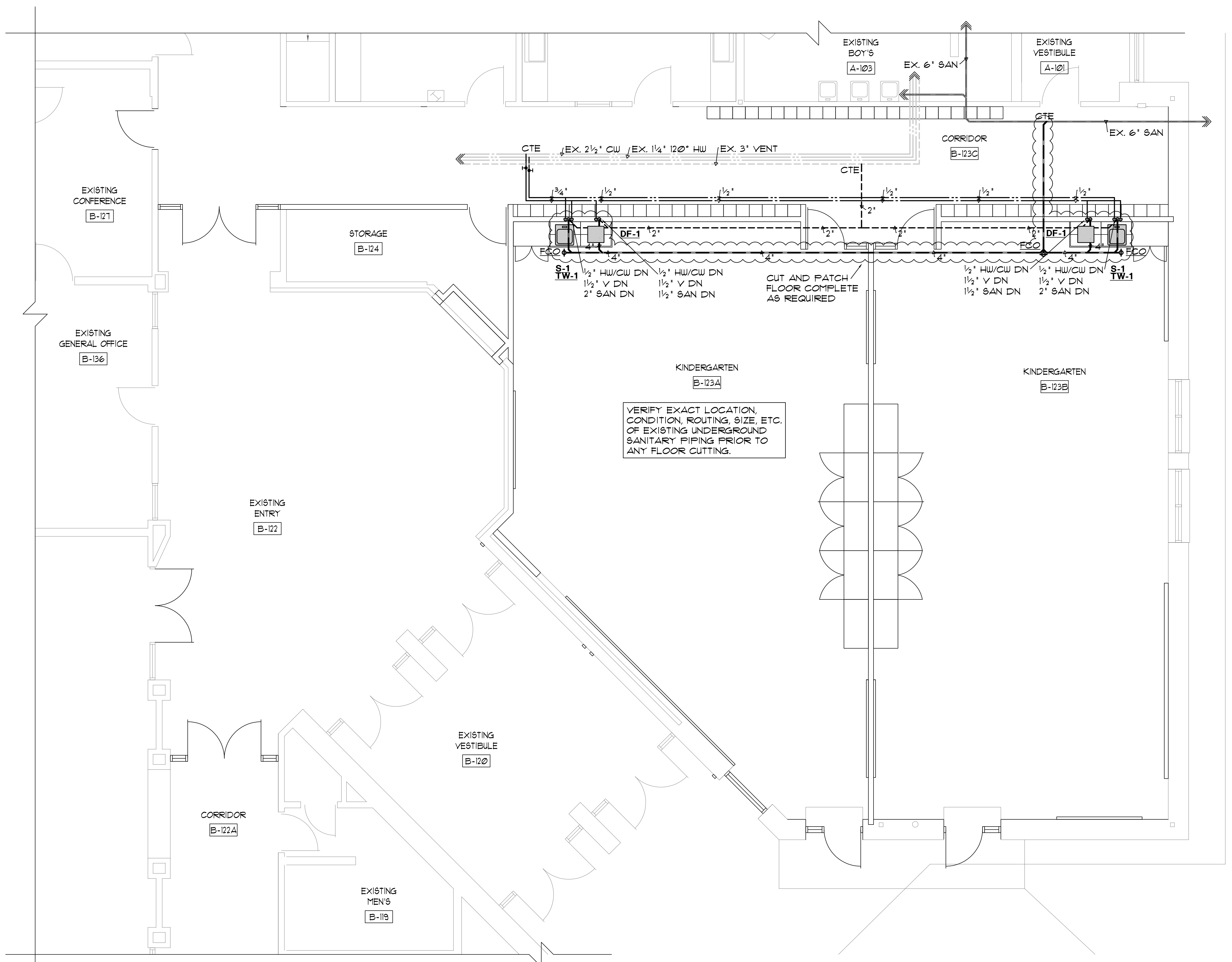
1 PLUMBING FLOOR PLAN 1/4" = 1'-0"
